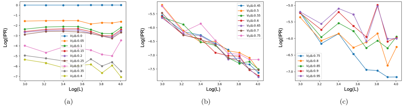
FIG. 17. IPR of the states that is in the middle of the spectrum. The x axis is \text{Log}(L) and the y axis is \text{Log}(\text{IPR}) for (a) small V_0 , (b) intermediate V_0 , and (c) large V_0 .
