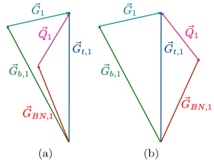
FIG. 1. (a) Case 1, \theta_{\text{BN}} > 0 and \theta_G > 0 . (b) Case 2, \theta_{\text{BN}} < 0 and \theta_G > 0 . The angles are exaggerated for illustration purpose.
