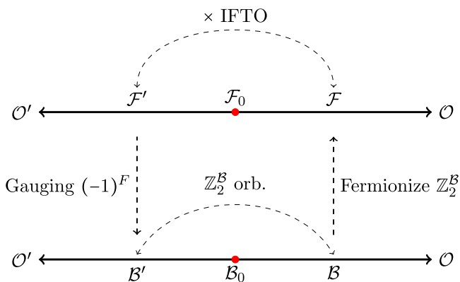
FIG. 7. The topological transition on the fermionic conformal manifold can be equivalently bosonized to a family of bosonic CFTs that are related by the \mathbb{Z}_2^{\mathcal{B}} orbifold.
