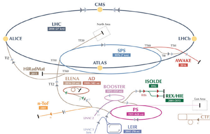
Figure 1-11: The schematic overview of the CERN accelerator complex with the accelerators labeled is shown above. Proton and lead ions are accelerated using these facilities and boost their energies to the TeV scale.
