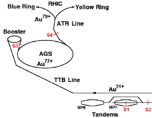
Figure 1-9: The acceleration of gold ions for RHIC is shown above.
