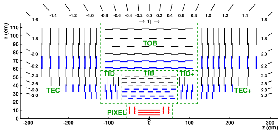
Figure 3-9: The schematic view of the CMS tracking system is shown above.
