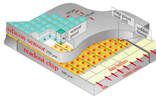
Figure 4-2: The schematic plot of a CMS silicon chip with pixel sensors is shown above.
