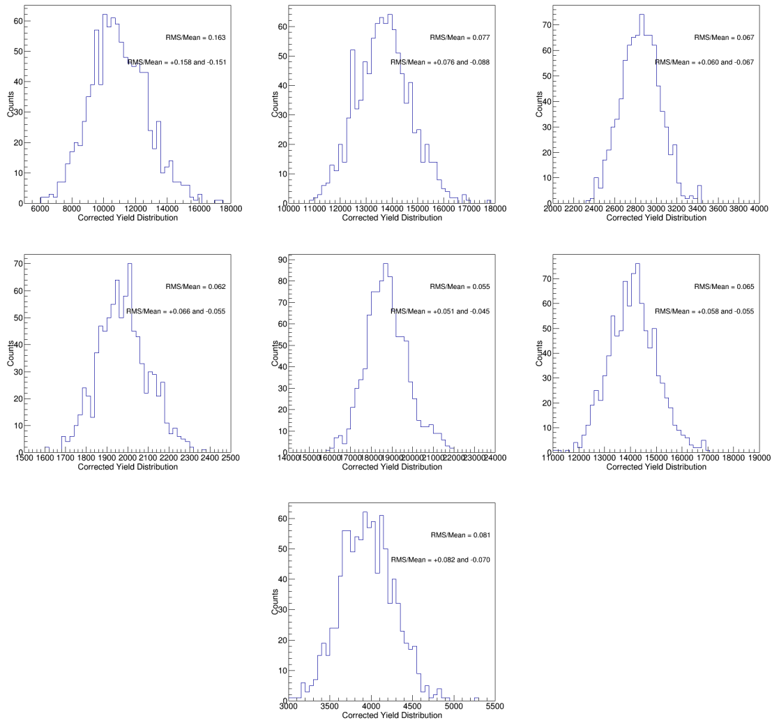
Figure 5-61: The B^+ corrected yield distributions of the 1000 data-like randomly resampled datasets for centrality in 0 - 90% in the p_T range of 7 - 10, 10 - 15, 15 - 20, and 20 - 50 GeV/c as well as 0 - 90%, 0 - 30%, and 30 - 90% in the p_T range of 10 - 50 GeV/c are shown above.
