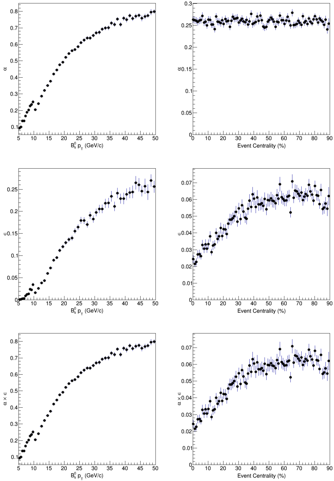
Figure 5-46: The B^+ acceptance (top), selection efficiency (middle), and efficiency (bottom) as a function of p_T (left) and event centrality (right) are shown respectively above. We should note that there is no significant centrality dependence on the B^+ acceptance, which makes sense.
