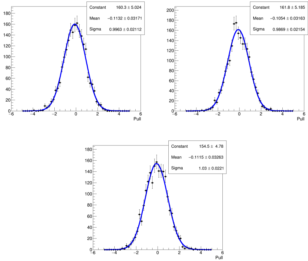
Figure 5-56: The B^+ pull distributions and the Gaussian fits for 0 - 30%, 30 - 90%, and 0 - 90% event centrality are shown respectively above.
