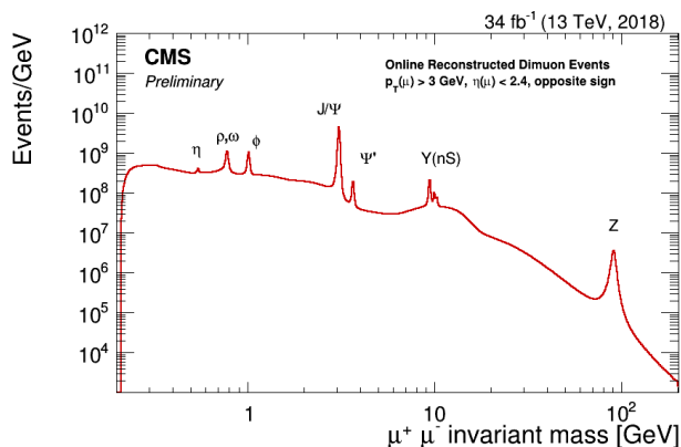
Figure 3-8: The dimuon invariant spectrum m_{\mu\mu} reconstructed by CMS HLT trigger in the 2018 pp dataset is shown above. We can identify the neutral vector boson resonances shown above.
