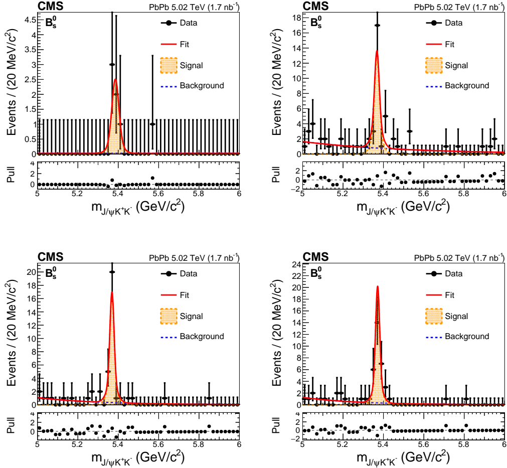
Figure 5-33: The B_s^0 invariant mass distributions as well as the fits to extract the signal raw yield N_S in different p_T bins are shown above.
