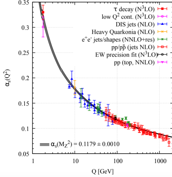
Figure 1-2: The running of the strong coupling constant \alpha_s in different experiments at different energy scales Q and the comparison with QCD calculations are shown above. Image from: [4]
