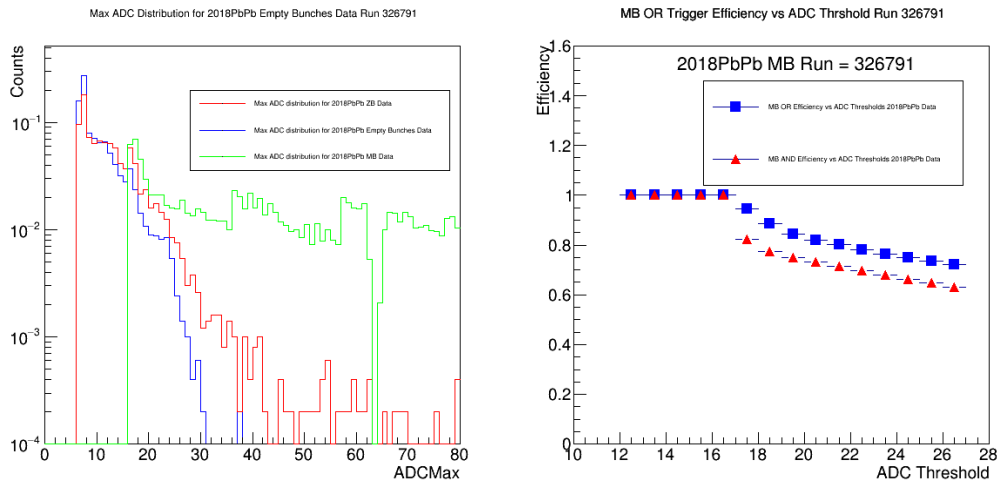
Figure 3-5: In the CMS 2018 PbPb Run 326791, the ZB data (red), Empty Bunches (blue), and MB data (green) maximum ADC distributions (left) and the efficiencies of MB OR (blue) and MB AND (red) as a function ADC threshold (right) are shown above.
