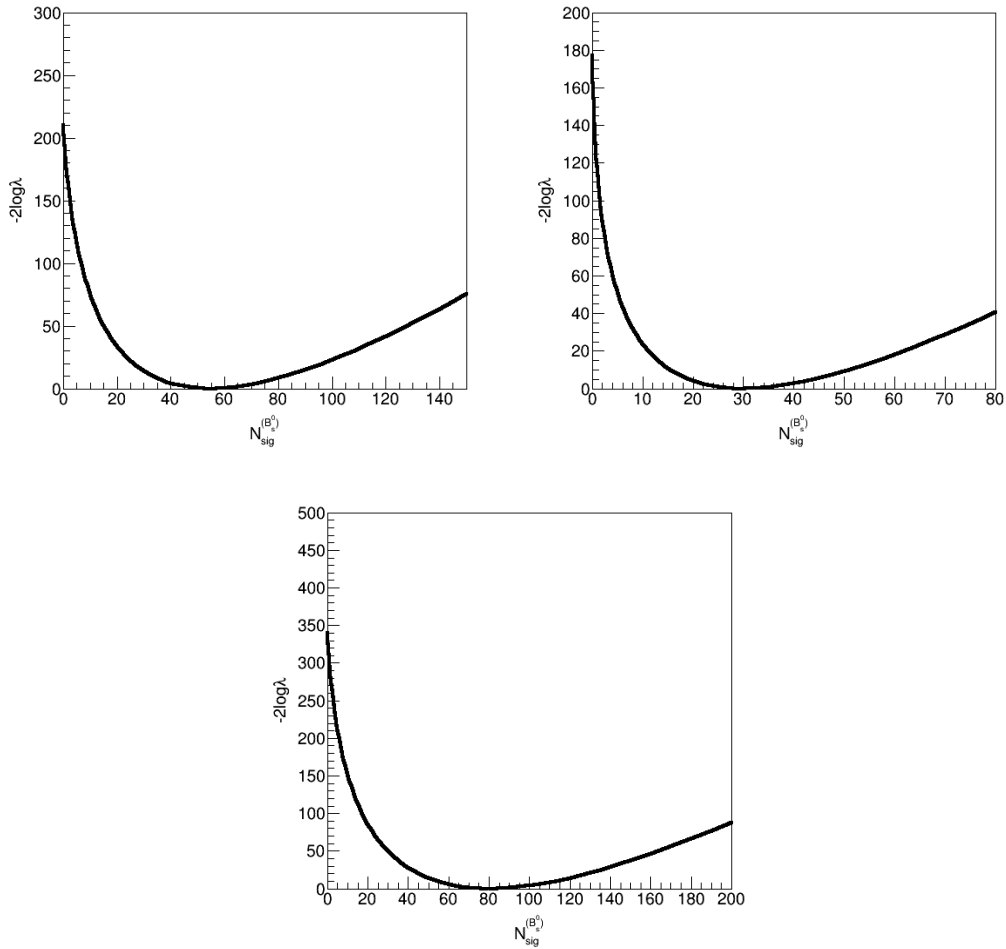
Figure 5-38: The significance vs signal yield for centrality bins in 0 - 30%, 30% - 90% 0 - 90% for p_T in 10 - 50 GeV/c are shown above
