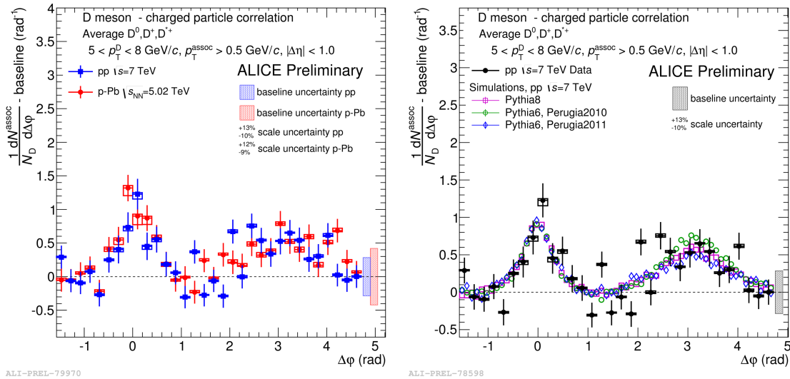
Figure 2-13: The ALICE D-hadron angular correlated in both pp (blue) and pPb (red) collision (left) and the comparison of pp data with PYTHIA calculations (right) are shown above.
