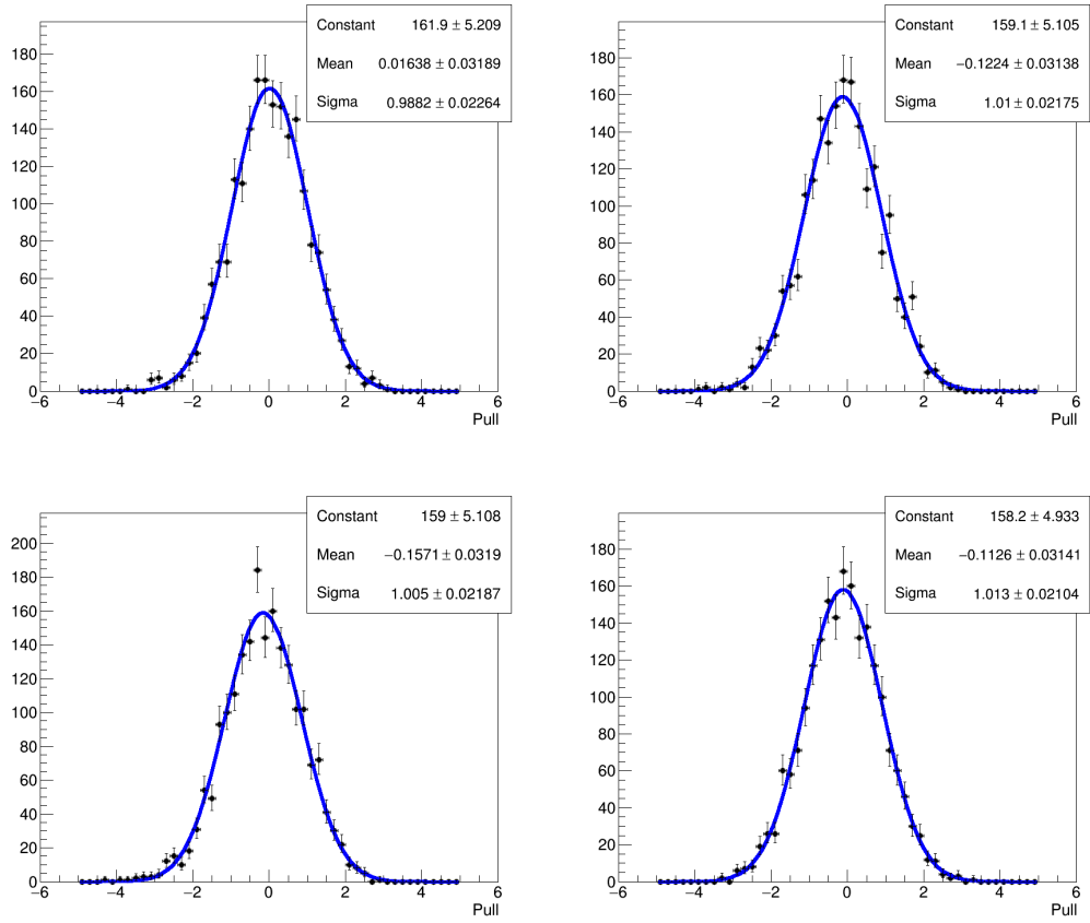
Figure 5-55: The B^+ pull distributions and the Gaussian fits for 0 - 90% at p_T 7 - 10, 10 - 15, 15 - 20, 20 - 50 GeV/c are shown respectfully above.
