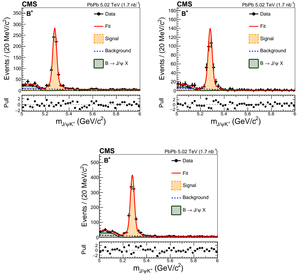
Figure 5-36: The B^+ invariant mass distributions as well as the fits to extract the signal raw yield N_S in different centrality bins are shown above.
