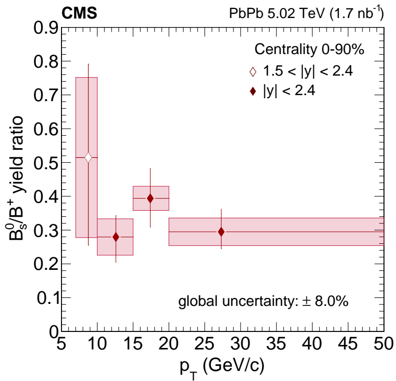
Figure 5-73: The measurement of B_s^0/B^+ as a function of p_T is shown above. The open markers from 7 - 10 GeV/c stand for the fiducial measurement at the B-meson rapidity of 1.5 < |y| < 2.4 .
