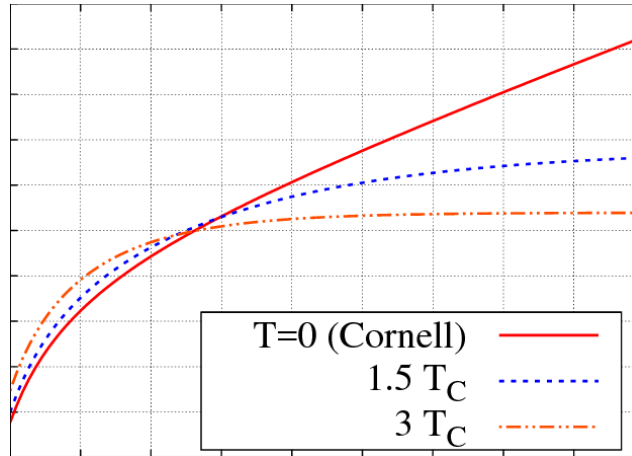
Figure 1-5: The QCD potential V(r) from at zero and finite temperatures as a function of distance r is shown above. Here, the critical temperature T_c = 192 MeV. We can see that V(r) saturates at a finite value at finite temperature.
