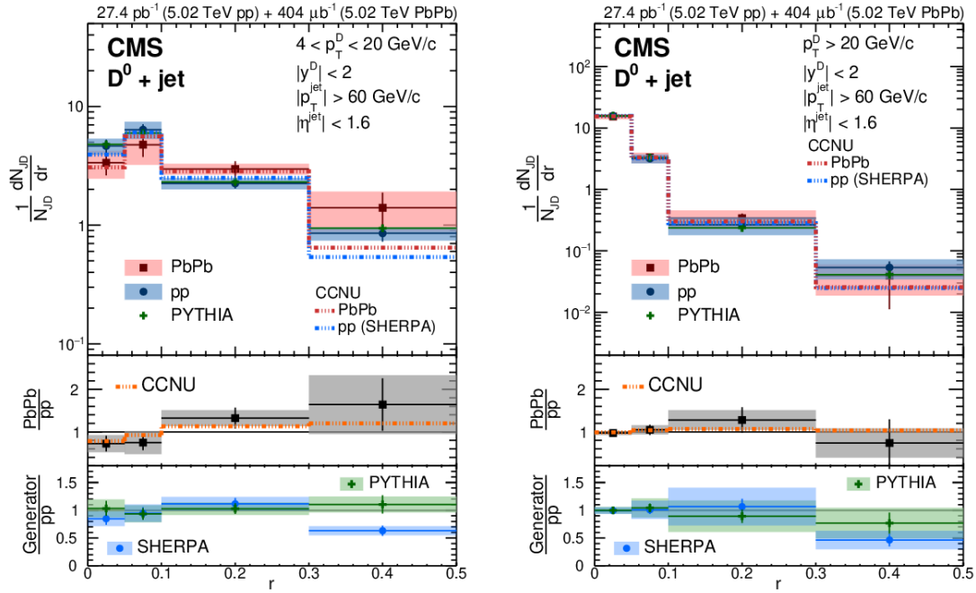
Figure 2-12: Distributions of fully reconstructed D^0 mesons in jets, as a function of the distance from the jet axis ( r ) for jets of p_T^{jet} > 60 \text{ GeV}/c and |\eta^{jet}| < 1.6 measured in pp and PbPb collisions at \sqrt{s_{NN}} = 5.02 \text{ TeV} , for 4 < p_T^D < 20 \text{ GeV}/c and p_T^D > 20 \text{ GeV}/c are shown above. The jet radius is defined as r = \sqrt{(\Delta\phi_{jD})^2 + (\Delta\eta_{jD})^2} where \phi_{jD} and \eta_{jD} are the \eta and \phi of the D^0 meson with respect to the jet axis.
