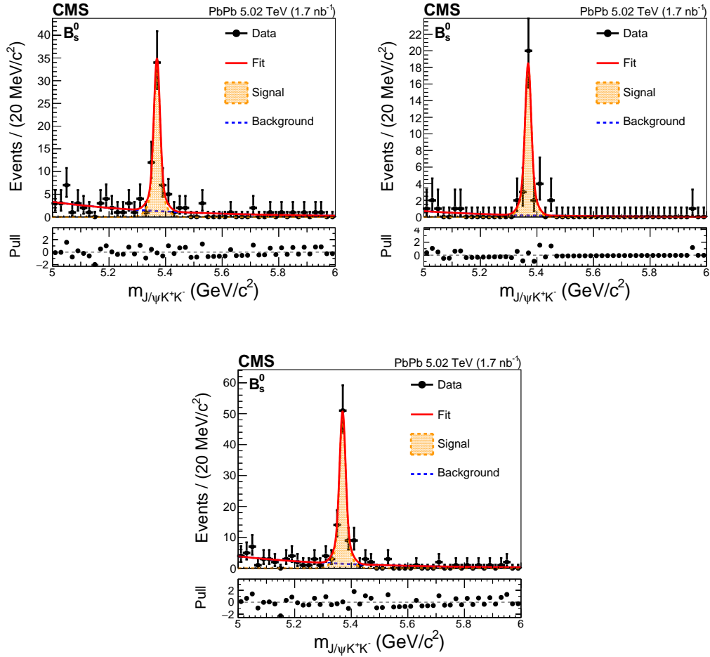
Figure 5-34: The B_s^0 invariant mass distributions as well as the fits to extract the signal raw yield N_S in different centrality bins are shown above.
