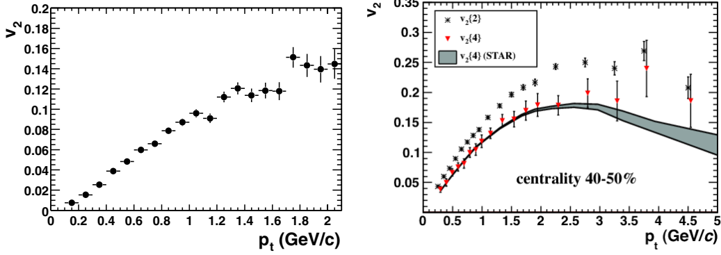
Figure 1-26: The elliptic flow v_2 of charged particles as a function of p_T in Au + Au collision measured by the STAR experiments at RHIC (left) and in PbPb collisions by the ALICE experiments at LHC (right) are shown above. Clearly, v_2 > 0 is observed in both experiments.
