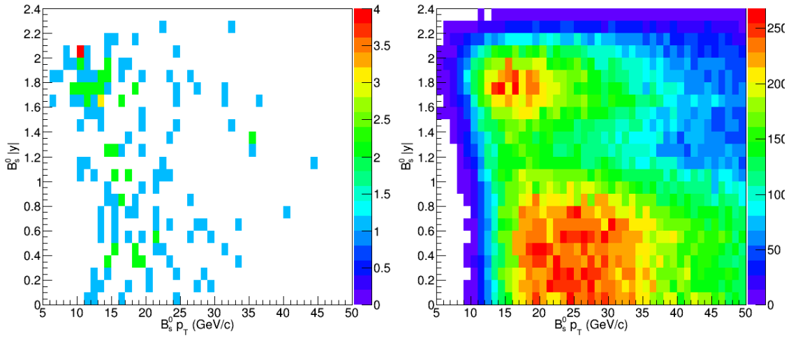
Figure 5-47: The finely binned 2D candidates distribution vs B p_T and B |y| for data and MC at centrality 0 - 90% are shown respectfully above.
