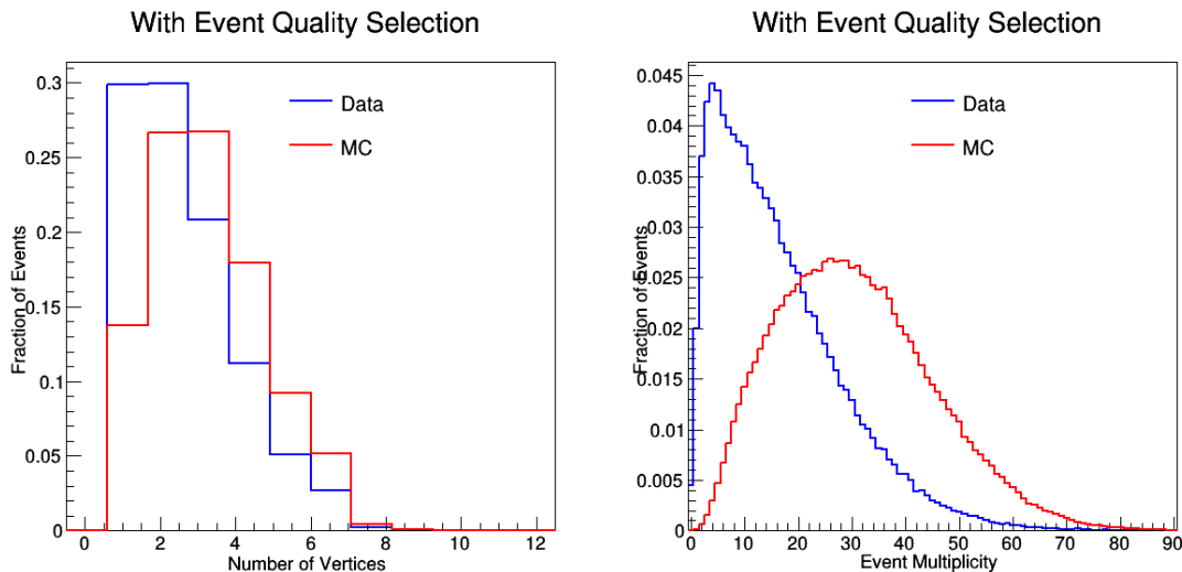
Figure 4-7: The Data (blue) and MC (red) of the number of primary vertex distribution (left) and event multiplicity (right) are shown above. We can see that an event could be more than one vertex with more than 100 tracks, which makes it very challenging to perform tracking.
