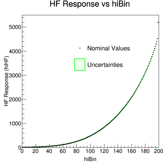
Figure 5-8: The nominal (black) and uncertainties band (green) hiHF vs hiBin for CMS 2018 PbPb dataset are shown above.
