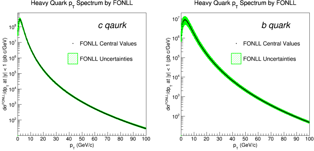
Figure 1-31: The charm quark (left) and beauty quark (right) differential cross section \frac{d\sigma}{dp_T} as a function transverse momentum p_T at |y| < 1 from FONLL calculations, are shown above.
