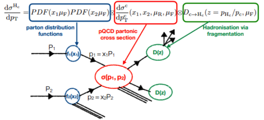
Figure 1-3: The QCD factorization theorem applied to study charm hadron production in a pp collision event involving soft and hard processes is shown schematically above.
