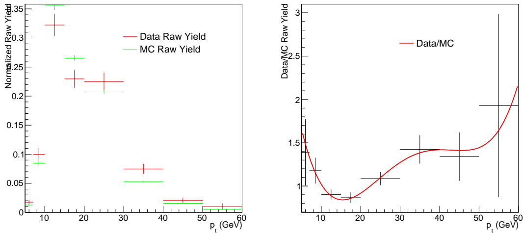
Figure 5-5: The normalized B^+ raw yield in MC (green) and Data (red) as a function RECO B^+ p_T (left) and the fourth-order polynomial fits to their ratio (right) are shown above.
