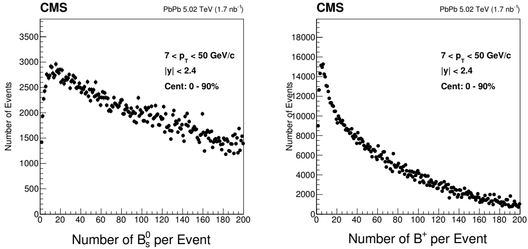
Figure 5-11: The number of reconstructed B-meson candidates per event distribution in the dimuon PbPb dataset for B_s^0 (left) and B^+ (right) are shown above. Multiple B-meson candidates are reconstructed in one event.
