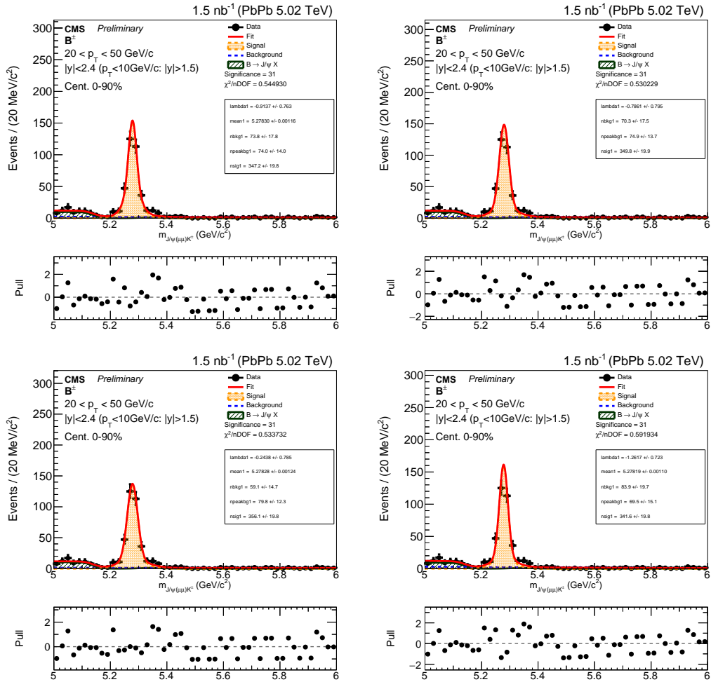
Figure 5-66: Invariant mass fit of B^+ candidates for B^+ p_T from 20 - 50 GeV/c and centrality from 0 to 90% in 5.02 TeV PbPb. The signal pdf from left to right is triple gaussian (with widths and relative proportions fixed from MC), double gaussian with all the parameters fixed (including the mean), increased width ( a=1.1 ), and decreased width ( a=0.9 ).
