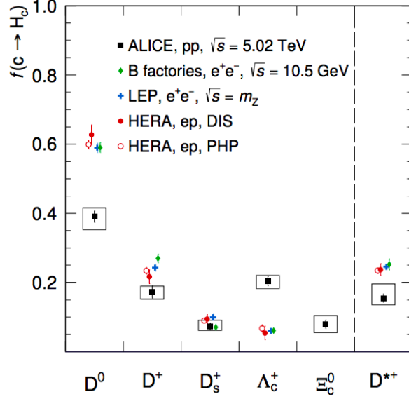
Figure 1-36: The charm quark fragmentation fraction to different charm hadrons species in e^+e^- , ep , and pp collisions are presented above. From the ALICE experiment, we can clearly see that the fragmentation fraction of D^0 has dropped by about 40% while the \Lambda_c^+ has enhanced by about a factor of 4. Therefore, the hadronization universality is clearly broken at the LHC energy in the charm sector.
