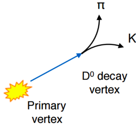
Figure 4-16: The decay of D^0 \rightarrow K^- \pi^+ with the definition of the secondary vertex is shown above
