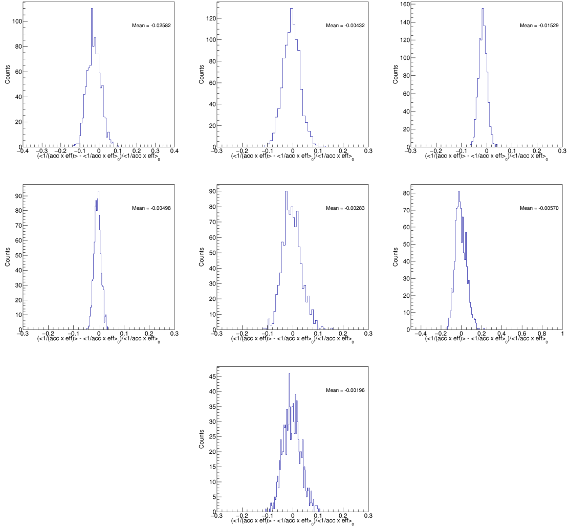
Figure 5-58: The percent deviation distributions of B^+ \langle \frac{1}{\alpha \times \epsilon} \rangle to RECO/GEN for the data-like randomly sampled MC samples for 0 - 90% at 7 - 10, 10 - 15, 15 - 20, and 20 - 50 GeV/c as well as 0 - 90%, 0 - 30%, and 30 - 90% event centrality are shown respectively above.
