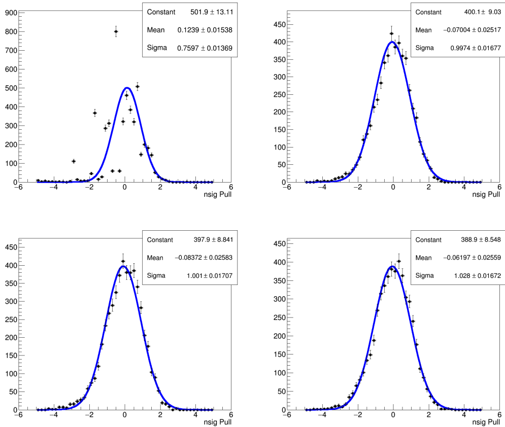
Figure 5-53: The B_s^0 pull distributions and the Gaussian fits for 0 - 90% at p_T 7 - 10, 10 - 15, 15 - 20, 20 - 50 GeV/c are shown respectfully above.
