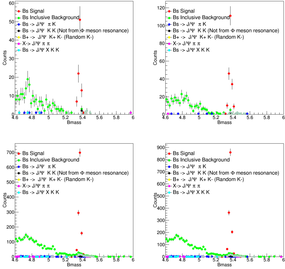
Figure 5-28: Individual Non Prompt background contributions with respect to the total background components and the signal channel for 10 to 15 GeV (top left), 15 to 20 GeV (top right), 20 to 50 GeV (bottom left), and 10 to 50 GeV (bottom right) for PbPb sample. We can see that the inclusive background is small compared to the signal we used in our studies.
