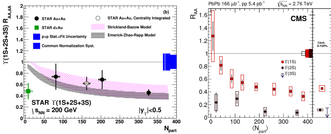
Figure 1-21: The nuclear modifications factor R_{AA} of fully reconstructed \Upsilon as a function of N_{part} measured by the STAR experiment (left) at RHIC and CMS experiment (right) at the LHC are shown above. We can see that the R_{AA} of the three \Upsilon states are below 1 when N_{part} > 3 . The \Upsilon R_{AA} decreases as N_{part} increases, consistent with the increasing creation probability of QGP with larger N_{part} . In addition, a sequential suppression of \Upsilon R_{AA} is observed by the CMS experiment: R_{AA}^{\Upsilon(1S)} > R_{AA}^{\Upsilon(2S)} > R_{AA}^{\Upsilon(3S)} , which agrees with the expectation of QGP color screening effect.
