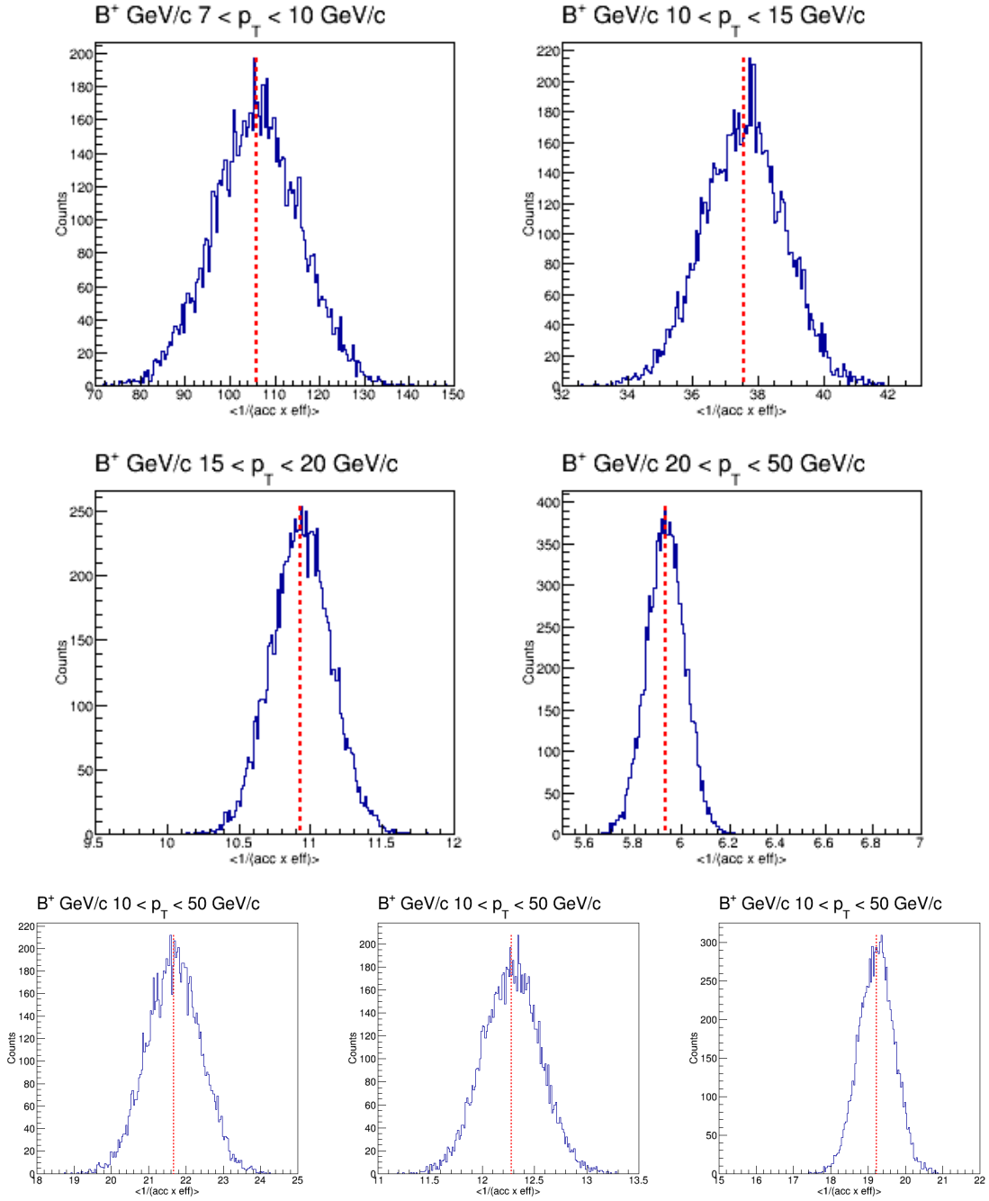
Figure 5-64: The distribution of B^+ \langle \frac{1}{\alpha \times \epsilon} \rangle for centrality in 0 - 90% in the p_T range of 7 - 10, 10 - 15, 15 - 20, and 20 - 50 GeV/c as well as 0 - 90%, 0 - 30%, and 30 - 90% in the p_T range of 10 - 50 GeV/c are shown above. The red dash lines are our nominal value for efficiency correction.
