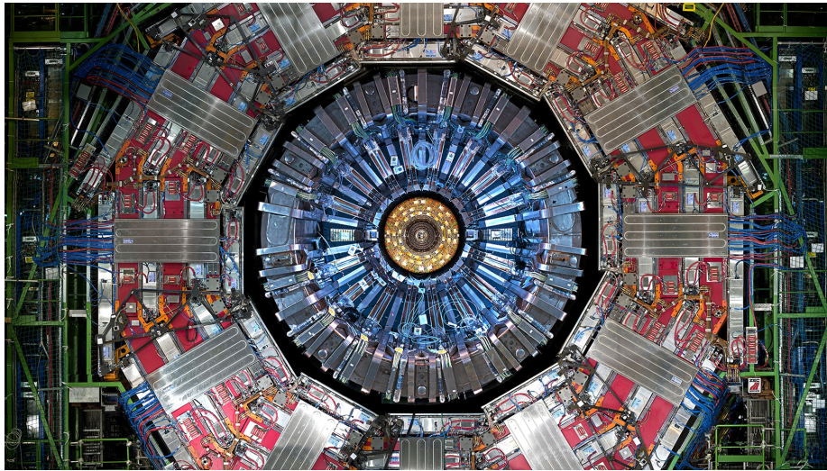
Figure 3-1: The front view of the CMS detector at the underground collision hall is shown above.
