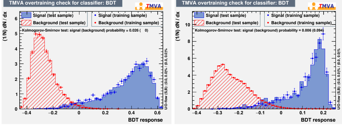
Figure 5-23: The Kolmogorov-Smirnov overtraining tests on the signal (blue) and background (red) in B_s^0 (left) and B^+ (right) at 10 < p_T < 15\text{GeV}/c are shown on the right. It looks like they both pass the tests.
