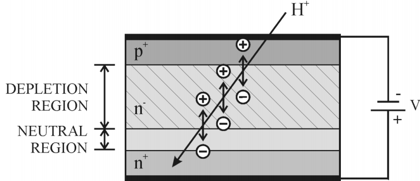
Figure 3-10: The schematic plot explaining how a silicon tracker detector charged particles is shown above.
