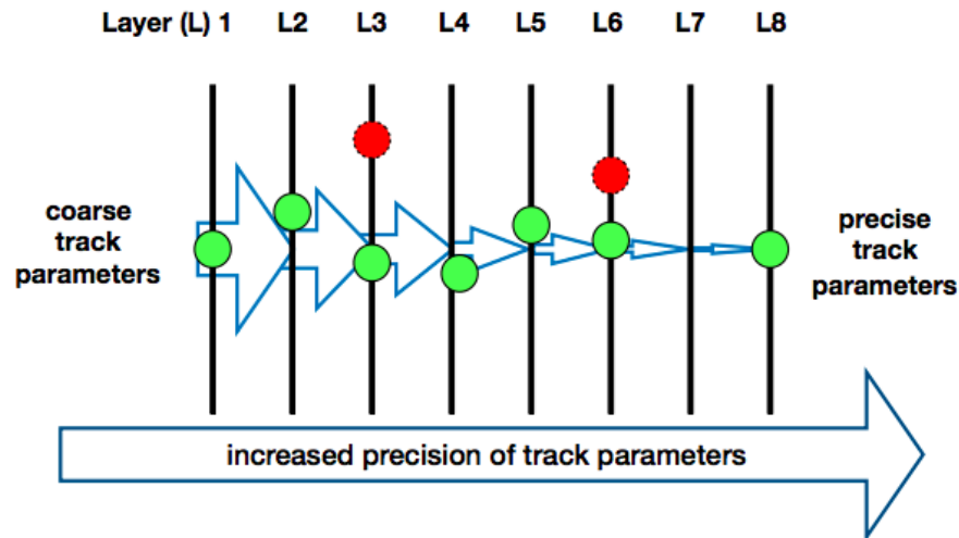
Figure 4-11: The schematic demonstration Kalman filter along with Rugga-Katta propagator to improve the tracks fitting is shown above.
