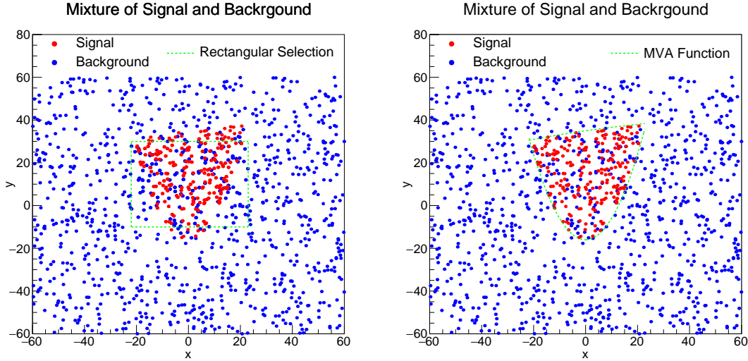
Figure 5-16: The performance of traditional rectangular selection with a range of x and y (left) compared to the MVA method of a curve as a function of X and Y (right) are shown above. Here, we have the total signal S = 215 and the background B = 1000 .
