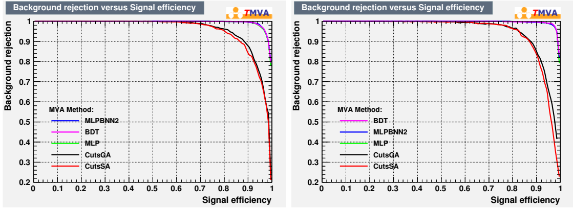
Figure 5-22: The B_s^0 ROC curves of CutsSA, CutsGA, BDT, MLP, and MLPBNN2 algorithms are shown above.
