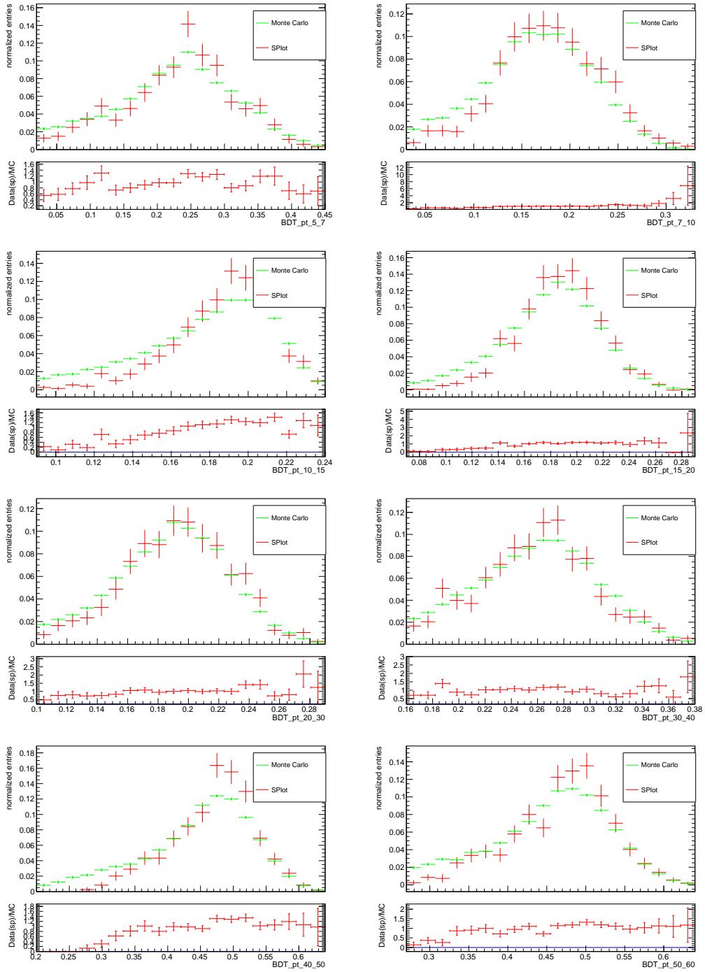
Figure 5-43: Comparison of B^+ BDT distribution in data (red) and MC (green) using the Splot method.
