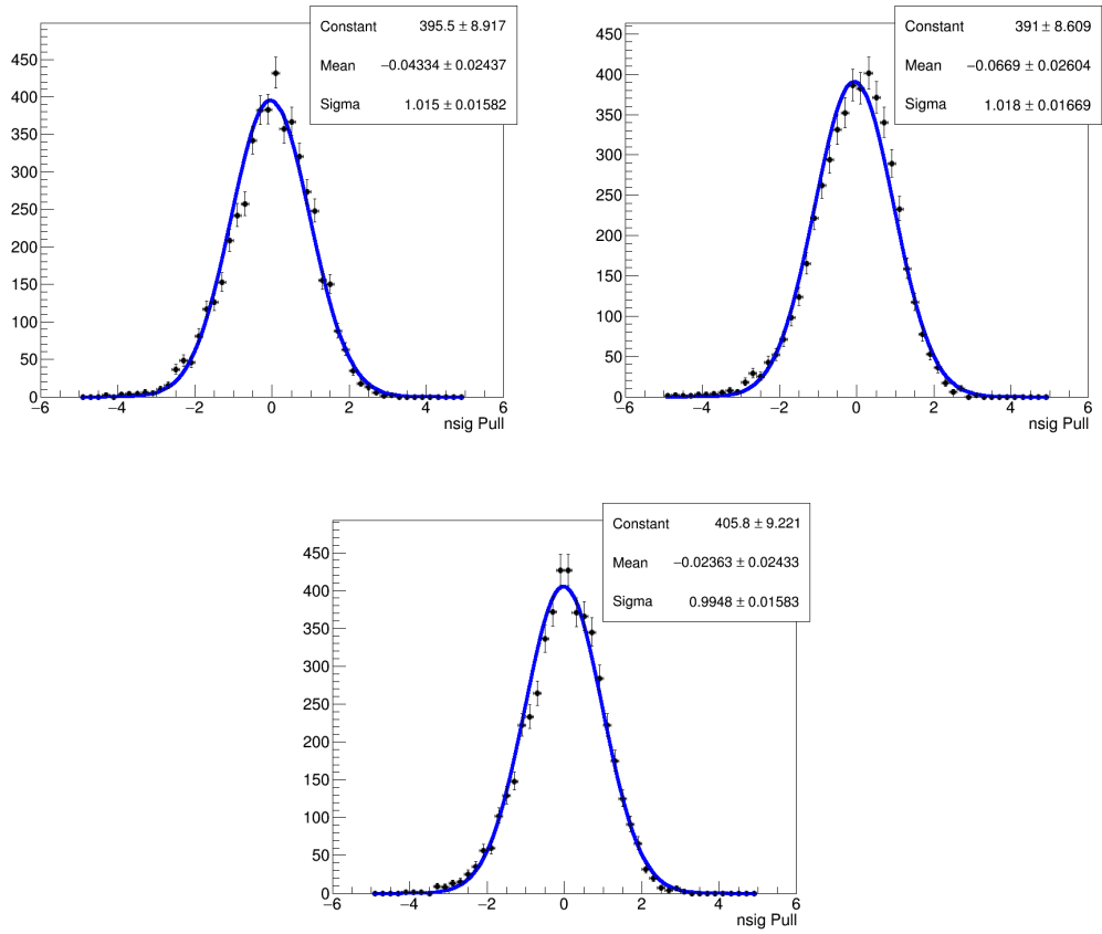
Figure 5-54: The B_s^0 pull distributions and the Gaussian fits for 0 - 30%, 30 - 90%, and 0 - 90% event centrality are shown respectively above.
