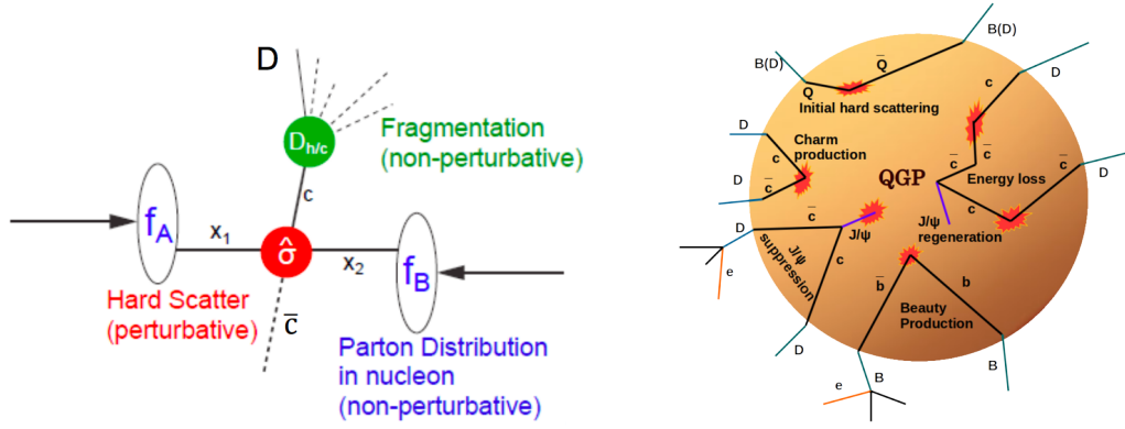
Figure 1-30: The schematic demonstrations of heavy quark production and hadronization in vacuum (left) and QGP (right) are shown above.
