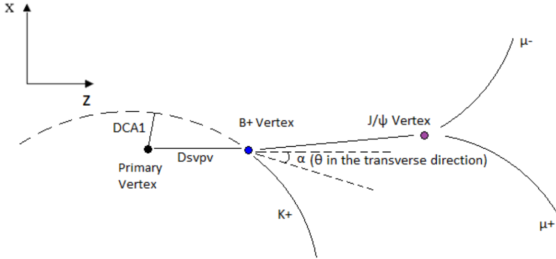
Figure 5-15: The definition of topological variables in the decay of B^+ \rightarrow J/\psi K^+ \rightarrow \mu^+ \mu^- K^+ are schematically shown above.
