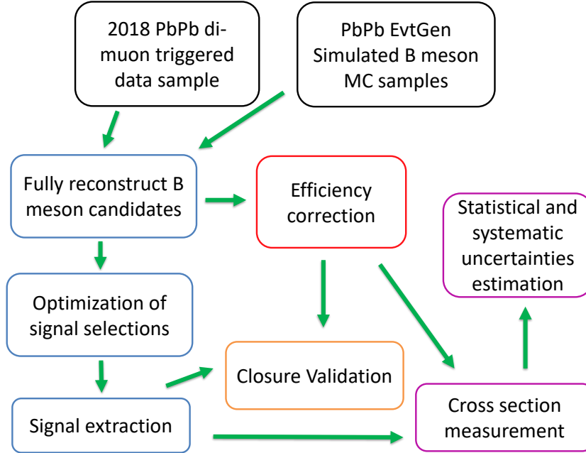
Figure 5-1: The block diagram of the workflow with major steps for both B-meson cross section measurements is shown above.
