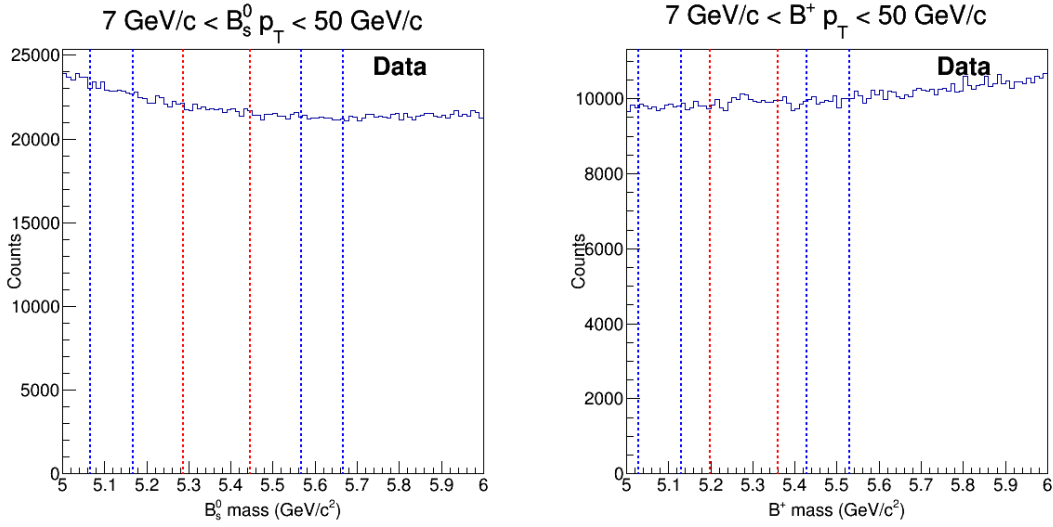
Figure 5-18: The definitions of signal (red band) and background region (blue band) in the fully reconstructed B-meson invariant distribution for B_s^0 (left) and B^+ (right) are shown above.
