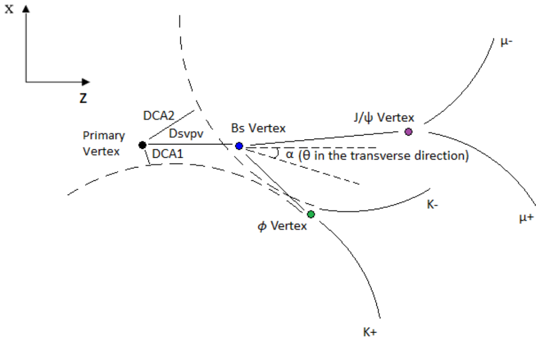
Figure 5-14: The definition of topological variables in the decay of B_s^0 \rightarrow J/\psi \phi \rightarrow \mu^+ \mu^- K^+ K^- (left) are schematically shown above.
