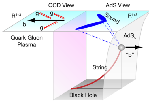
Figure 1-38: The schematic demonstration of ADS/CFT picture: a quark loses energy in the QGP medium holographically due AdS/CFT drag force.
