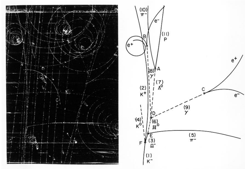
Figure 4-1: The bubble chamber picture of an \Omega^- baryon reconstructed from an event: K^-p \rightarrow K^0K^+\Omega^- \rightarrow \Xi^0\pi^- \rightarrow \Lambda^0\gamma\gamma \rightarrow \pi^-p taken from the group led by Nicholas Samios at BNL is shown above.
