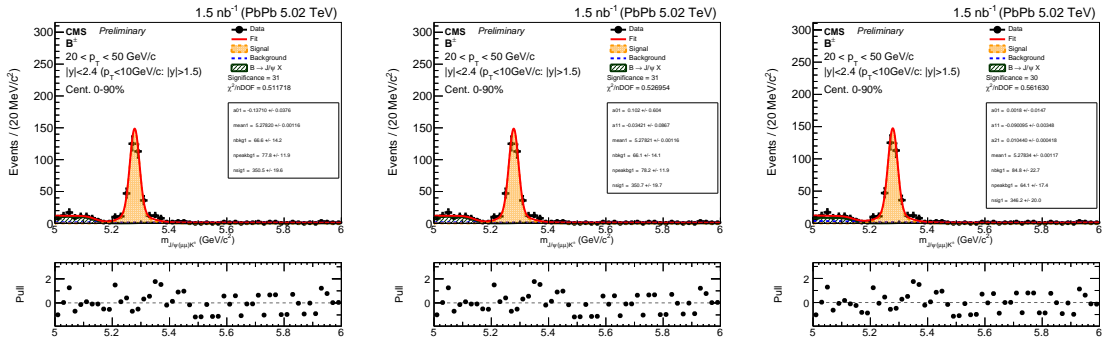
Figure 5-68: Invariant mass fit of B^+ candidates for B^+ p_T from 20 - 50 GeV/c and centrality from 0 to 90% in 5.02 TeV PbPb. The background PDFs from left to right are first-, second-, and third-order polynomials.
