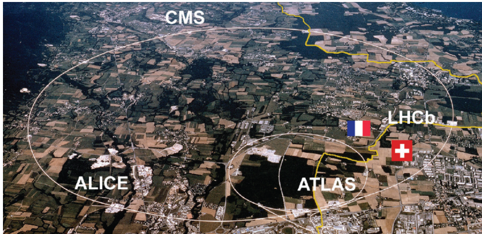
Figure 1-10: The sky view of LHC at CERN is shown above. The actual locations of the experiments at the LHC: ATLAS, CMS, ALICE, and LHCb, as well as the French-Swiss border, are also displayed.
