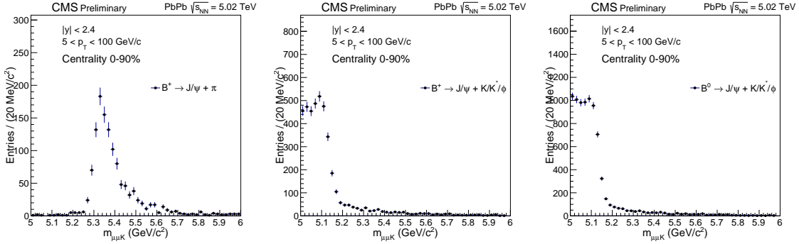
Figure 5-31: Peaking background contribution from B^+ \rightarrow J/\psi\pi and from K resonant decay channels of B^0 and B^+ in PbPb MC.
