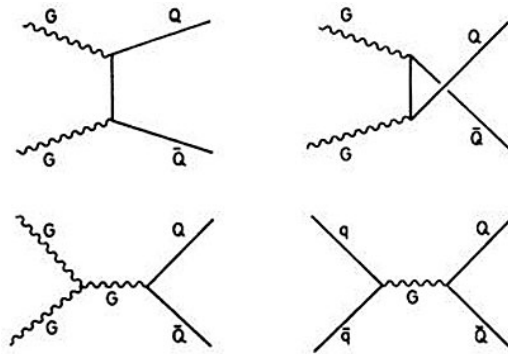
Figure 1-29: The four lowest order tree-level Feynman diagrams of heavy quark pair production are shown above.
