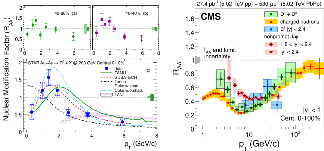
Figure 2-5: The fully reconstructed D^0 R_{AA} vs p_T with the STAR experiment in 0 - 10%, 10 - 40%, and 40 - 80% centrality at RHIC and the D^0 , B^+ , non-prompt J/\psi and charged hadrons R_{AA} vs p_T at 0 - 100% centrality with the CMS experiment at LHC are shown above.
