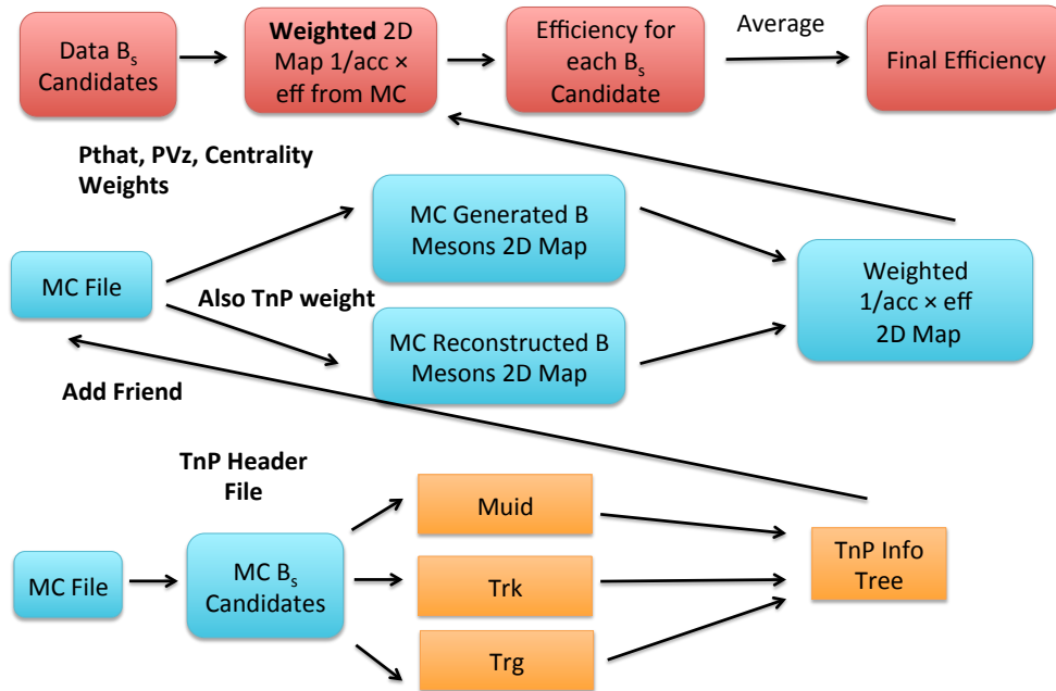
Figure 5-48: The workflow for the efficiency correction including the data-driven tag-&-probe approach in B-meson analysis is shown above.
