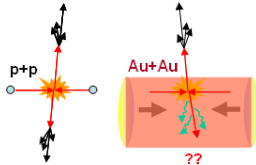
Figure 1-23: The schematic picture explaining jet quenching is shown above. Hard scatterings in pp collisions produce back-to-back "jets" of particles, but in Au + Au collisions, the presence of QGP modifies the jets' properties.
