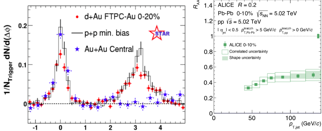
Figure 1-24: The comparison of two-particle azimuthal distributions for central d + Au collisions to those seen in pp and central Au + Au collisions measured with the STAR experiment and the jet R_{AA} as a function p_T measured by the ALICE experiment at LHC (right). From the STAR results, in central Au + Au collisions, the back-to-back peak has disappeared due to the redistribution of jet energy to the slow expanding medium constituents. The jet R_{AA} from ALICE measurement is clearly below 1, suggesting that jets lose significant fractions of energy in AA collision compared to pp .
