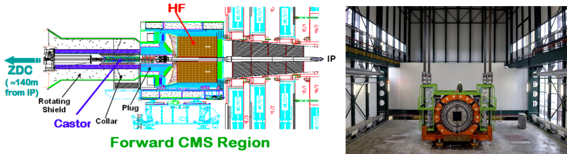
Figure 3-13: The schematic view of the CMS forward region including HF, CASTOR, and ZDC (left) and the physical view of the HF (right) are shown above.
