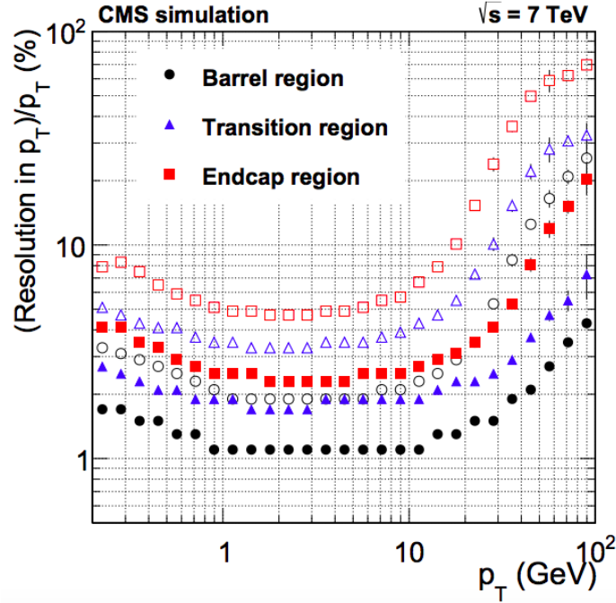
Figure 4-6: The transverse momentum resolution \frac{\sigma_{p_T}}{p_T} of a track as a function of transverse momentum p_T is shown above.
