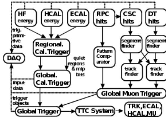
Figure 3-3: The figure above demonstrates how the CMS L1 hardware trigger function schematically.
