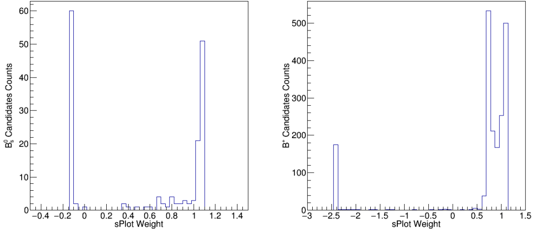
Figure 5-59: The sPlot weight distributions for B_s^0 (left) and B^+ (right) candidates are shown above.
