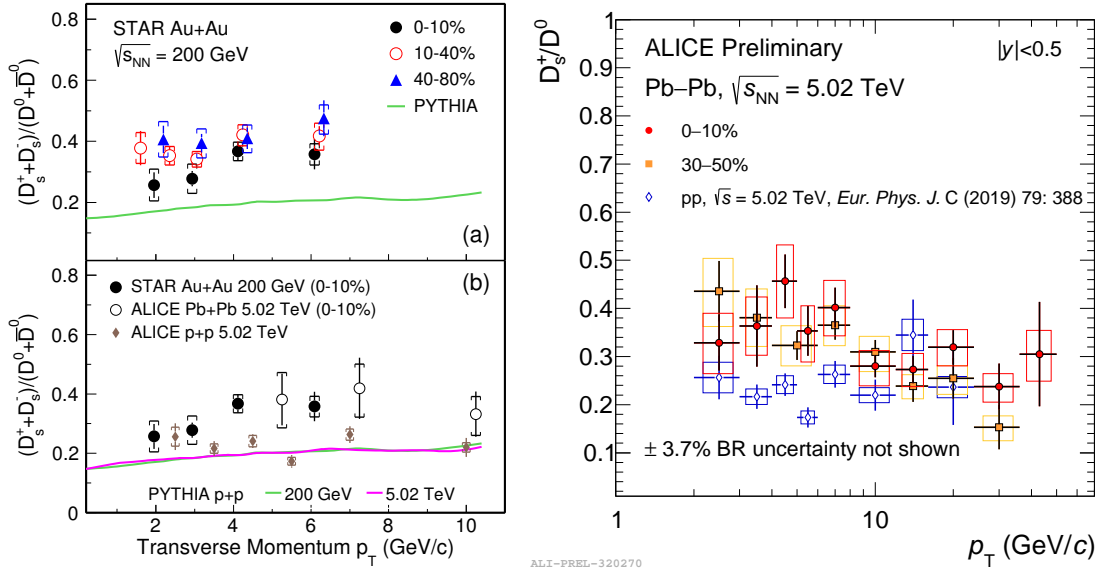
Figure 2-7: The fully reconstructed D_s^+/D^0 ratio in Au + Au measured by the STAR experiment at RHIC (left) and in PbPb the ALICE experiment at LHC (right) as functions of p_T are shown above.
