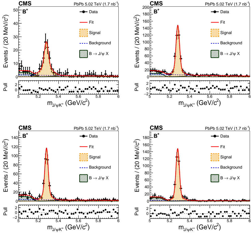
Figure 5-35: The B^+ invariant mass distributions as well as the fits to extract the signal raw yield N_S in different p_T bins are shown above.
