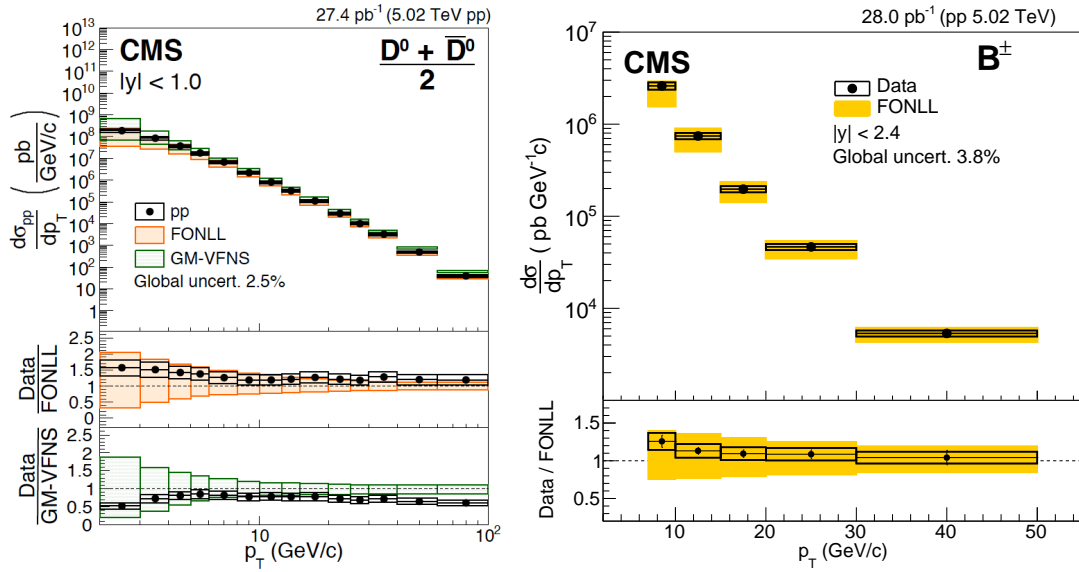
Figure 1-32: The charm quark (left) and beauty quark (right) p_T spectra and the ratio with FONLL and GM-VFNS pQCD theoretical calculations are shown above.
