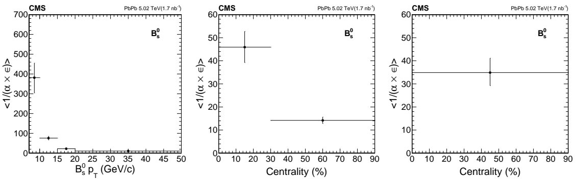
Figure 5-51: The B_s^0 efficiency correction factor \langle \frac{1}{\alpha \times \epsilon} \rangle vs p_T (left) and 0 - 30 % and 30 - 90% centrality (middle) and the inclusive 0 - 90% centrality (right) are shown above.
