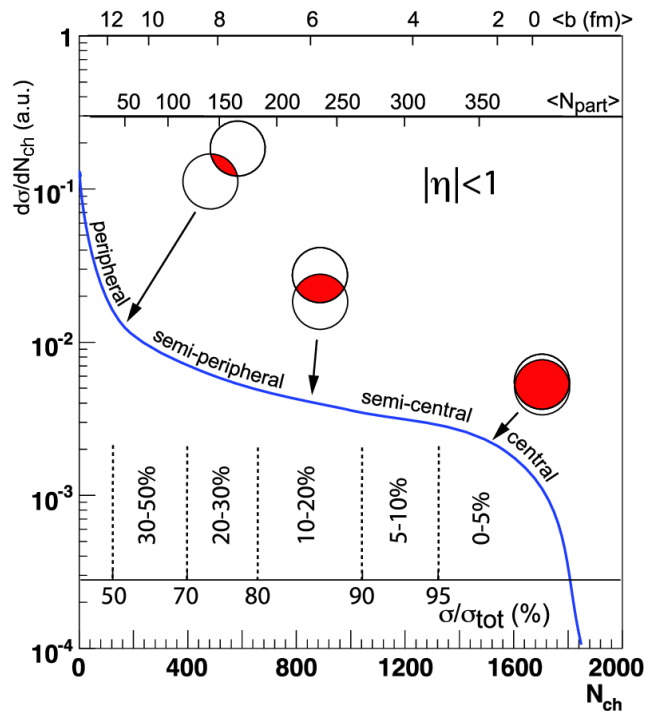
Figure 1-16: The plot showing a relationship among the number of charged particles, N_{ch} , related to the number of participants N_{part} , the differential cross section \frac{d\sigma}{dN_{ch}} , and the centrality, according to the Glauber Model calculations, is shown above.
