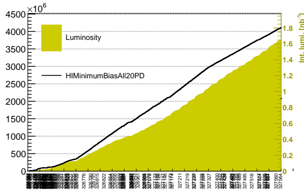
Figure 3-6: The figure above shows the total number of 20 PbPb MB events from and corresponding luminosity how the as a function Run ID from November 15 to December 2, 2018.
