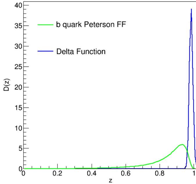
Figure 1-34: The comparison between the Peterson fragmentation function (green) and the delta function (blue) is shown above.
