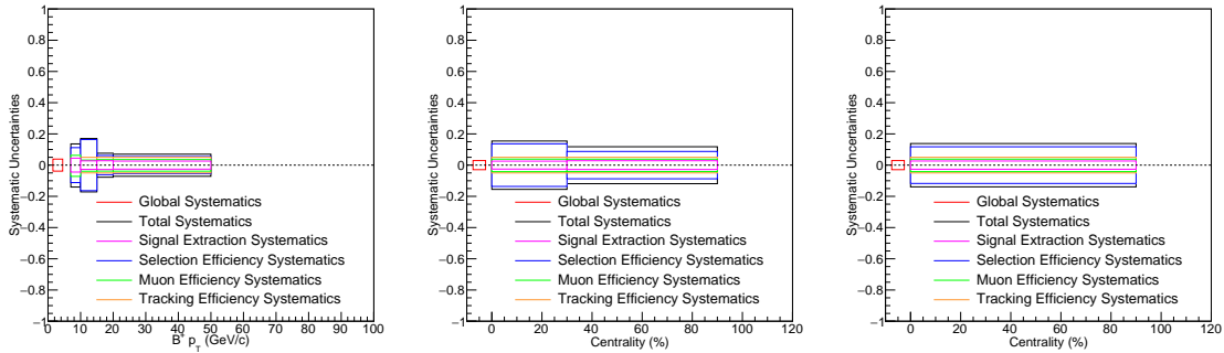
Figure 5-70: The summary of B^+ systematic uncertainties plotted as a function of p_T (left), centrality in 0 - 30%, and 30 - 90% (middle), and the inclusive centrality bin 0 - 90% (right) are shown above.
