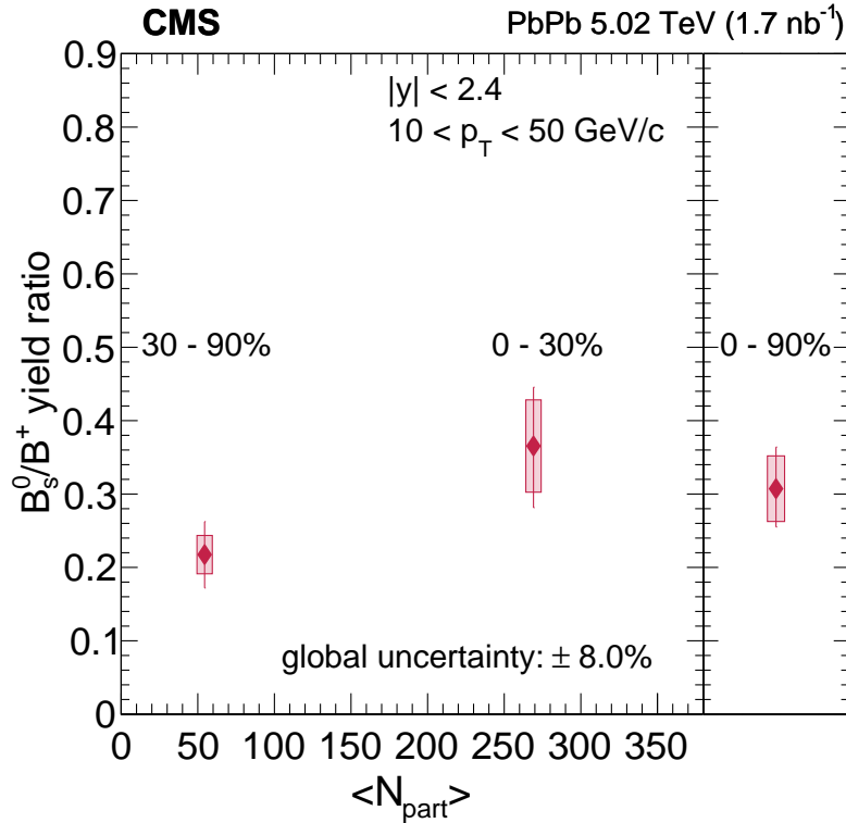
Figure 5-74: The measurement of B_s^0/B^+ as a function of p_T is shown above.
