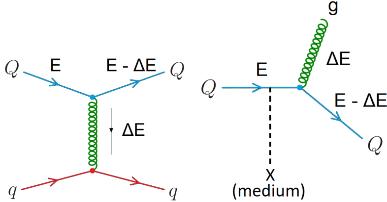
Figure 1-37: The schematic demonstration of the pQCD picture: collisional energy loss (left) and radiative energy loss (right) of heavy quarks in the QGP medium.
