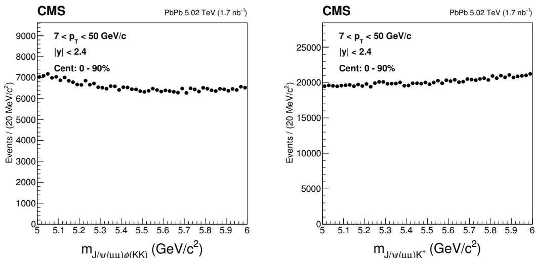
Figure 5-13: The invariant mass distributions of fully reconstructed B_s^0 (left) and B^+ (right) after preselection are shown above.
