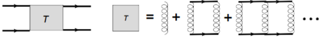
Figure 1-40: The ladder diagram used by the TAMU model to describe heavy quark diffusion in the QGP medium is shown schematically above.
