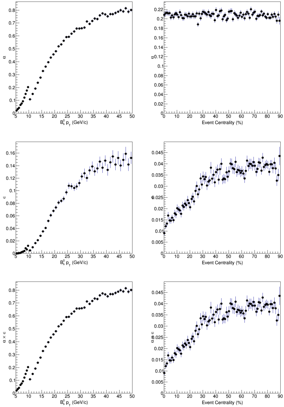
Figure 5-45: The B_s^0 acceptance (top), selection efficiency (middle), and efficiency (bottom) as a function of p_T (left) and event centrality (right) are shown respectively above. We should note that there is no significant centrality dependence on the B_s^0 acceptance, which makes sense.
