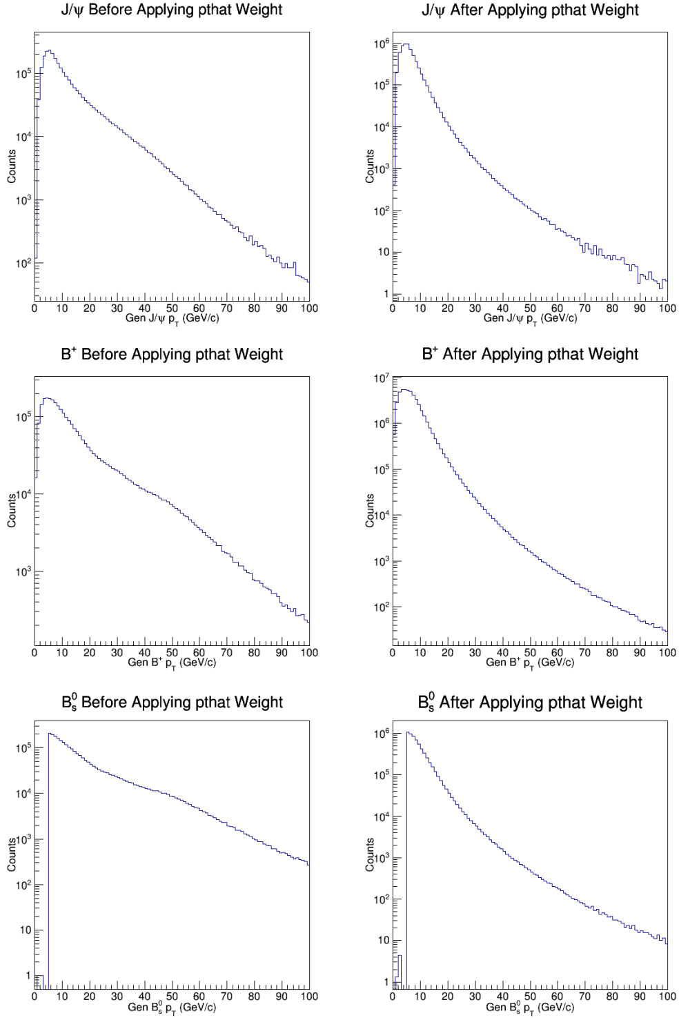
Figure 5-3: J/\psi generated p_T distribution before (upper left) and after (upper right) \hat{p}_T reweighing, B^+ generated p_T distribution before (middle left) and after (middle right) \hat{p}_T reweighing, and B_s^0 generated Gp_T distribution before (lower left) and after (lower right) \hat{p}_T reweighing are shown above.
