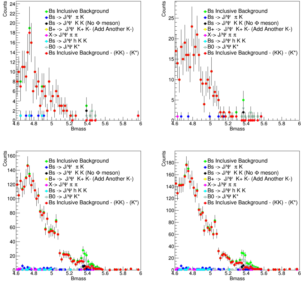
Figure 5-27: Individual NP background contributions with respect to the total background components for 10 to 15 GeV (top left), 15 to 20 GeV (top right), 20 to 50 GeV (bottom left), and 10 to 50 GeV (bottom right) for PbPb sample. We can see that the non-prompt background from all channels listed above is negligible compared to the inclusive background. Also, no peak near the B_s^0 resonance is observed when the inclusive background subtracts the B^0 \rightarrow J/\psi K^{*0} and B_s \rightarrow J/\psi K^+ K^- components.
