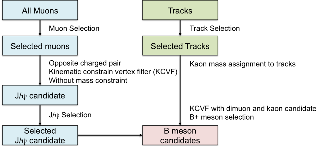
Figure 5-10: The schematic block diagram of the full reconstruction workflows for B^+ via the decay channel of B^+ \rightarrow J/\psi K^+ \rightarrow \mu^+ \mu^- K^+ in the Bfinder is shown above.
