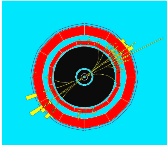
Figure 1-22: The schematic display of a di-jet event from the ALEPH (a particle detector at the Large Electron-Positron collider) Experiment at the Large Electron-Positron Collider (LEP) is shown above. We can see two sprays of back-to-back particles within a narrow cone, representing a di-jet event.
