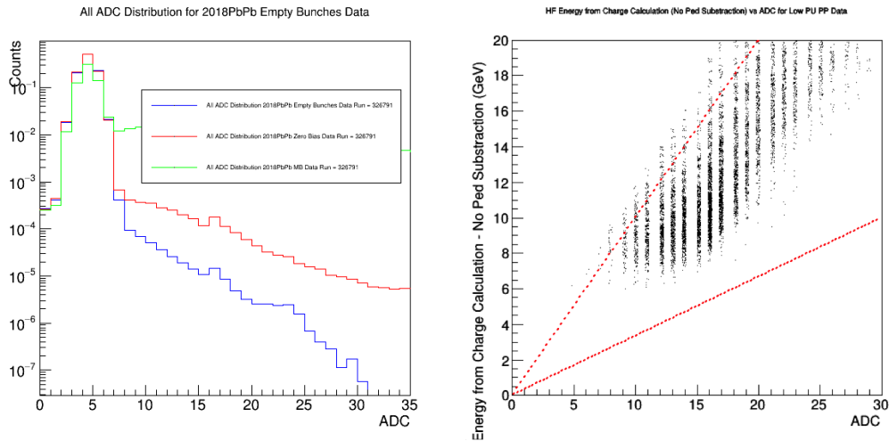
Figure 3-4: In the CMS 2018 PbPb Run 326791, the ZB data (red), Empty Bunches (blue), and MB data (green) ADC distributions (left), and the HF energy according to the charge collected as a function of ADC (right) are shown above. We can see that the HF energy is about (0.5 - 1) conversion factor to the ADC.
