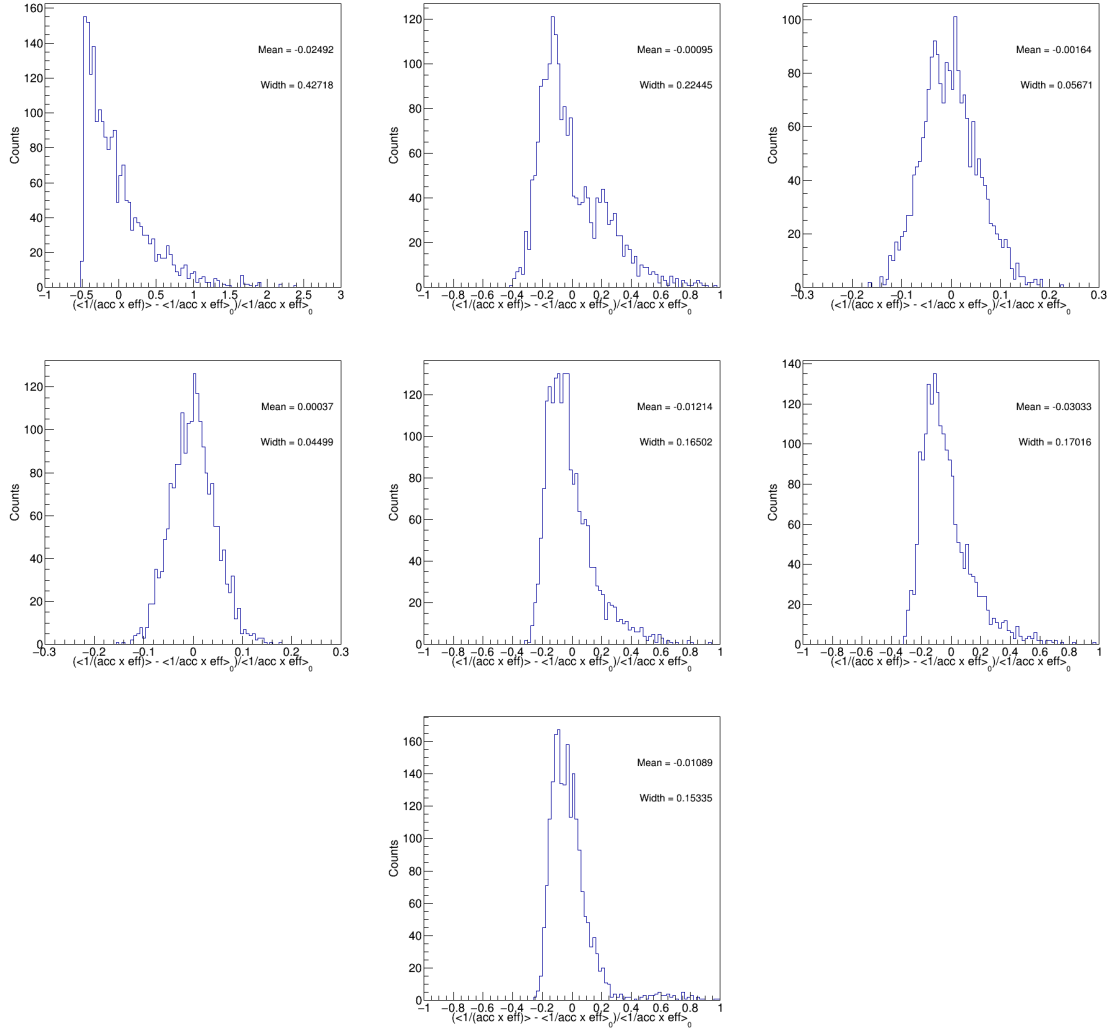
Figure 5-57: The percent deviation distributions of B_s^0 \langle \frac{1}{\alpha \times \epsilon} \rangle to RECO/GEN for the data-like randomly sampled MC samples for 0 - 90% at 7 - 10, 10 - 15, 15 - 20, and 20 - 50 GeV/c as well as 0 - 90%, 0 - 30%, and 30 - 90% event centrality are shown respectfully above.
