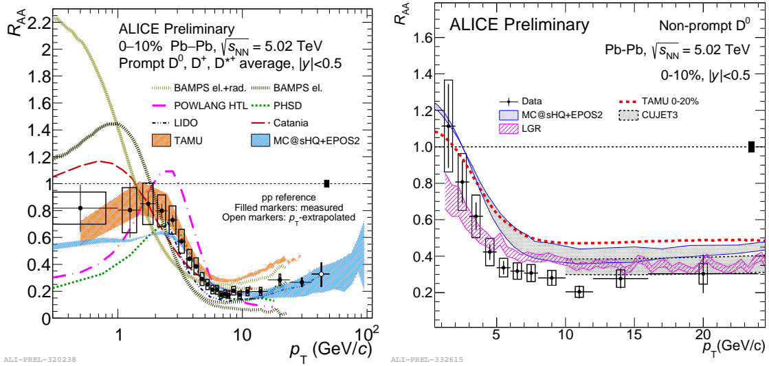
Figure 2-6: The R_{AA} of prompt D mesons vs p_T down to p_T = 0 (left) and non-prompt D mesons down to p_T = 1 GeV/c (right) are shown above.
