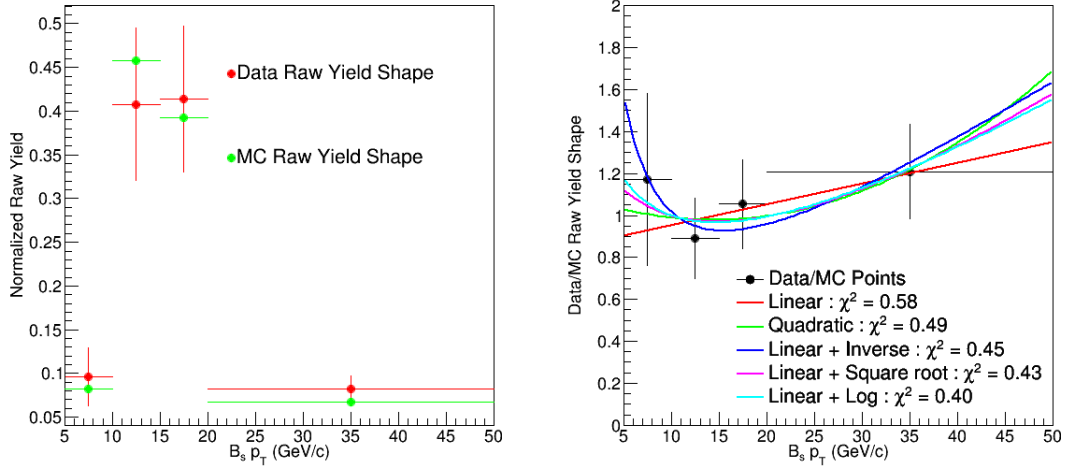
Figure 5-4: B_s^0 p_T normalized raw yields obtained in PbPb MC and Data are shown above on the top left panel. The data/MC ratio and different fitting functions: Linear (Red), Quadratic(Green), Linear + Inverse (Blue), Linear + Square Root (Purple), and Linear + Log (Cyan) and their \chi^2 are shown above on the top right panel. The bottom plots are the data/MC reweighed yields with different functions from the fit on the top right panel.
