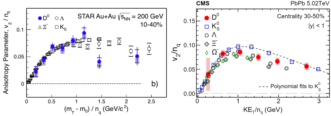
Figure 2-1: The NCQ scaled D^0 v_2/n_q vs K_T/n_q and the comparison of light hadrons measured by the STAR experiment at RHIC (left) and the CMS experiment at LHC (right) are shown above.
