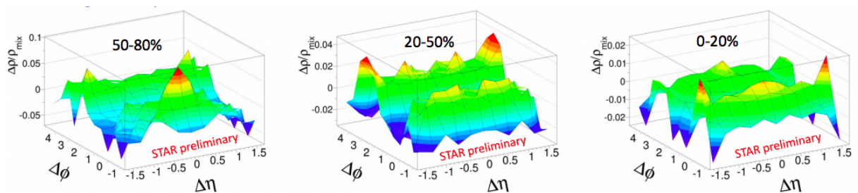
Figure 2-14: The 2D \Delta\eta \times \Delta\phi distributions of D^0 meson and associated hadrons in Au + Au collision centrality 0 - 20%, 20 - 50%, and 50 - 80% at \sqrt{s_{NN}} = 200 GeV measured by STAR experiment are shown above.
