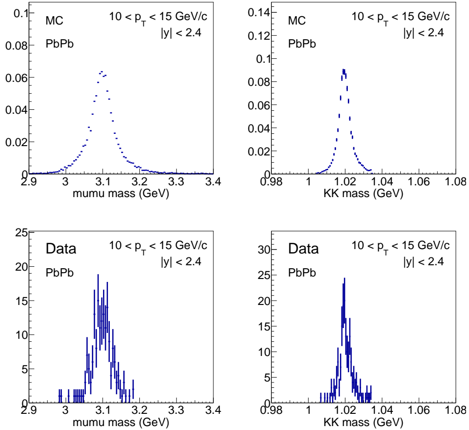
Figure 5-25: The J/\psi (left) and \phi (right) meson mass distributions after applying \text{BDT} > 0 for MC (top) and data (low) in B_s^0 analysis are shown above.
