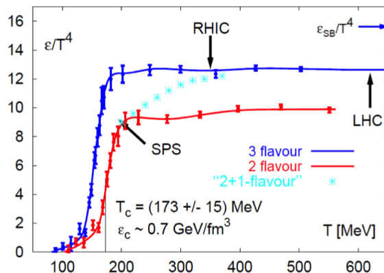
Figure 1-7: The reduced energy density \epsilon/T^4 as a function of temperature T for different numbers of flavor scenarios from the lattice QCD calculations (data points) and the interpolation curves are shown above.
