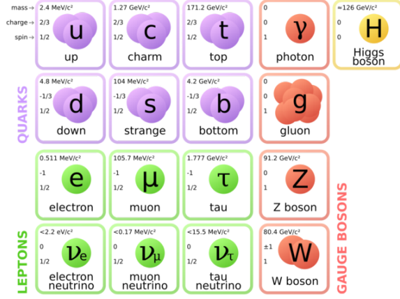
Figure 1-1: The 17 elementary particles, including 6 leptons, 6 quarks, 4 gauge bosons, and the Higgs boson, and their basic properties, such as mass, electric charge, spin, in the Standard Model of Particles Physics are shown above.
