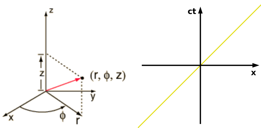
Figure 1-12: The cylindrical coordinate system in the position space (left) and the space-time diagram (right) for relativistic heavy-ion physics analysis are shown above.
