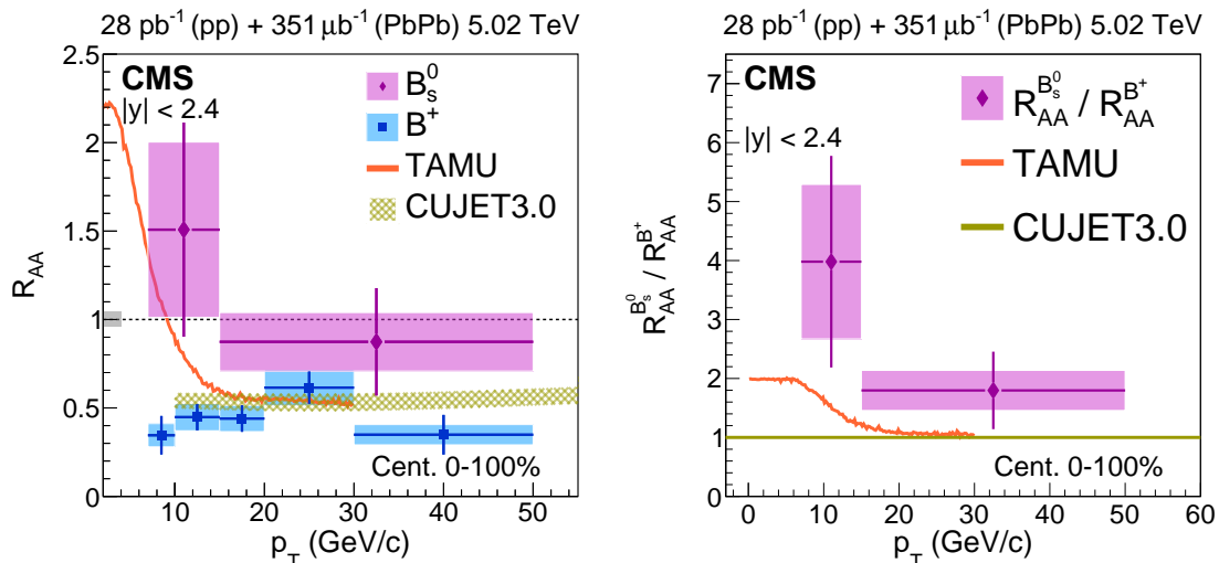
Figure 2-10: The fully reconstructed B_s^0 and B^+ R_{AA} (left) and B_s^0/B^+ R_{AA} ratio (right) as a function of p_T using the 2015 CMS pp and PbPb datasets are shown above.
