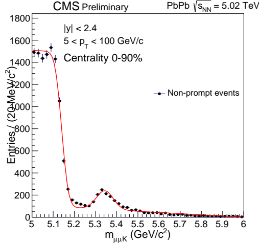
Figure 5-30: B^+ candidate mass spectrum obtained in inclusive B-meson MC production after vetoing the contribution of genuine B^+ signal candidates in PbPb.
