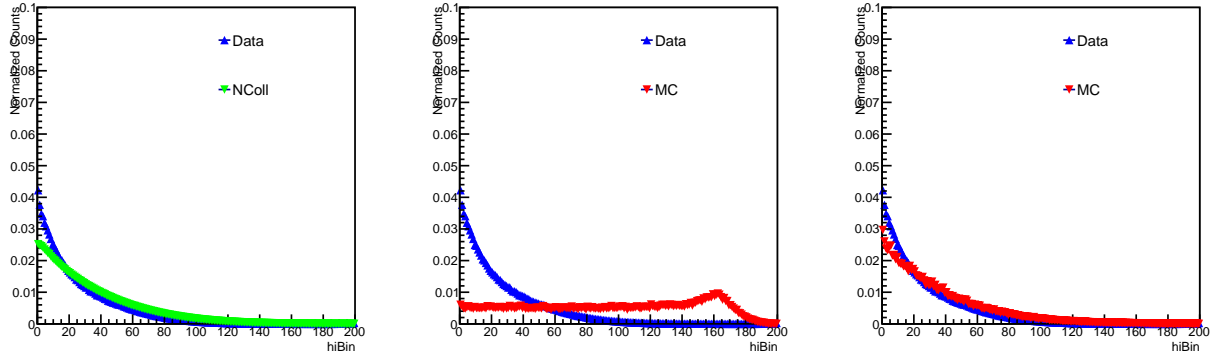
Figure 5-6: The comparison between N_{coll} and Data vs hiBin (left), centrality distribution of MC (red) and data (blue) in PbPb collisions in the centrality interval 0-100% without N_{coll} weight (middle), and with N_{coll} weight (right) are shown above.
