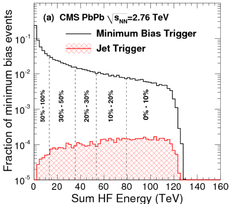
Figure 3-14: The distribution of the sum of HF energy using Minimum Biased Trigger and Jet Trigger with the classification of centrality binning is shown above. As we can see, the energy of the HF increase as the collision events become more central, which is within our expectation.
