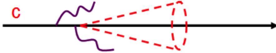
Figure 1-39: The schematic demonstration of a charm quark radiation is shown above. A suppression in small angles due to the dead cone effect in the QGP medium is highlighted.
