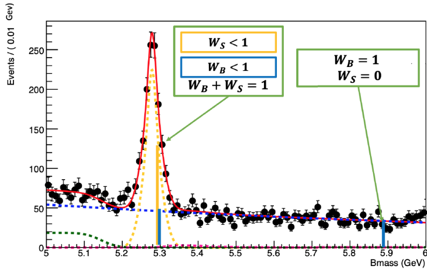
Figure 5-39: The illustration of Splot techniques via an unbinned fit to B^+ invariant mass distribution using our fitting model to extract the Splot weights w_S and w_B is shown above.
