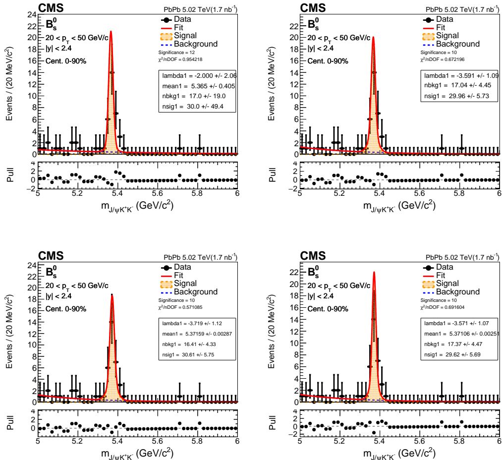
Figure 5-65: Invariant mass fit of B_s^0 candidates for B_s^0 p_T from 20 - 50 GeV/c and centrality from 0 to 90% in 5.02 TeV PbPb. The signal pdf from left to right is triple gaussian (with widths and relative proportions fixed from MC), double gaussian with all the parameters fixed (including the mean), increased width ( a=1.1 ), and decreased width ( a=0.9 ).
