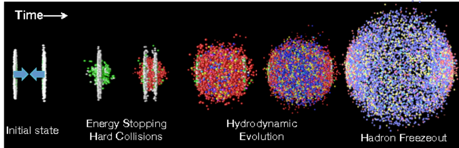
Figure 1-13: A typical heavy-ion collision event with different stages as time evolves is shown above.
