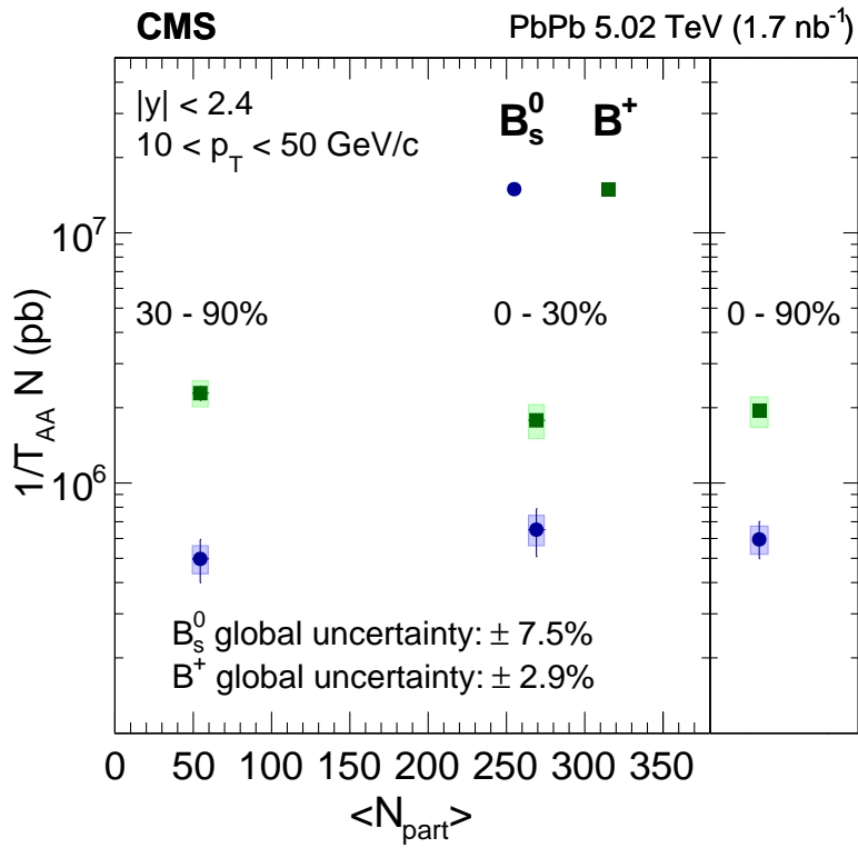
Figure 5-72: The measurement of B_s^0 and B^+ p_T differential cross section \frac{1}{T_{AA}} \frac{dN}{dp_T} measurement as a function of \langle N_{part} \rangle at different PbPb collision centrality within B-meson p_T from 10 - 50 GeV/c is shown above.
