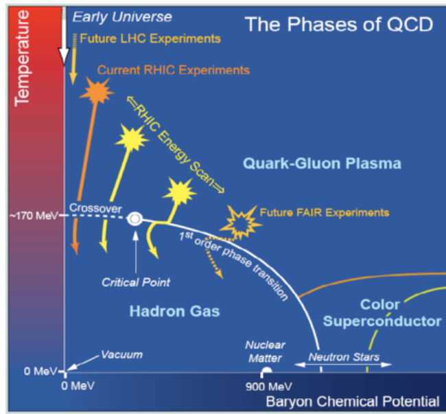
Figure 1-6: The theoretical QCD phase diagram of different QCD matter, including hadron resonance gas, quark-gluon plasma, neutron star, and color superconductor, as a function of temperature and baryon chemical potential, is shown above. The solid line indicates the conjecture of first-order phase transition between quark-gluon plasma and hadron gas while the dashed line is a smooth crossover. Thermodynamically, a critical point must exist in the boundary of smooth crossover and first-order phase transition.
