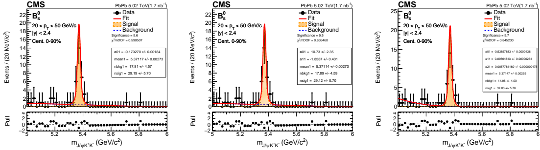
Figure 5-67: Invariant mass fit of B_s^0 candidates for B_s^0 p_T from 20 - 50 GeV/c and centrality from 0 to 90% in 5.02 TeV PbPb. The background PDFs from left to right are first-, second-, and third-order polynomials.
