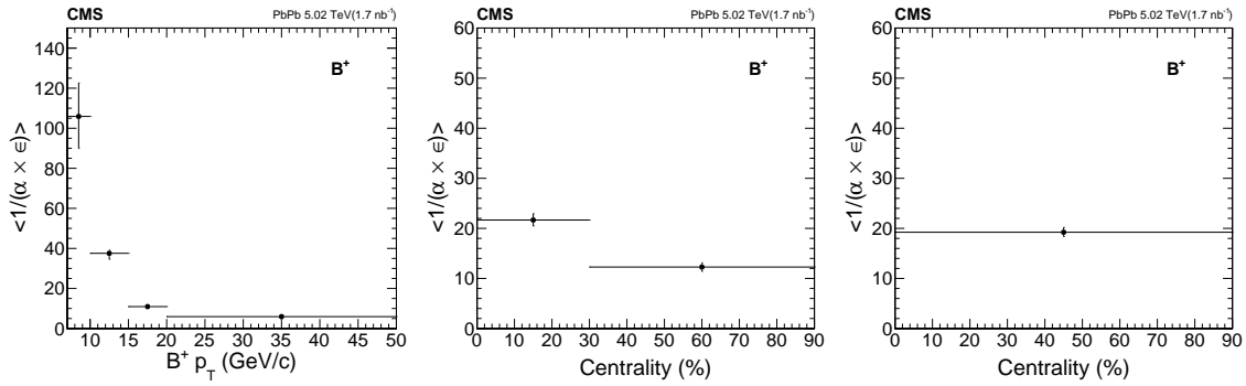
Figure 5-52: The B^+ efficiency correction factor \langle \frac{1}{\alpha \times \epsilon} \rangle vs p_T (left) and 0 – 30 % and 30 – 90% centrality (middle) and the inclusive 0 – 90% centrality (right) are shown above.
