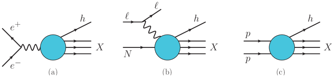
Figure 1-33: Single-inclusive hadron production process, where fragmentation function are involved, in (a) electron-positron annihilation, (b) deep-inelastic lepton-nucleon scattering, (c) proton-proton scattering, are shown above.
