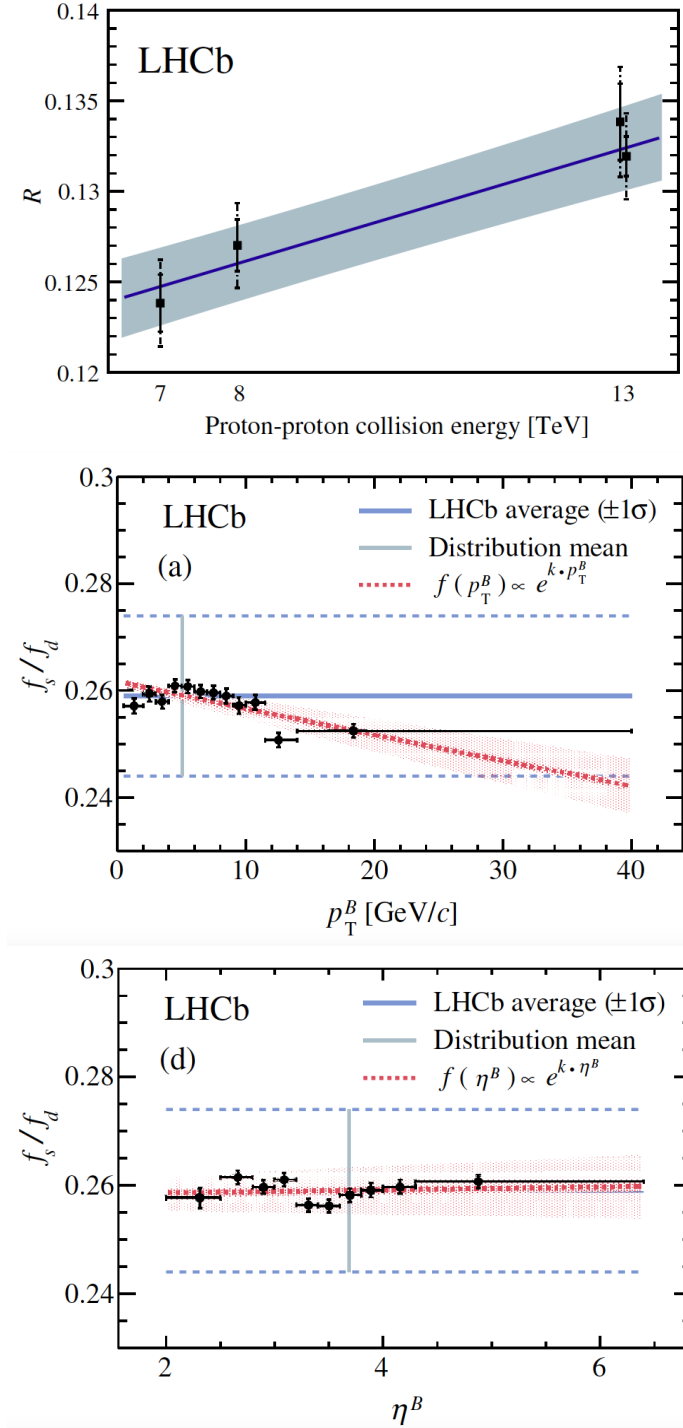
Figure 1-35: R , the corrected yield ratio of B_s^0/B^+ , as a function of the pp collision energy \sqrt{s} (top), the f_s/f_d ratio as a function p_T (middle), and the f_s/f_d ratio as a function \eta_B (bottom) from the LHCb experiment, are shown above.
