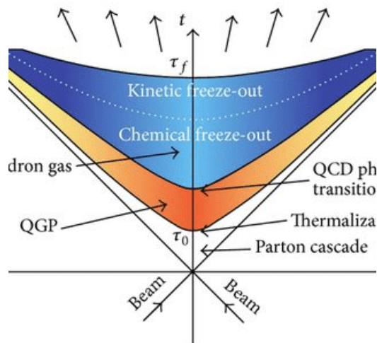
Figure 1-14: The space-time evolution diagram of heavy-ion collisions is shown above. It consists of five stages: initial state before the collisions, early stage of hard scattering processes, the hydrodynamic expansion of QGP, hadronization after QGP expands and cools down, and the freeze-out stage, first chemical freezeout when the particle species no longer change, and finally kinetic freezeout when the elastic scattering processes ceas.
