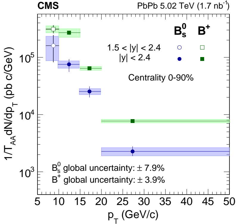
Figure 5-71: The measurement of B_s^0 and B^+ p_T differential cross section \frac{1}{T_{AA}} \frac{dN}{dp_T} as a function of B-meson p_T within 0 - 90% centrality is shown above. It should be pointed out that the cross section results are plotted in the unit of pb c/GeV since T_{AA} is in the unit of \text{pb}^{-1} while the p_T is in the unit of GeV/c. The open markers from 7 - 10 GeV/c stand for the fiducial measurement at the B-meson rapidity of 1.5 < |y| < 2.4 .
