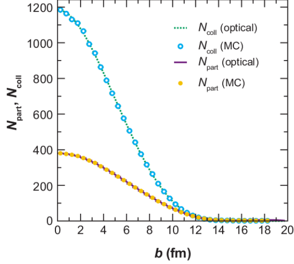
Figure 1-19: The N_{part} and N_{coll} as a function impact parameter calculated from the Glauber Model with optical approximation (lines) and from MC simulations (circles) are shown above. We can see they have an almost perfect agreement with each other.
