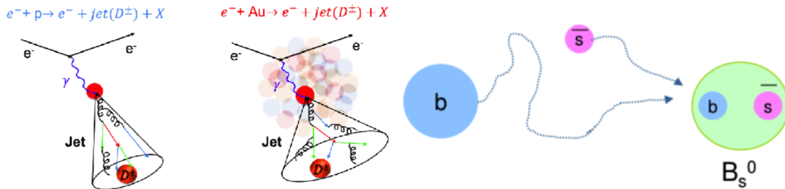
Figure 1-4: The fragmentation process of charms quarks hadronize into D^\pm (left) and the coalescence process of a beauty quark combining with a strange quark nearby to form a B_s^0 are shown above.
