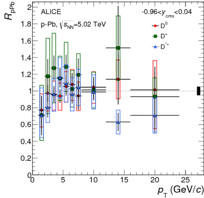
Figure 2-3: The R_{pA} as a function of p_T of prompt D mesons measured by the ALICE experiment is shown above.
