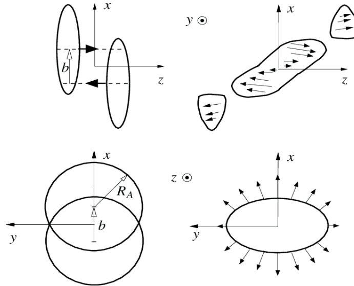
Figure 1-15: The definitions of impact parameter b in heavy-ion collisions, the overlapping interaction region, and the break-up remnants of the two nuclei, called spectators, moving along the z -direction are shown above. An almond shape of the nuclear interaction region, which results in the azimuthally anisotropic emission of final state particles, is seen in heavy-ion collisions.
