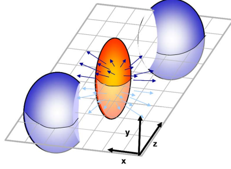
Figure 1-25: The figure above shows the ellipsoid of the overlapping nuclear reaction region of two nuclei in heavy-ion collisions. The reaction plane, which is the x - z plane shown above, is constructed by the beam direction and the impact parameter vector. The emission of particles is azimuthally anisotropic in the x - y plane due to the almond shape geometry.
