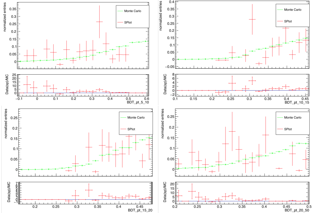
Figure 5-42: Comparison of B_s^0 BDT distribution in data (red) and MC (green) using the Splot method.
