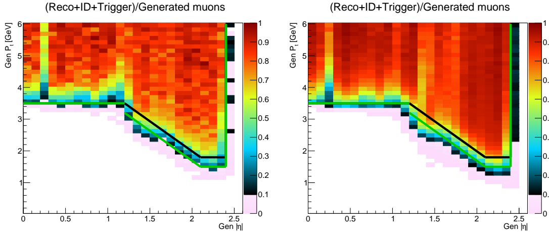
Figure 5-12: The total efficiency, including reconstruction, identification, and trigger, of a single muon in 2018 PbPb (left) and 2017 pp (right) are shown above. The black curve is the 2015 PbPb and pp 90% muon efficiency boundary while the green curve is the 2017 pp and 2018 PbPb 90% muon efficiency boundary. The green boundary is translated to numerical values in Table 5.4
