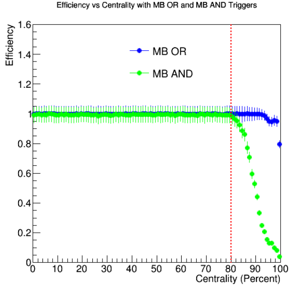
Figure 3-7: The efficiency vs centrality with ADC > 16 for MB OR (blue) and MB AND (green) are shown above.
