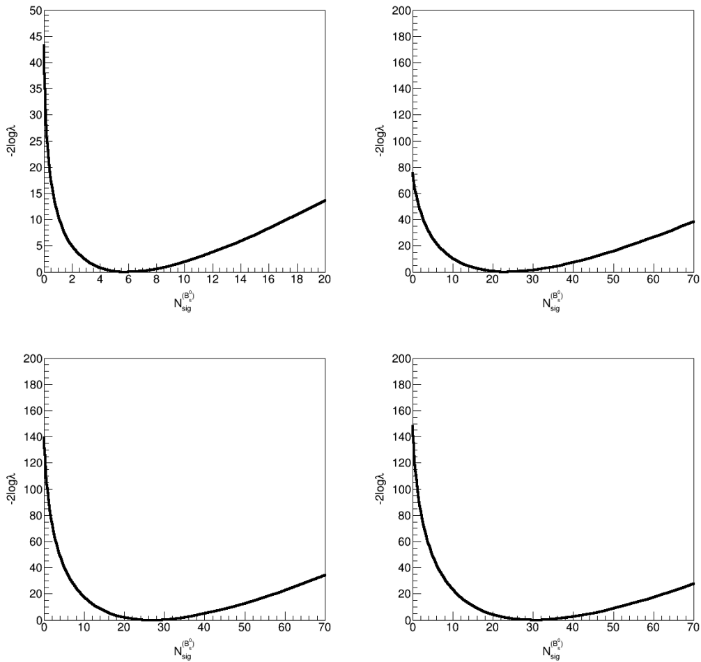
Figure 5-37: The significance vs signal yield for p_T bins at 7 – 10, 10 – 15, 15 – 20, and 20 – 50 GeV/c for 0 - 90% centrality are shown above
