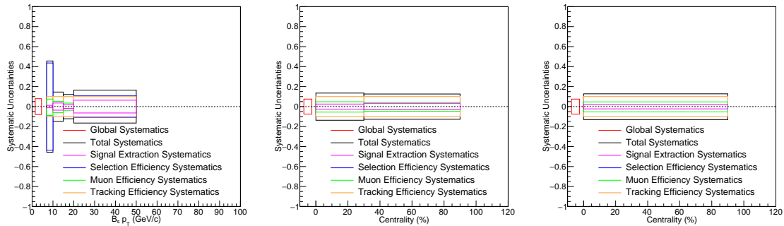
Figure 5-69: The summary of B_s^0 systematic uncertainties plotted as a function of p_T (left), centrality in 0 - 30%, and 30 - 90% (middle), and the inclusive centrality bin 0 - 90% (right) are shown above.
