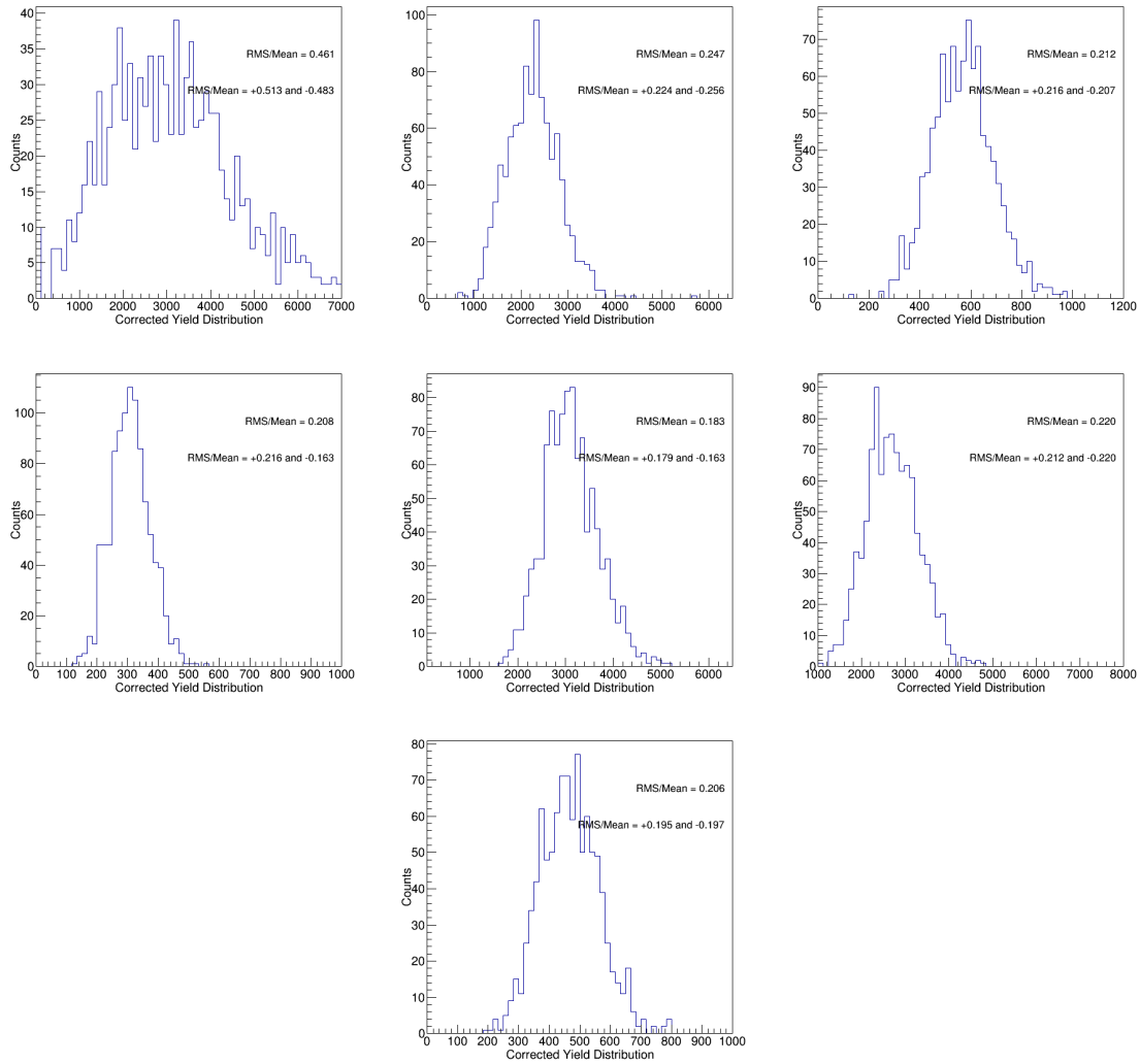
Figure 5-60: The B_s^0 corrected yield distributions of the 1000 data-like randomly resampled datasets for centrality in 0 - 90% in the p_T range of 7 - 10, 10 - 15, 15 - 20, and 20 - 50 GeV/c as well as 0 - 90%, 0 - 30%, and 30 - 90% in the p_T range of 10 - 50 GeV/c are shown above.
