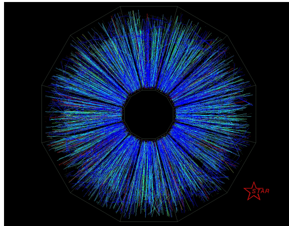
Figure 1-17: Two gold ions collide head-on in the STAR detector. The event with reconstructed tracks of final state particles is displayed by STAR TPC shown above. Image from [61]
