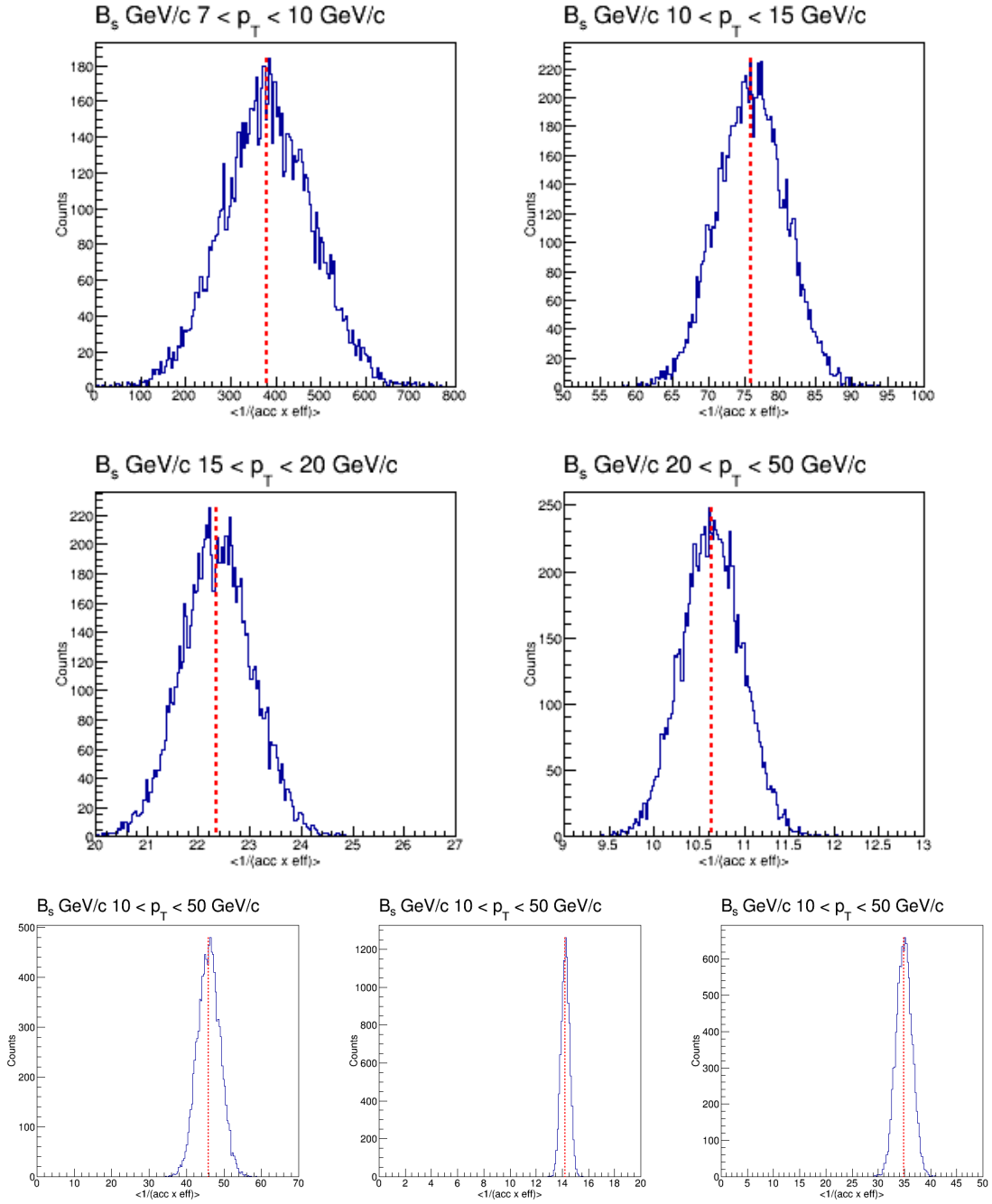
Figure 5-63: The distribution of B_s^0 \langle \frac{1}{\alpha \times \epsilon} \rangle for centrality in 0 - 90% in the p_T range of 7 - 10, 10 - 15, 15 - 20, and 20 - 50 GeV/c as well as 0 - 90%, 0 - 30%, and 30 - 90% in the p_T range of 10 - 50 GeV/c are shown above. The red dash lines are our nominal value for efficiency correction.
