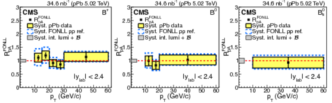
Figure 2-4: The R_{pA} as a function of p_T of B^+ , B^0 , and B_s^0 mesons measured by the CMS experiment is shown above.
