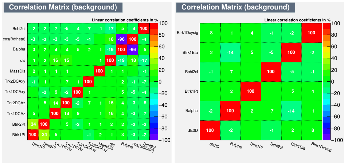
Figure 5-21: The correlation matrices of B_s^0 (left) and B^+ (right) in data at 10 < p_T < 15 GeV/c are shown above.
