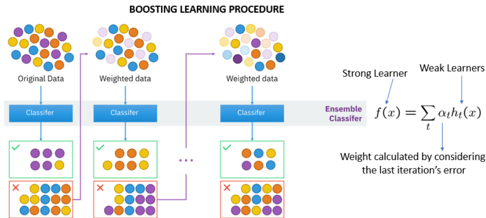
Figure 5-19: The schematic illustration of boosting procedures in machine learning is shown above.
