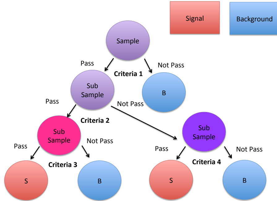
Figure 5-20: The schematic block diagram of a binary decision tree with N_{Tree} = 4 to separate signal and background in a training sample.
