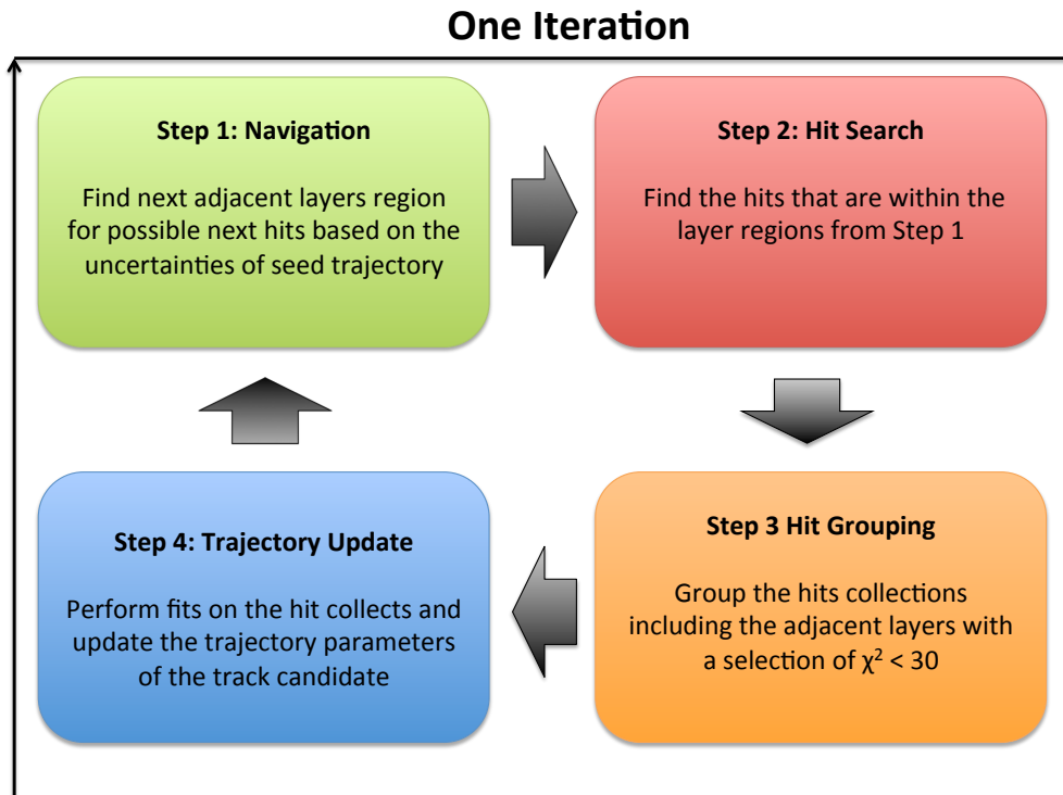
Figure 4-9: The four steps of CMS track finding workflow (left) and the schematic demonstration of each step (right) are shown above.
