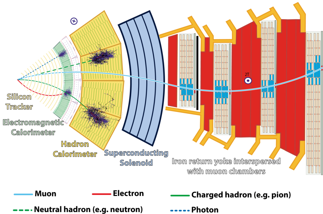
Figure 3-11: The particle flow of long-life particles, such as electrons, muons, photons, charged hadrons: \pi, K, p , and neutral hadrons: neutrons, in the CMS detector are shown above.
