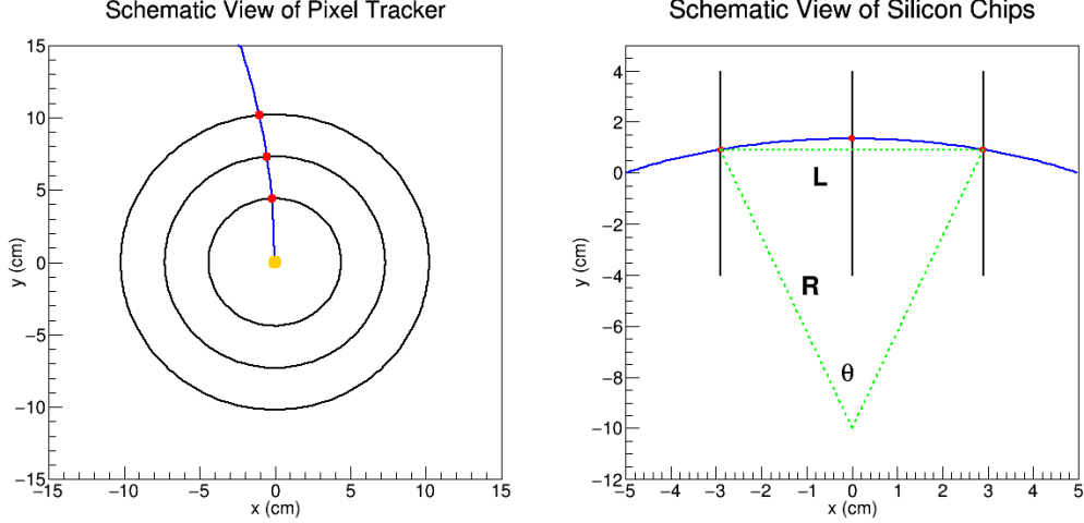
Figure 4-5: A track (blue) initiated from the beam spot (orange) passing through 3 layers of pixel detectors (black) with 3 clusters (red) is shown on the left and the circular fit to the 3 clusters with the definition of R , L , and \theta is shown on the right.
