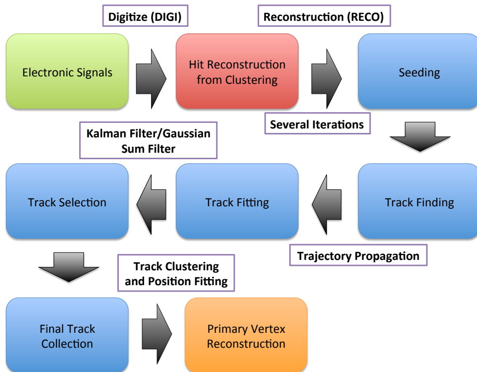
Figure 4-8: The schematic block diagram of CMS tracking workflow is shown above.
