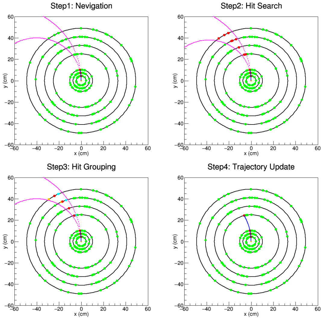
Figure 4-10: The four schematic plots demonstrating each of the four steps for track finding are shown respectively above.
