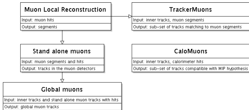
Figure 4-14: The relationship between different reconstructed muon in CMS is shown above
