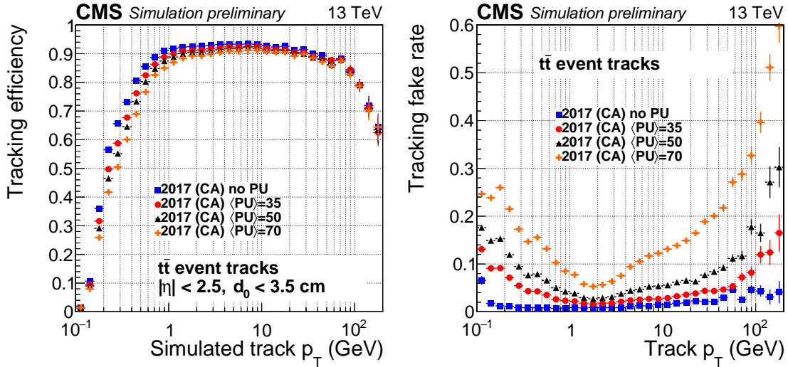
Figure 4-12: The CMS tracking efficiency (left) and fake rate (right) as a function of p_T from simulations of t\bar{t} events at 13 TeV with different pileup conditions are shown above.
