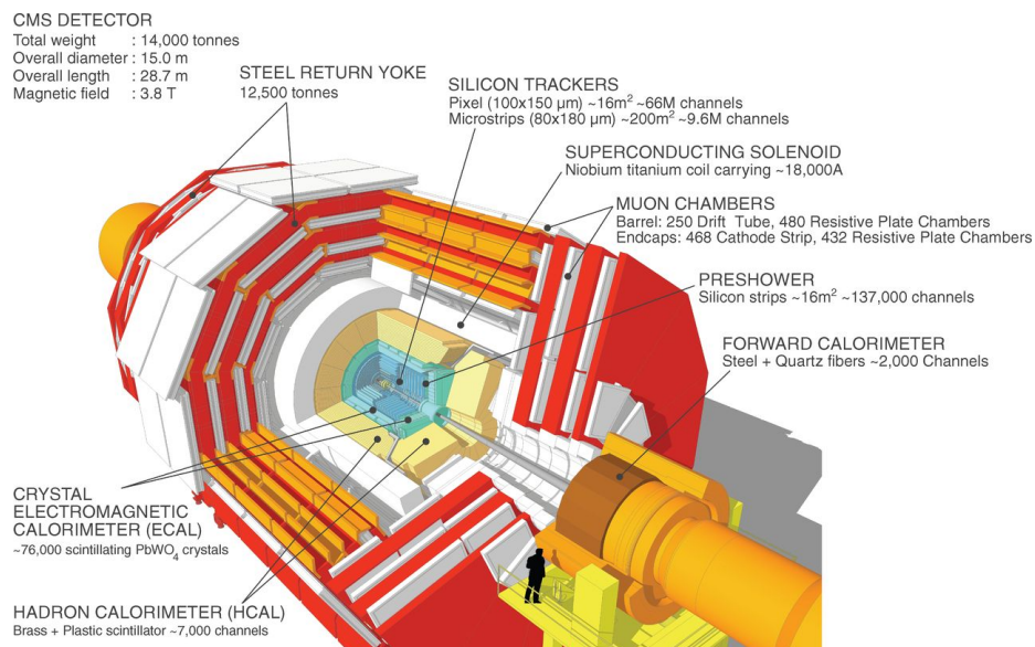
Figure 3-2: The schematic view of the CMS detector with brief descriptions of all its components is shown above. Image from [158]
