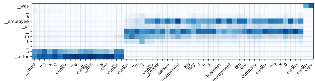
Span-level Supervision
