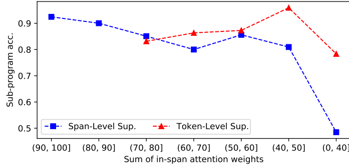
Figure 2: Sub-program prediction accuracy w.r.t. the sum of attention weights over oracle utterance spans. Models are trained on |\mathcal{C}_{\text{train}}| = 32 . Results averaged over three runs.
