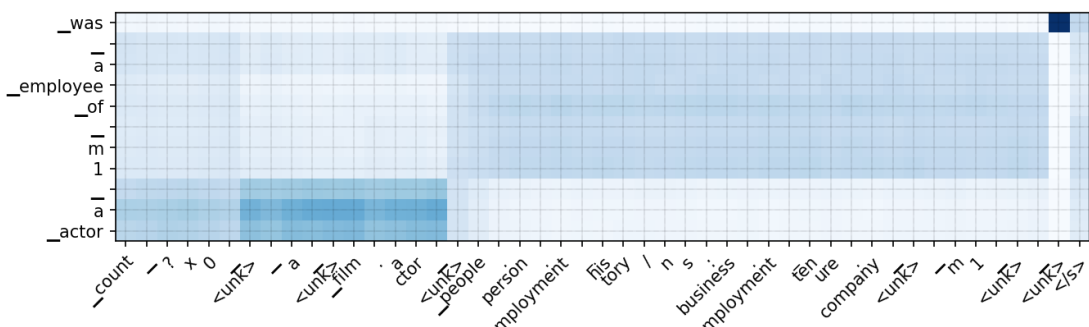
Span-level Supervision
