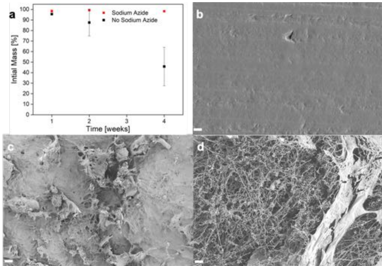
Figure 5.3. Silk film degradation with soil microbial activity vs no activity. A) Mass loss. Statistical significance across time ( p < 0.05 ) and across sodium azide presence ( p < 0.05 ). B) 6hr Annealed silk film T=0 C) No microbial activity T=4 weeks D) Microbial activity T=4 weeks. Scale bar 10 \mu\text{m} .
