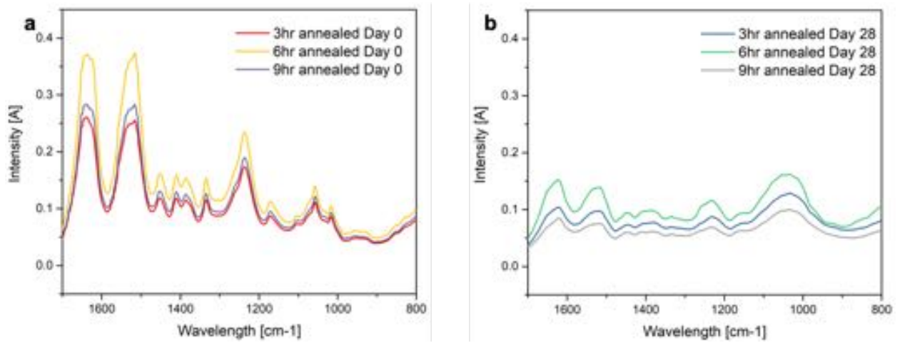
Supplement Figure 5.8. FTIR of degraded silk film week 4. A) Day 7 B) Day 28
