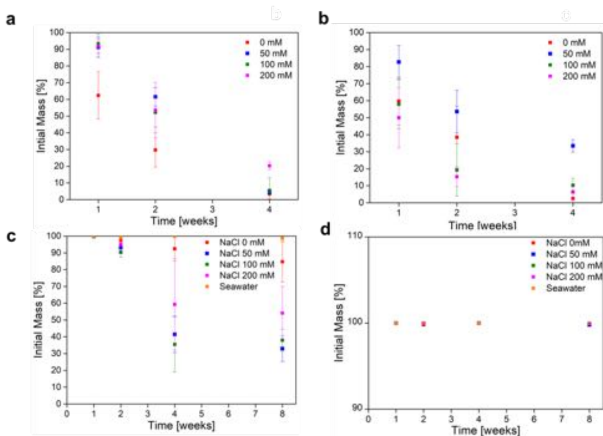
Figure 5.4. Silk film degradation profile in Soil and Solution. A) Soil with varying salinity with R. tropici embedded in films. No statistical significance between 50 mM and 100 mM; 50 mM and 200 mM; 100 mM and 200 mM but statistical significance between the rest of the samples ( p < 0.05 ). B) Soil with varying NaCl concentration with no R. tropici embedded in films. No statistical significance between 0 mM and 100 mM; 100 mM and 200 mM but statistical significance between the rest of the conditions ( p < 0.05 ). C) Solution with varying salinity with R. tropici embedded in films. Statistical significance across time ( p < 0.05 ) and NaCl solution concentration ( p < 0.05 ). D) Solution with varying salinity with no R. tropici embedded in films. No statistical significance across time and NaCl solution concentration.
