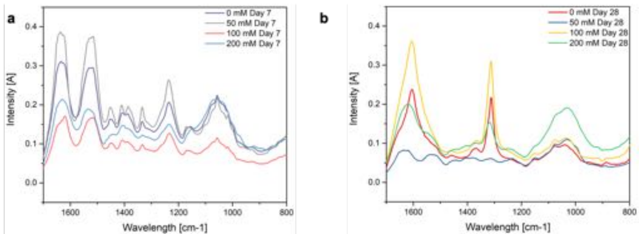
Supplement Figure 5.7. FTIR of degraded silk film in soil of varying salinity. A) Day 7 B) Day 28
