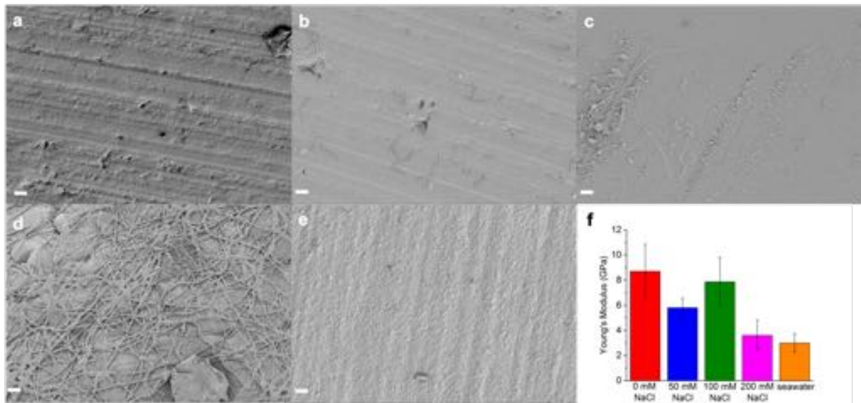
Supplement Figure 5.4. SEM of silk film degradation profile in solution with no R.tropici week 8. A) 0 mM NaCl B) 50 mM NaCl C) 100 mM NaCl D) 200 mM NaCl E) Sea water. Scale 10 \mu\text{m} F) Young's modulus (Nano-indentation). Statistical significance across all conditions ( p < 0.05 ).
