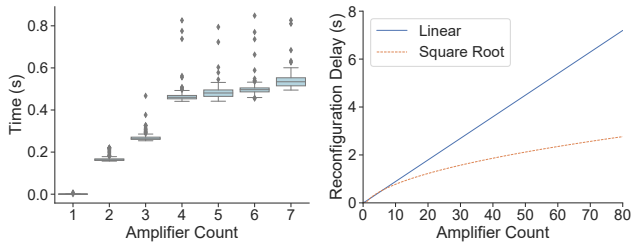
(a) We collect 100 measurements for each set of amplifiers using SNMP. (b) Linear (solid) and square-root (dotted) regression models.
