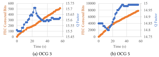
Figure 6: QoT measurements for witness waves while adding/dropping OCG1. During the add/drop, Q factor for the witness waves is relatively constant—varying by +/- 0.1. Errors accumulate at a linear rate as expected in a live transport network; 100% are corrected with FEC while running traffic over OCGs 3 and 5.
