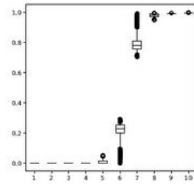
Flip from horizontal 1 million steps
