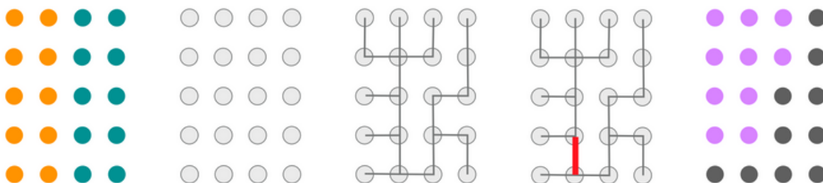
Figure 5. A schematic of a ReCom spanning tree step for a small grid with k = 2 districts that are merged ( l = 2 ) and resplit. Deleting the indicated edge from the spanning tree leaves two connected components with an equal number of nodes.
