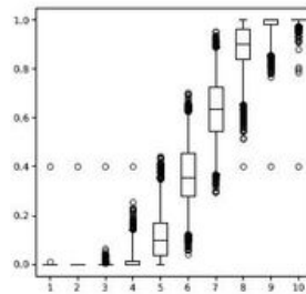
ReCom from vertical 20,000 steps
