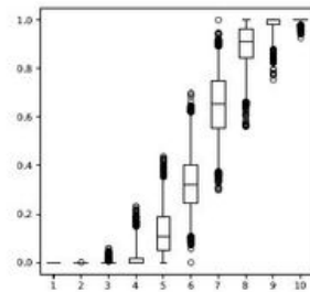
ReCom from horizontal 20,000 steps
