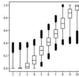
Flip from vertical 1 billion steps
