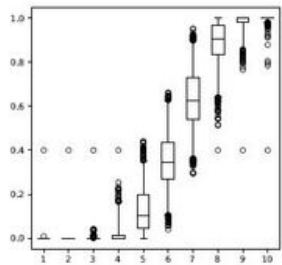
ReCom from vertical 10,000 steps
