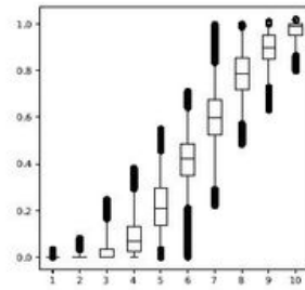
Flip from horizontal 1 billion steps
