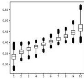
Flip from vertical 1 million steps
