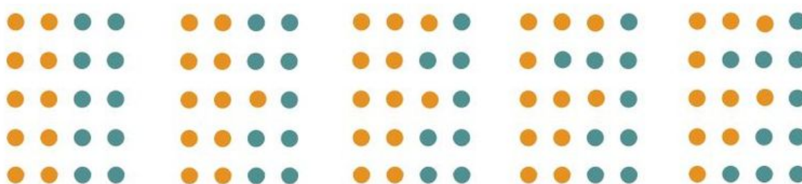
(A) Sequence of four flip steps
