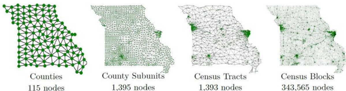
Figure 7. Four dual graphs for Missouri at different levels of geography in the census hierarchy.
