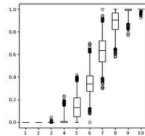
ReCom from horizontal 10,000 steps
