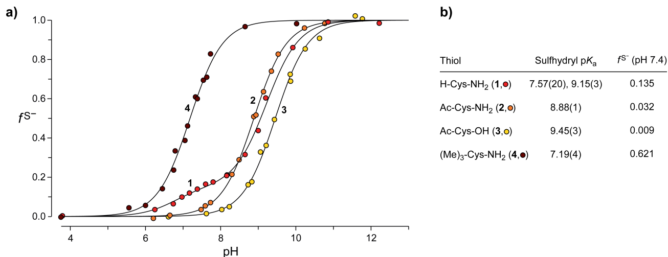
Figure 2. Determination of sulfhydryl pK_a values by UV titration monitoring A_{238} relative to A_{238} of the buffer containing no thiol. a) Fraction thiolate ( fS^- ), calculated as a function of pH. Data were fitted to a single titration model (thiols 2–4) or to a titration model accounting for microscopic pK_a values (thiol 1) (Equation S1). b) Table of measured sulfhydryl pK_a and calculated fS^- (pH 7.4) values.
