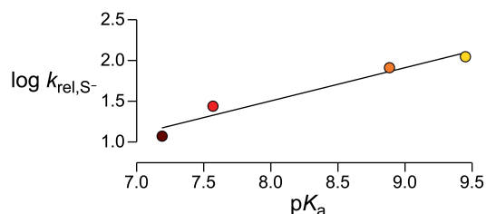
Figure 3. Brønsted plot of \log(k_{\text{rel,S}^-}) against pK_a , yielding \beta_{\text{nuc}} = 0.41(7) . For thiol 1 , pK_a^{SH,1} was used for plotting. Thiolate concentration-independent relative rate constants k_{\text{rel,S}^-} were determined using Equation S4.
