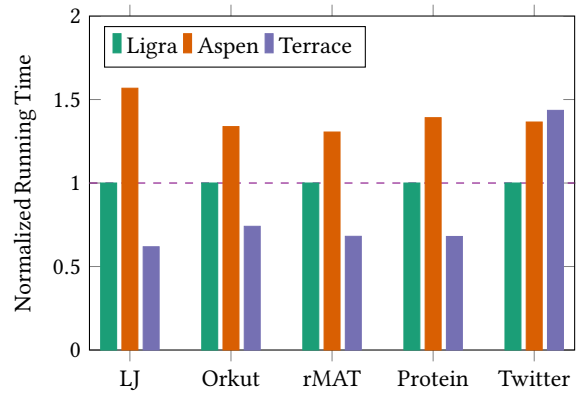
Figure 7: Time to run BFS normalized to Ligra.
