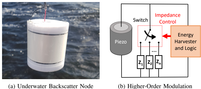
Fig. 1. PAB-QAM . (a) shows one of our potted PAB-QAM transducers (b) shows the schematic design for PAB-QAM .
