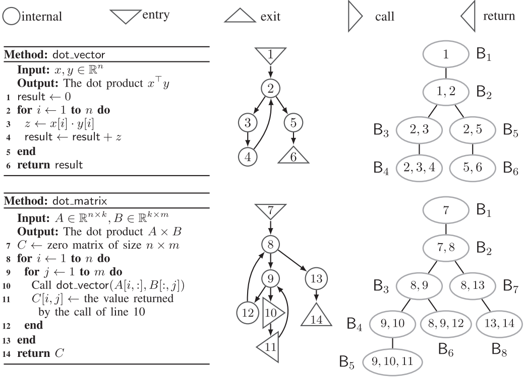
Fig. 3. Example of a program consisting of two methods: their control flow graphs G_i = (V_i, E'_i) where nodes correspond to line numbers, and the corresponding tree decompositions, each one achieving treewidth 2.
