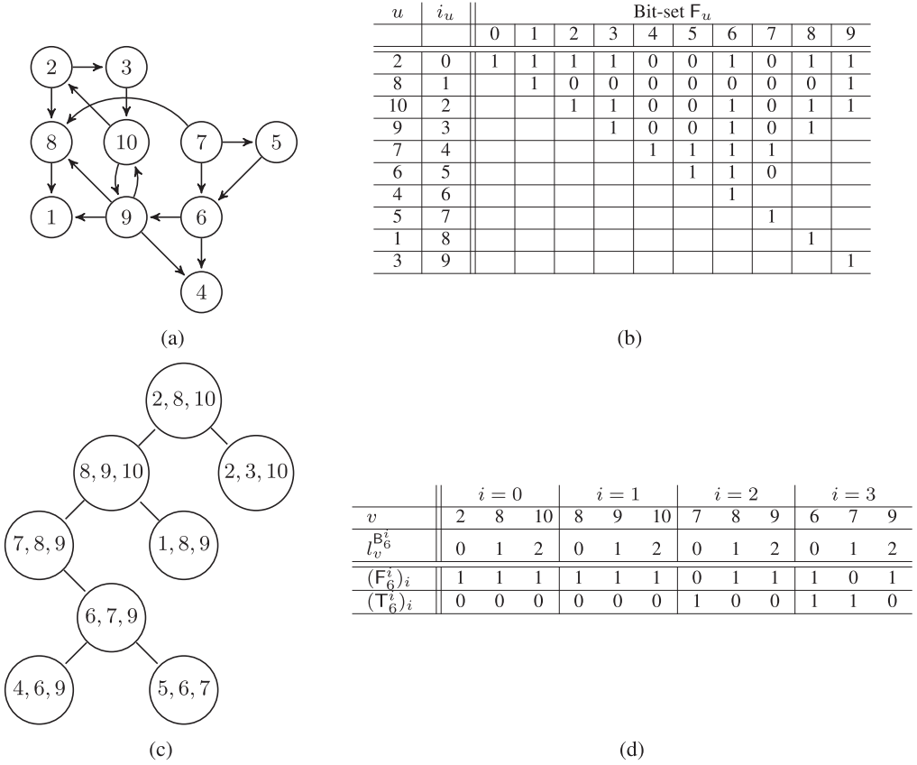
Fig. 6. (a), (c): A graph G and a tree-decomposition T = (V_T, E_T) of G . (b): The sets F_u constructed from step 5 to answer single-source queries. The j th bit of a set F_u is 1 iff (u, v) \in E^* , where v is such that i_v - i_u = j . (d): The set sequences (F_6^i)_i and (T_6^i)_i constructed from step 6 to answer pair queries, for u = 6 . For every i \in \{0, 1, 2, 3\} and ancestor B_6^i of B_6 at level i , every node v \in B_6^i is assigned a local index l_v^{B_6^i} . The j th bit of set F_6^i (respectively, T_6^i ) is 1 iff (6, v) \in E^* (respectively, (v, 6) \in E^* ), where v is such that i_v^{B_6^i} = j .
