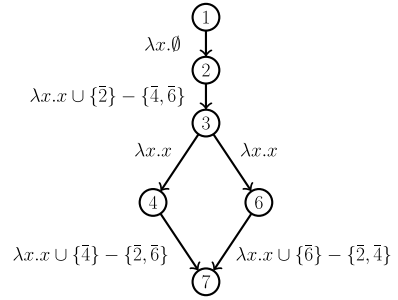
Fig. 8. An example program (left) and its reaching definitions analysis in IFDS (right).
