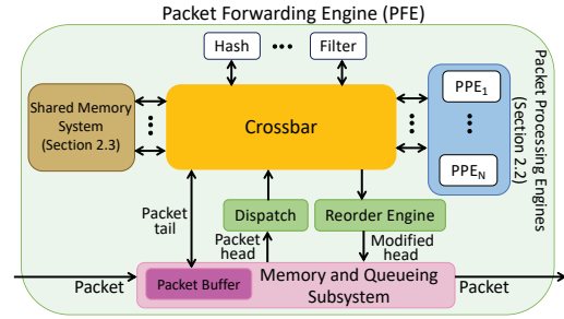
Figure 2: Trio’s Packet Forwarding Engine (PFE) architecture. Each PFE has hundreds of multi-threaded Packet Processing Engines (PPEs).
