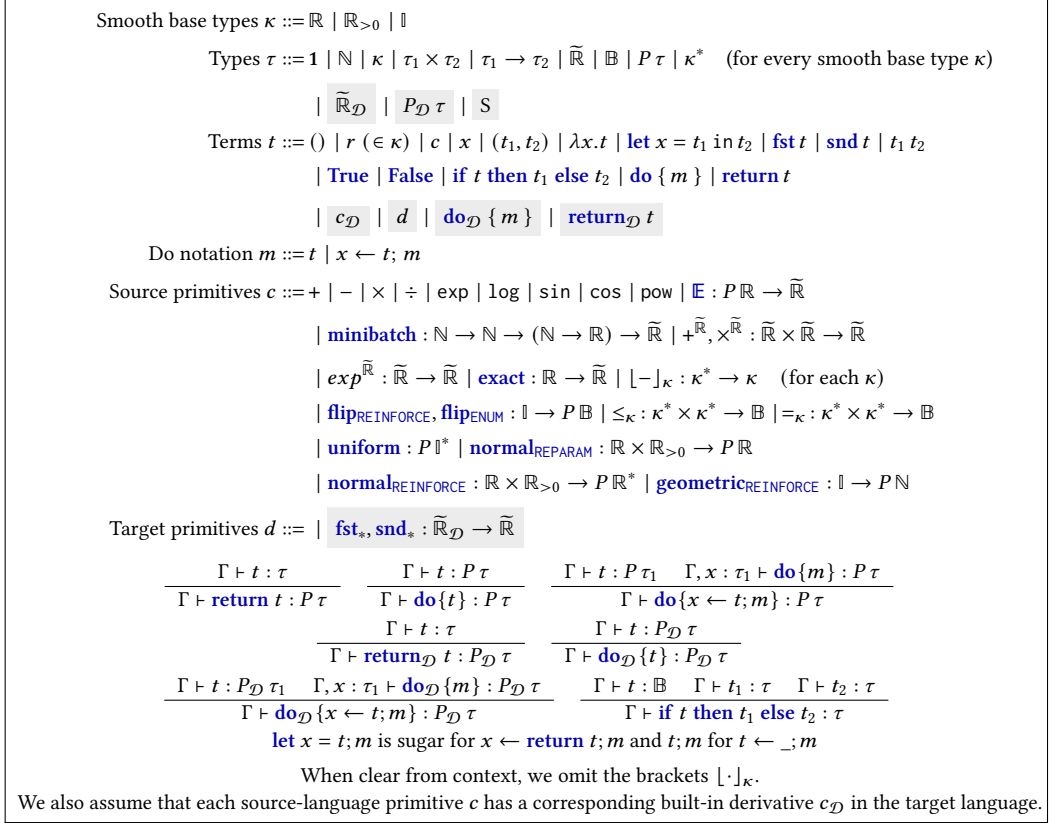
Fig. 22. Full grammar and selected typing rules of the language we study. Gray highlights indicate syntax only present in the target language of the AD macro.
