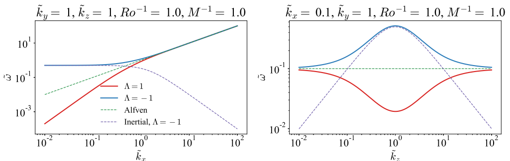
FIGURE 7. The dispersion relation for waves in the B\Omega -MHD system, in the case where \mathbf{B}_0 = B_0\hat{\mathbf{x}} and \boldsymbol{\Omega} = \Omega\hat{\mathbf{z}} (equation (A3)). The green dashed line shows the Alfvén wave dispersion relation, and the purple dashed line shows that of an inertial wave. The low frequency branch with \Lambda = 1 is similar to the magnetostrophic mode in the case when \mathbf{B}_0 and \boldsymbol{\Omega} are aligned (Galtier 2014).
