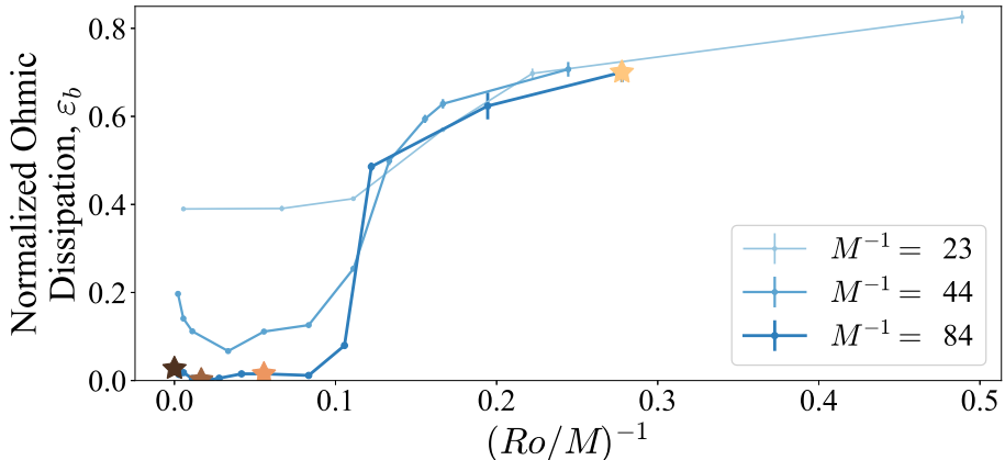
FIGURE 6. Normalized Ohmic dissipation, \varepsilon_b , versus (Ro/M)^{-1} . The Ohmic dissipation represents a measure of how active the induced magnetic field is in the dynamics. We see that, for three values of M^{-1} , the induced magnetic field begins to dominate the dynamics once (Ro/M)^{-1} > 0.1 , in other words when Ro^{-1} > 0.1M^{-1} . (Ro/M)^{-1} is also referred to as the Lehnert number (Lehnert 1955). Stars represent runs whose snapshots are shown in Figure 1.
