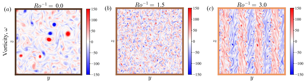
FIGURE 4. Snapshots of the out-of-plane vorticity, \omega = \hat{x} \cdot (\nabla \times \mathbf{v}) = -\nabla_{\perp}^2 \psi , for the 2D3C rotating simulations, representing, from left to right, Regimes I (a), II (b), and III (c), as rotation is increased. We see striking similarities to Figure 1, confirming that the asymptotic 2D3C model captures the different regimes found in the 3D simulations of section 3.
