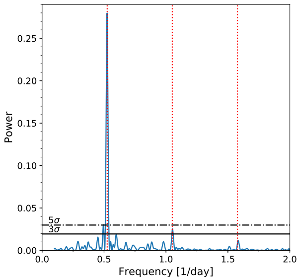
Figure 2. Lomb–Scargle periodogram of the detrended TESS PDCSAP light curve of TOI-1518, with the transits and secondary eclipses removed. Significance thresholds are indicated by the horizontal lines. The red vertical lines denote the first three harmonics of the orbital period. There are clear signals at the orbital frequency and at the first harmonic, corresponding to the planetary atmospheric brightness modulation and stellar ellipsoidal distortion, respectively.
