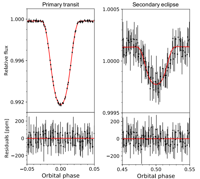
Figure 4. Zoomed-in views of the primary transit (left) and secondary eclipse (right) of TOI-1518b. The light curves are binned in 3-minute intervals. Note the difference in vertical scale between the two plots. The difference in out-of-occultation baselines primarily reflects the planetary phase-curve modulation. The bottom panels show the corresponding residuals from the best-fit model.
