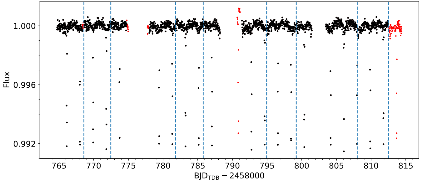
Figure 1. The normalized Presearch Data Conditioning Simple Aperture Photometry (PDCSAP) light curve of TOI-1518 generated by the SPOC pipeline. The scheduled momentum dumps are indicated by the vertical blue dashed lines. The red points denote flux ramps and regions of severe systematics that were trimmed prior to our light curve fits. The orbital phase curve modulations are discernible in the raw photometry.
