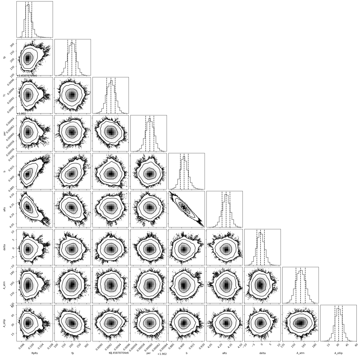
Figure 10. Corner plot of parameters involved in the joint TESS and ground-based light-curve fit.
