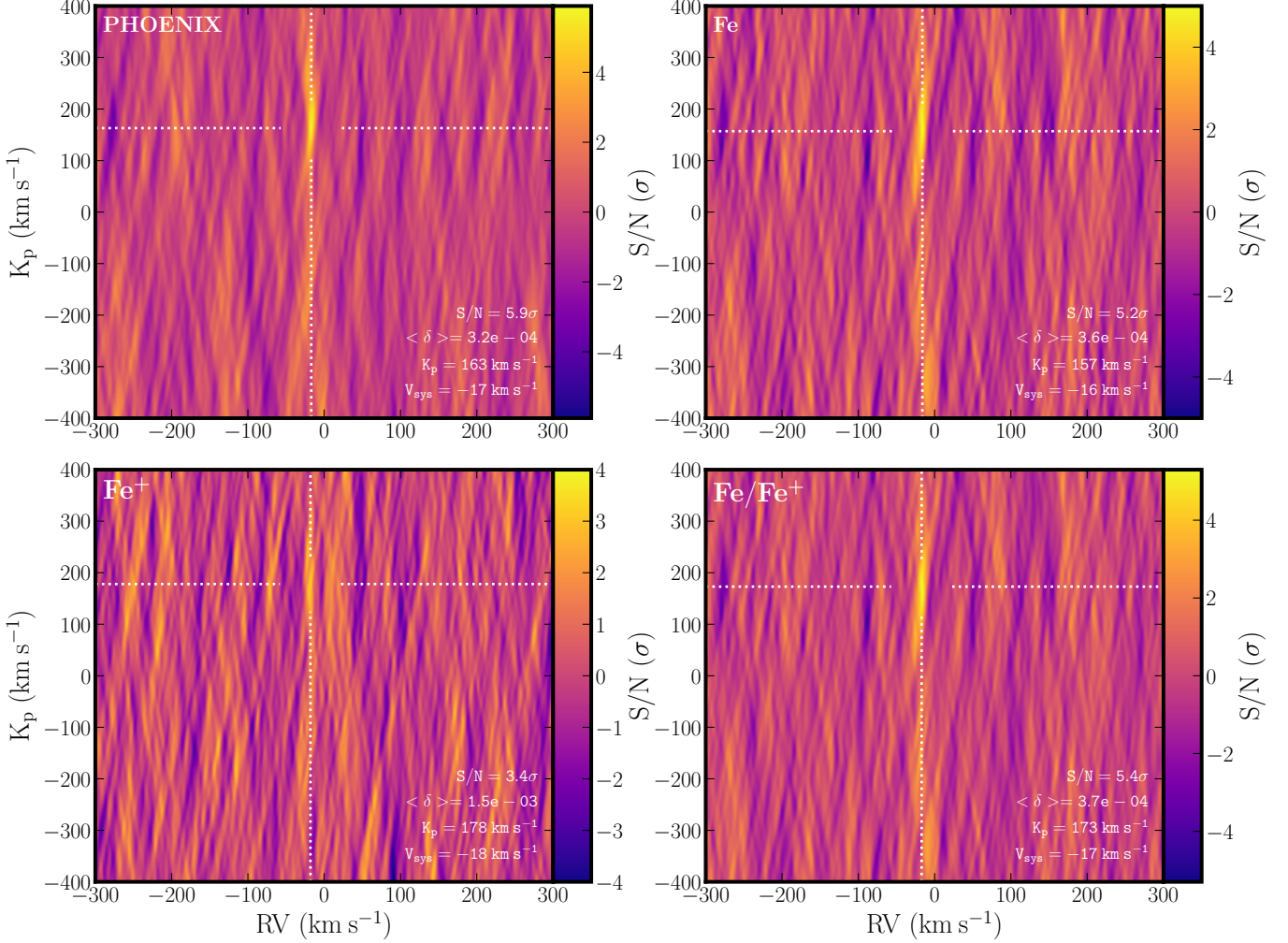
Figure 9. Atmospheric detections in TOI-1518b and their K_p - V_{\text{sys}} maps. The top-left corner of each panel indicates the cross-correlation template, and the bottom right corner lists properties of the peak value, including S/N of the detection, the average absorption depth after co-adding CCF rows ( \langle \delta \rangle ), and the maximal value of K_p , and V_{\text{sys}} . In all panels the Doppler shadow has been corrected per the methods in Section 3.2. For reference, we show results from cross-correlation with the PHOENIX spectrum used to model the Doppler shadow, revealing there are species common to both the planet’s atmosphere and star. The subsequent panels show results from cross-correlating with templates containing Fe and \text{Fe}^+ . In each panel, the white dotted lines indicate the K_p and V_{\text{sys}} with the highest signal.
