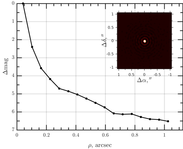
Figure 5. SPP 5\sigma contrast curve for TOI-1518 with autocorrelation function (ACF) inset. The observations were obtained at \lambda_c = 880 nm (FWHM=70 nm).
