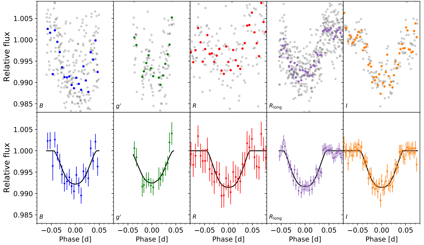
Figure 11. Ground-based light curves of TOI-1518 with full coverage of the primary transits, collected as part of the TESS Follow-up Program. Top: the photometry at the native time resolution (gray points) and binned (colored points). Each panel is labeled by the respective bandpass. The binning interval for the B -, g' -, and R -band observations is 7 minutes; a shorter 4-minute bin size is used for the higher-precision R_{\text{long}} - and I -band transits. Bottom: binned, systematics-corrected light curves, with the best-fit transit model from the joint TESS and ground-based photometric fit (Table 1) plotted in black.
