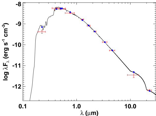
Figure 6. Spectral energy distribution of TOI-1518. Red symbols represent the observed photometric measurements, where the horizontal bars represent the effective width of the passband. Blue symbols are the model fluxes from the best-fit Kurucz atmosphere model (black).
