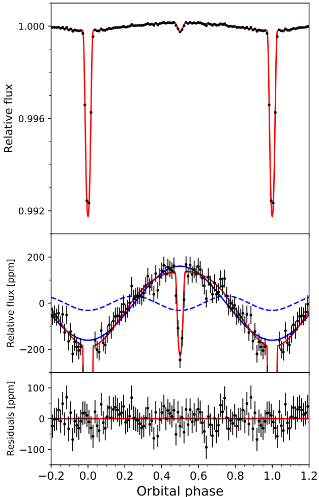
Figure 3. Top panel: systematics-corrected and phase-folded TESS light curve of TOI-1518, binned in 30-minute intervals, with the best-fit phase-curve model plotted in red. Middle panel: zoomed-in view of the phase-curve modulations and secondary eclipse. The atmospheric brightness modulation and ellipsoidal distortion signals are plotted separately in the solid and dashed blue lines. Bottom panel: corresponding residuals from the best-fit model.
