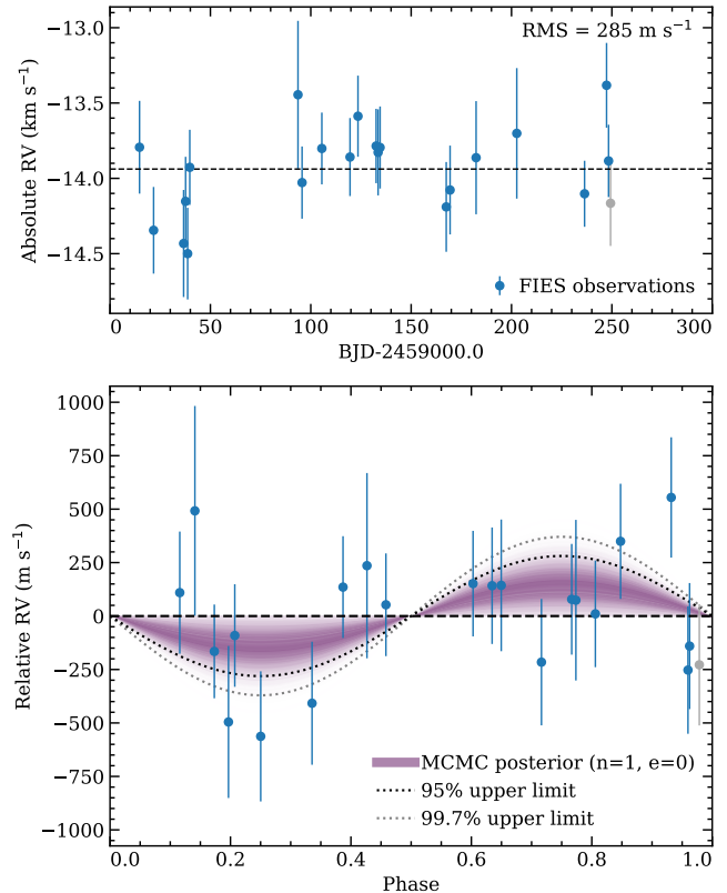
Figure 7. Out-of-transit RVs measured with FIES. Upper panel shows the full RV time series. Lower panel shows the same RVs phase-folded from T_c with the known orbital period. The K_s posterior distribution is visualized as shaded, purple curves in the background (darker: higher density). The last observation (gray) overlaps with the transit and has therefore been excluded from the fit. While the data have large uncertainties, the amplitude of the velocity variation is consistent with a planetary companion of M_p < 2.3 M_J .
