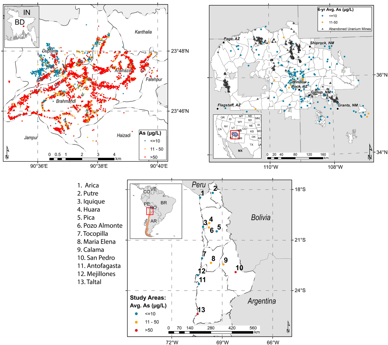
Fig. 2. Map showing the distribution of As sources for the three study populations in (a) rural Bangladesh, (b) Navajo Nation, and (c) Northern Chile. Note that WAS concentrations for the Northern Chile study are assigned to entire municipalities. Precise locations of PWS points in the NBCS map are obscured using a geo-masking algorithm.
