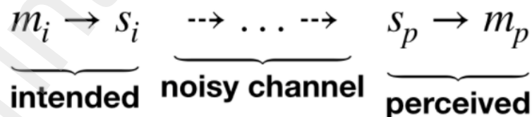
Figure 1: Schematic representation of the noisy channel model
