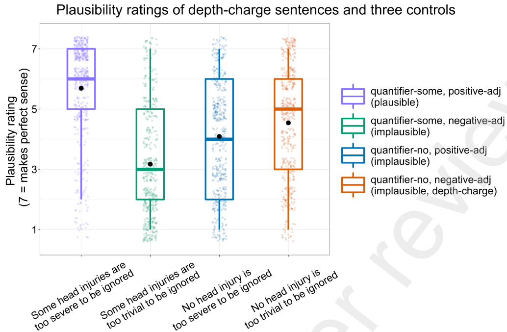
Figure 2: Plausibility ratings for sentences by condition in Exp.1. The depth-charge sentences were rated more plausible than the other implausible conditions. (the middle horizontal line in the boxplot represents the median; the black dot represents the mean; the jittered points represent single trial plausibility ratings)
