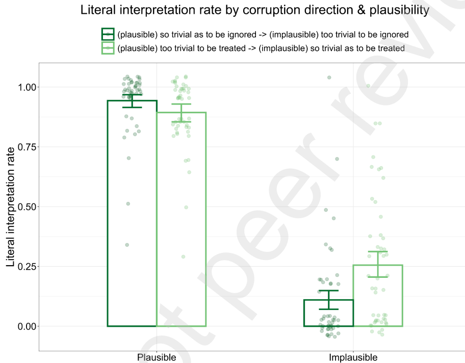
Figure 7: The literal interpretation rate of plausible and implausible sentences crossing the noise corruption direction and structure (error bars indicate 95% bootstrapped confidence interval; the points indicate average literal interpretation rate by subject)
