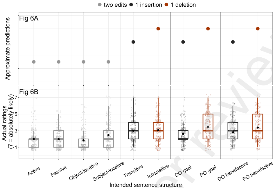
Approximate predictions vs. actual ratings of noise likelihood for Gibson et al. (2013) material
