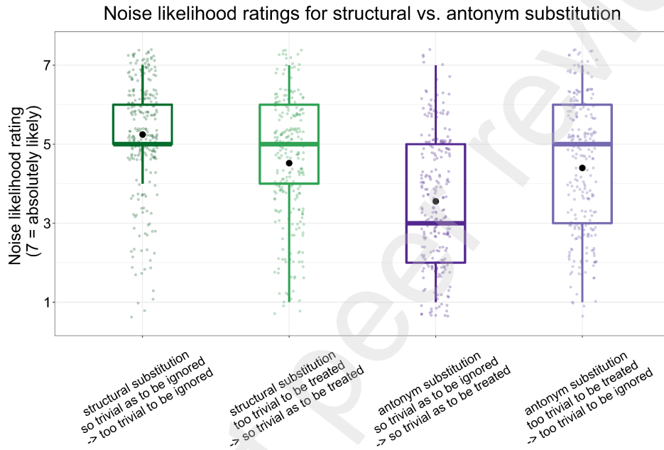
Figure 5: Noise likelihood ratings for the depth-charge material crossing types of noise corruption and intended structure (black points are mean; horizontal lines are median, with dots representing individual trials)
