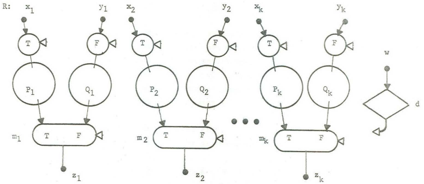
(a) Conditional schema.
