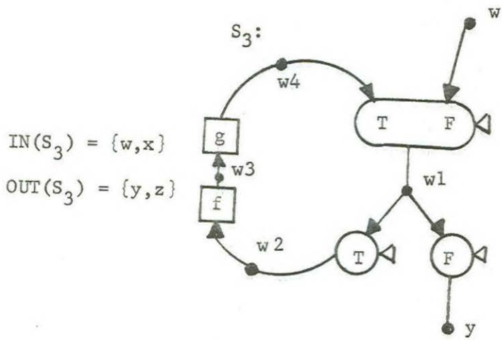
(c) Iteration Schema
