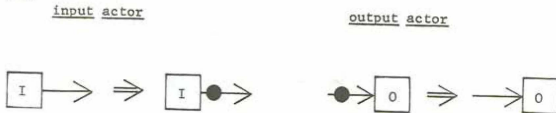
Figure 2.3 (continued) Firing rules
