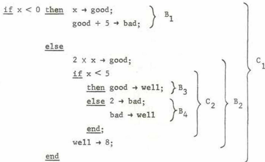
Figure 2.14 An example for the single assignment rule
