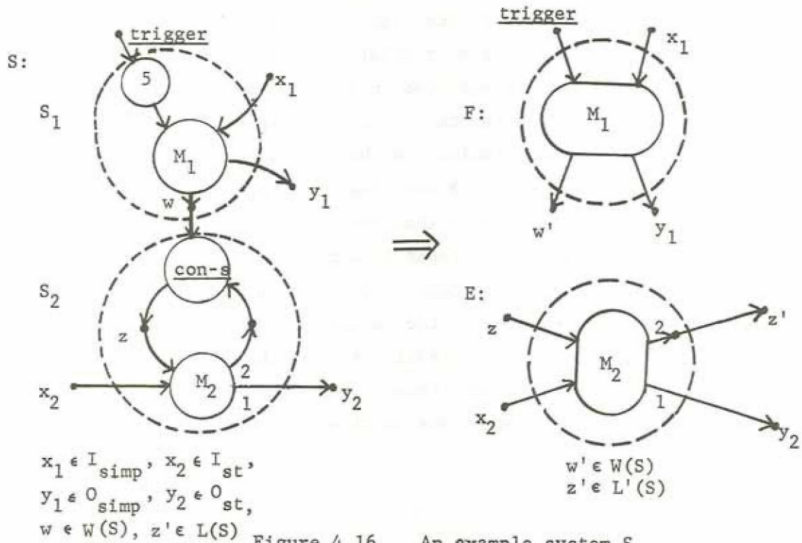
Figure 4.16 An example system S
