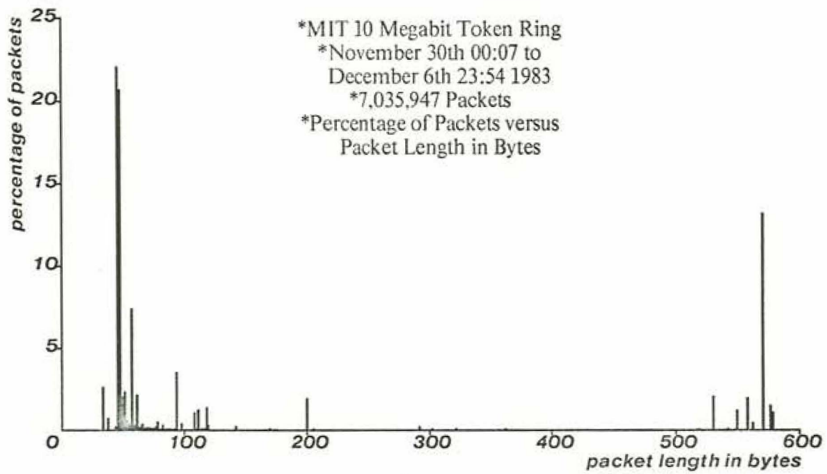
Figure 4-2:Percentage of Packets versus Packet Length
