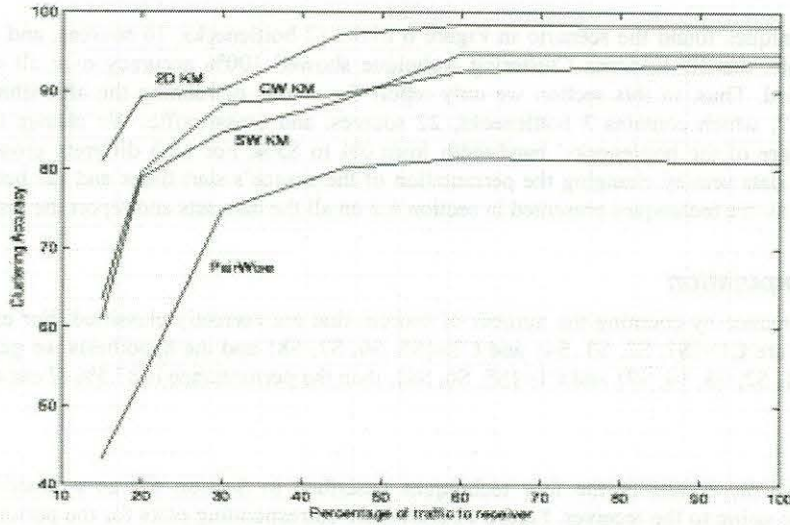
Figure 12: Performance Results PairWise: Iterative PairWise; CW: Cluster-Weighted KMeans; SW: Sample-Weighted KMeans, 2D KM: 2Dimensional Cluster-Weighted KMeans
