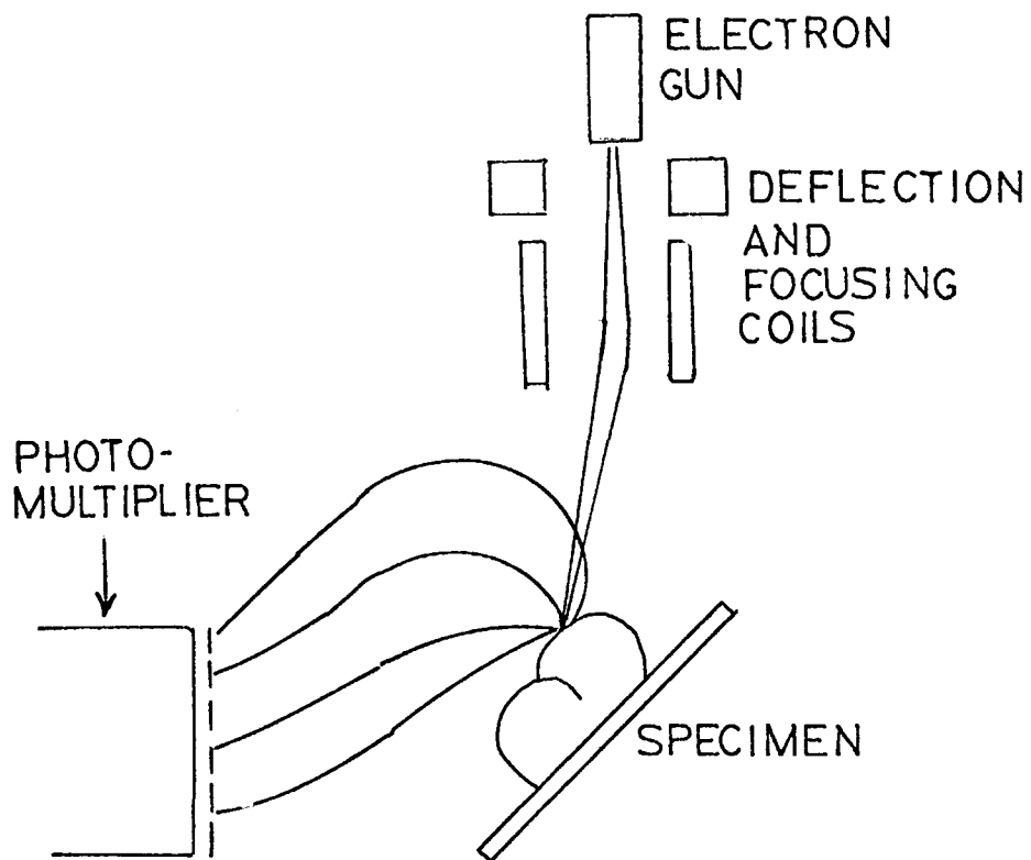
Figure 21: Sketch of a scanning electron microscope.
