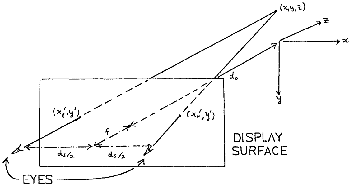
Figure 28: Stereo-projection of an object point.
