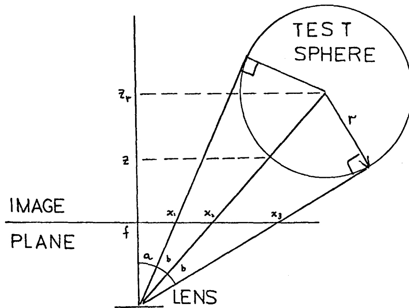
Figure 30 : Determining the exact position of the calibration sphere.
