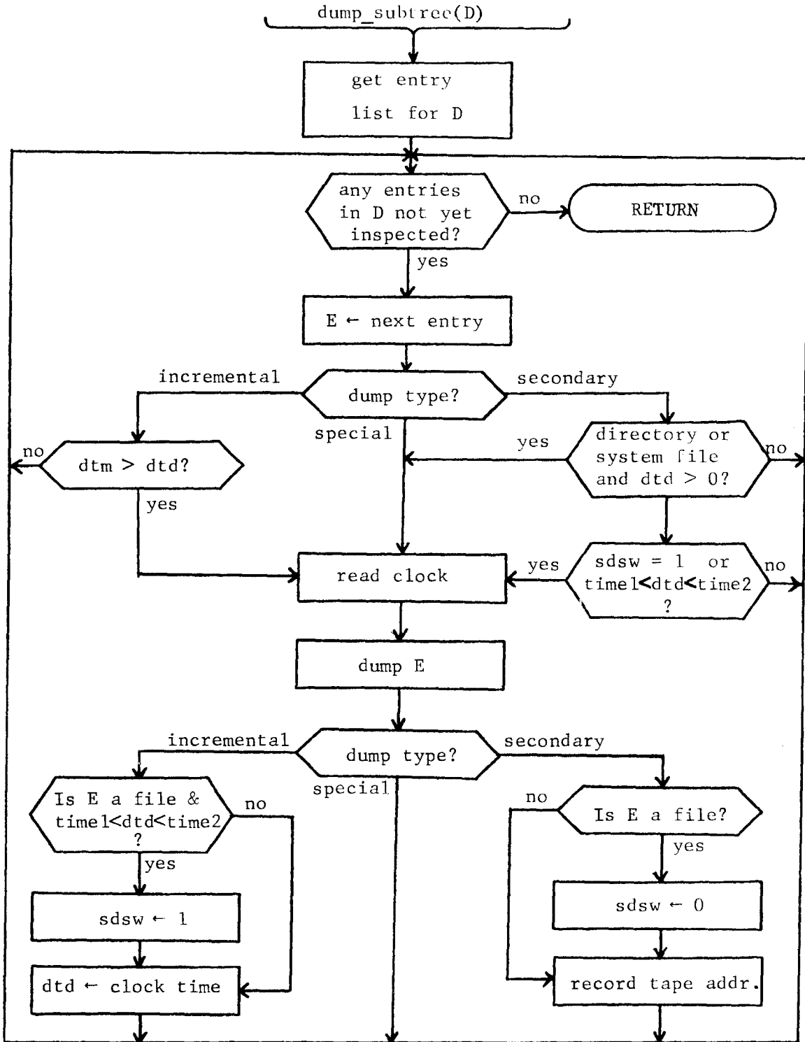
Figure 3.3: The incremental and secondary dumper algorithm (part 2).
