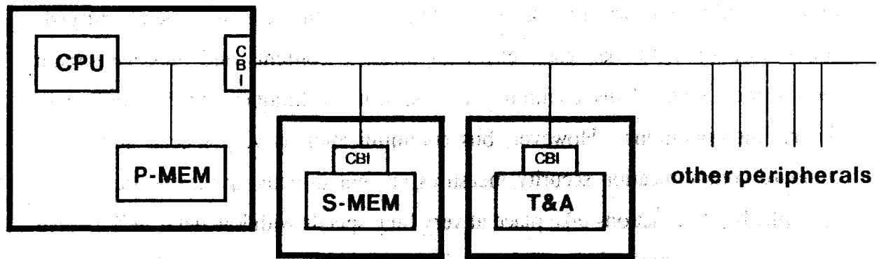
Figure 1-2: An Encrypted Bus Approach System Configuration
