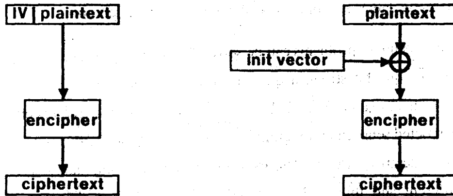
Figure 2-10: In-block and Additive Initialization Vector Techniques
