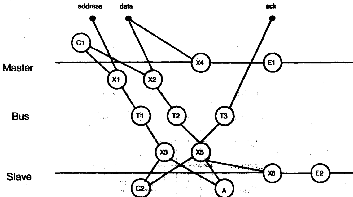
Figure 3-14: Event Graph for an aggregate secure write
