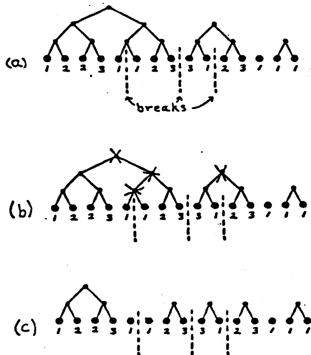
Figure 3. An illustration of the procedure described in Lemma 9.
