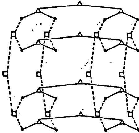
Figure 11. The 4 \times 4 mesh of trees M_{2,4} .
