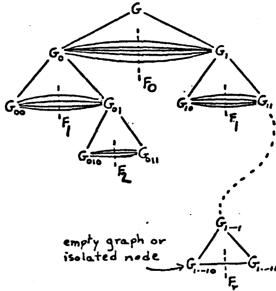
Figure 4. An (F_0, F_1, \dots, F_r) -decomposition tree.
