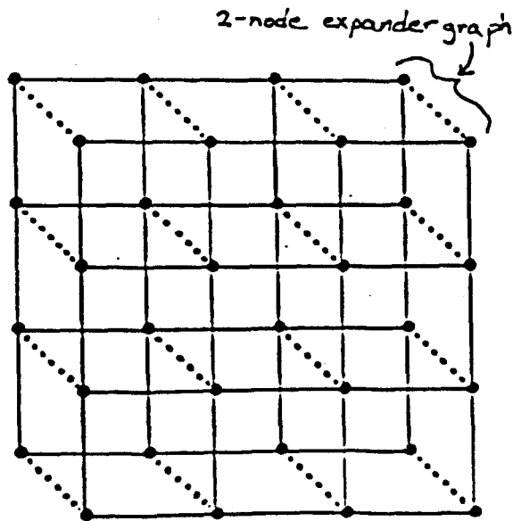
Figure 10. The expander-connected mesh P_{2,4} .
