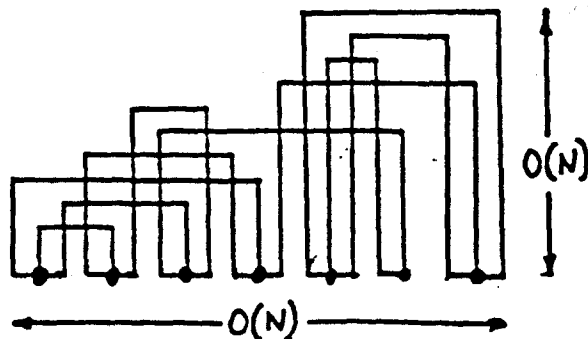
Figure 2. Every N -node graph can be laid out in O(N^2) area.
