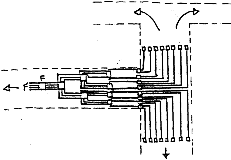
Figure 8. An improved layout for the tree of meshes.
