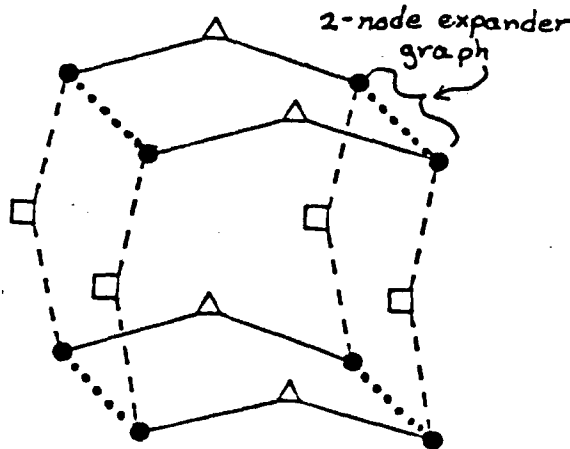
Figure 12. The expander-connected mesh of trees Q_{2,2} .
