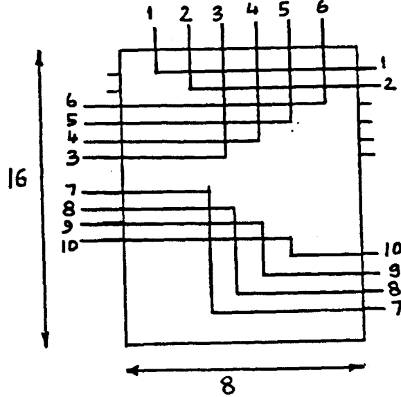
Figure 6. Using a mesh in the tree of meshes as a crossbar switch.
