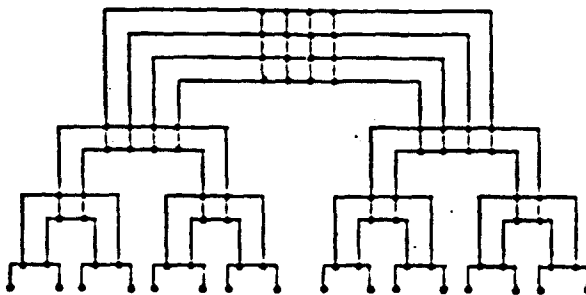
Figure 5. The 4 \times 4 tree of meshes T_4 .
