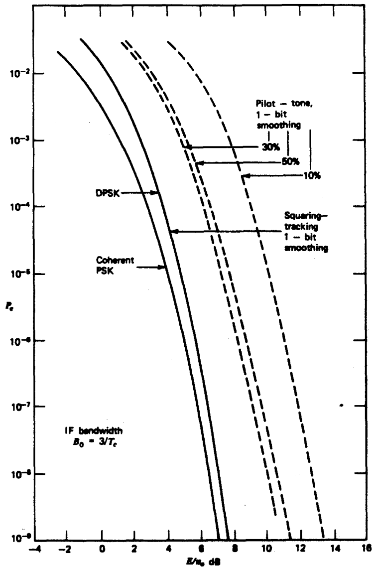
Figure 3-6: Error Rates for Several Modulation Systems (from [27])
