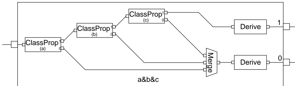
Figure 5-15: Compound module for computing A and B
