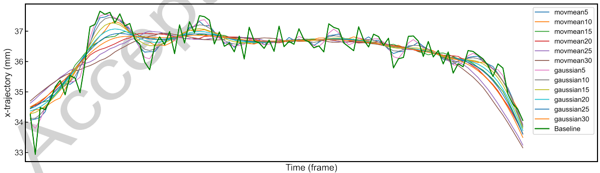
Fig. 7 Visualization of different smoothing strategies. The thick green line corresponds to the original trajectory predicted by the 10% baseline model.
