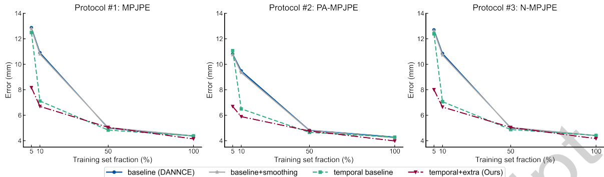
Fig. 3 Qualitative comparison of landmark localization performance over different annotation conditions. We randomly selected 5% ( n = 8 ), 10% ( n=17 ) and 50% ( n=85 ) of the training set to simulate low annotation regimes. Temporal supervision generally improved performance on all three localization protocols compared to the baseline models, especially with limited access to the training data. Similar improvement cannot be achieved via post hoc smoothing of the predicted movement trajectories.
