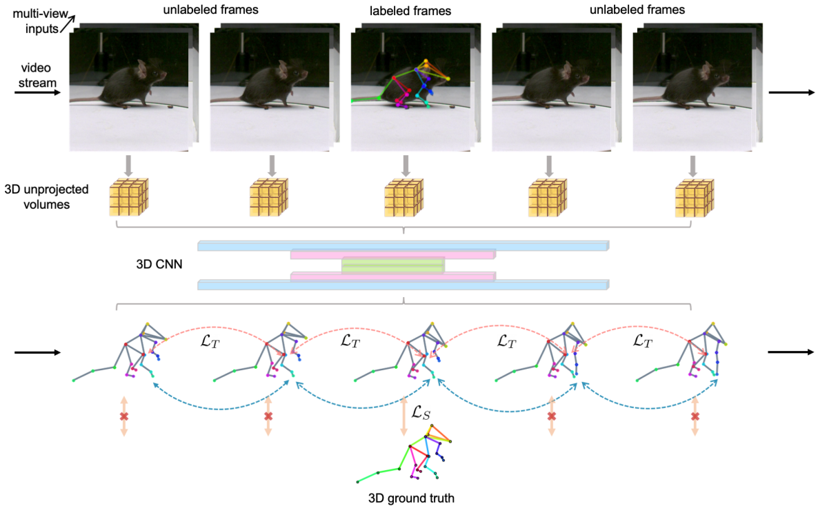
Fig. 1 Method Overview. Our multi-view volumetric approach constructs a 3D image feature grid using projective geometry for each timepoint in videos. A 3D CNN (UNet) processes batches of temporally contiguous volumetric inputs and directly predicts 3D keypoint positions. We then combine a traditional supervised regression loss with an unsupervised temporal consistency loss for training. While the regression loss \mathcal{L}_S is applied only on labeled video frames, which are sparsely distributed across video recordings, the unsupervised temporal loss \mathcal{L}_T operates over both labeled and unlabeled frames.
