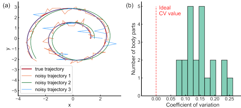
Fig. 2 (a) Ambiguity in absolute position error analysis. In this simulated example, we present three noisy trajectories with the same absolute point position errors with respect to the true spiral trajectory. (b) Histogram of body segment length variation in manually labeled mouse data. We compute the coefficient of variation (CV) for the lengths of 22 body segments. While CV values should ideally be close to 0, we instead observed notable amounts of length variation in all body segments. This illustrates the noise present in manually labeled 3D poses.
