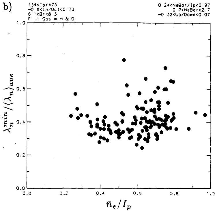
Figure 9.32 Scrape-off Length Asymmetry Relative to Poloidally Averaged Scrape-off Length vs. \bar{n}_e / I_p
