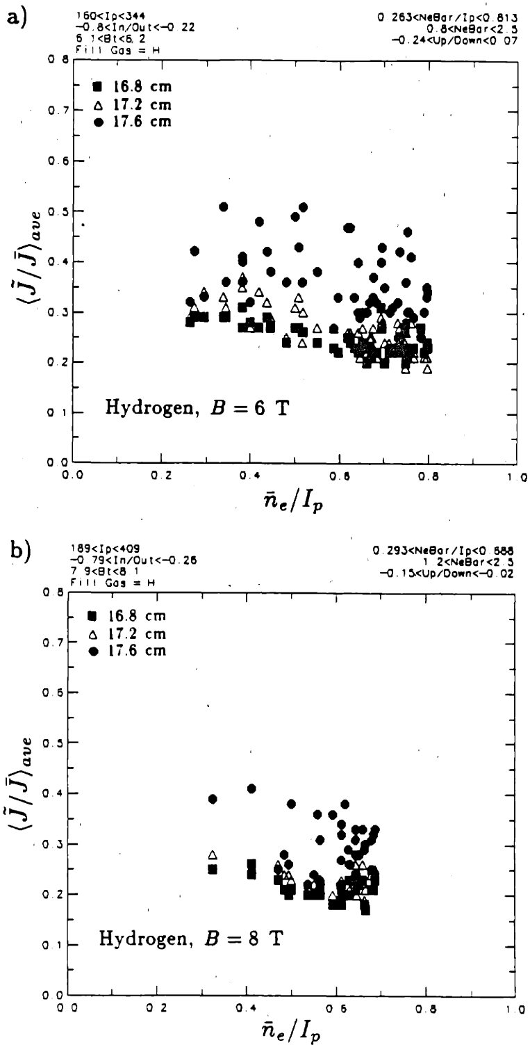
Figure 9.20 \langle \bar{J} / \bar{J} \rangle_{ave} vs. \bar{n}_e / I_p for Hydrogen Discharges in 6 and 8 tesla Toroidal Magnetic Fields
