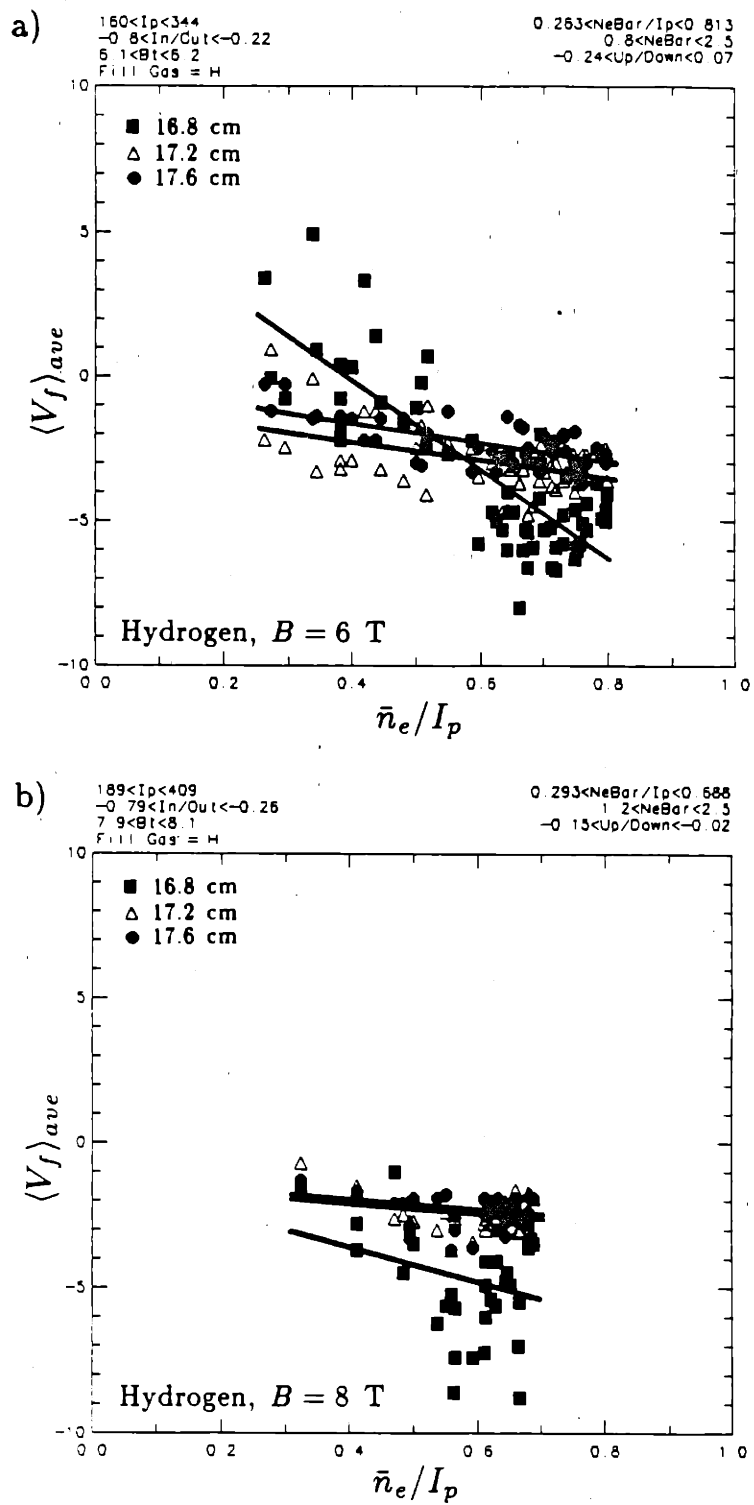
Figure 9.18 \langle V_f \rangle_{ave} vs. \bar{n}_e/I_p for Hydrogen Discharges in 6 and 8 tesla Toroidal Magnetic Fields
