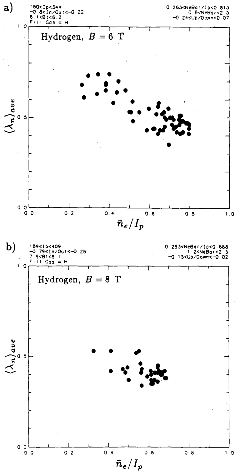
Figure 9.14 \langle \lambda_n \rangle_{ave} vs. \bar{n}_e/I_p for Hydrogen Discharges in 6 and 8 tesla Toroidal Magnetic Fields
