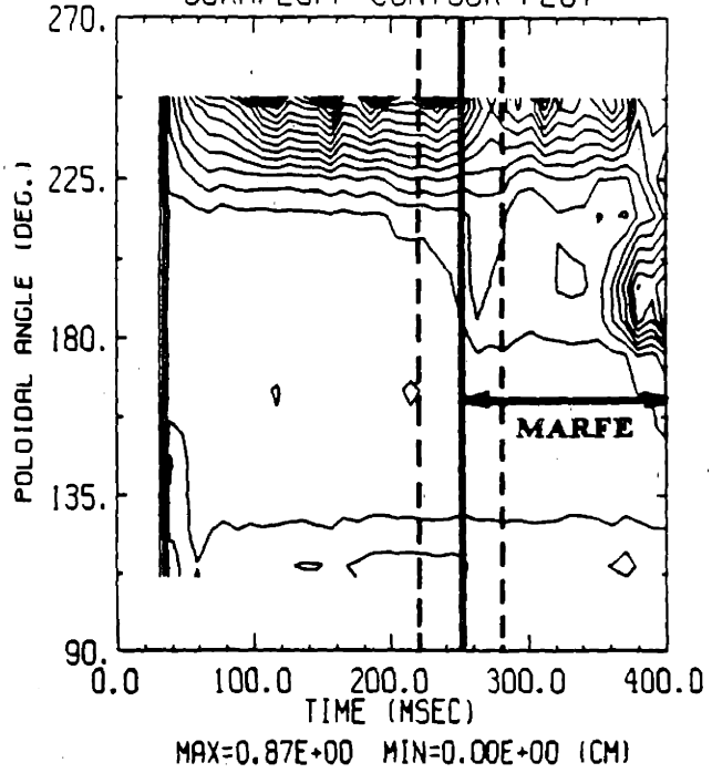
SCRAPEOFF CONTOUR PLOT
