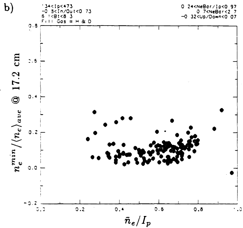
Figure 9.26 Density Asymmetry Relative to Poloidally Averaged Density at r = 17.2 \text{ cm} vs. \bar{n}_e / I_p
