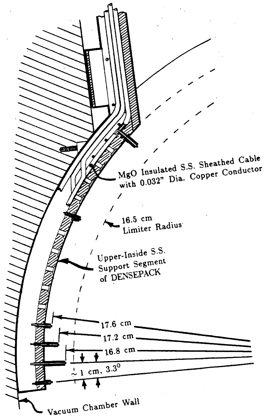
Figure 5.6 Schematic of Upper-Inside Segment of DENSEPACK
