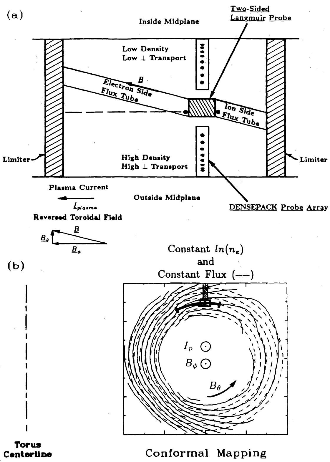
Figure 8.11 Flux Tubes Sampled by Two-Sided Langmuir Probe (reversed toroidal field direction)
