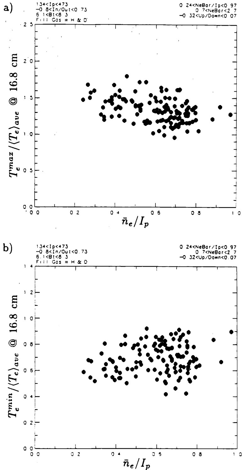
Figure 9.29 Temperature Asymmetry Relative to Poloidally Averaged Temperature at \tau = 16.8 \text{ cm} vs. \bar{n}_e / I_p
