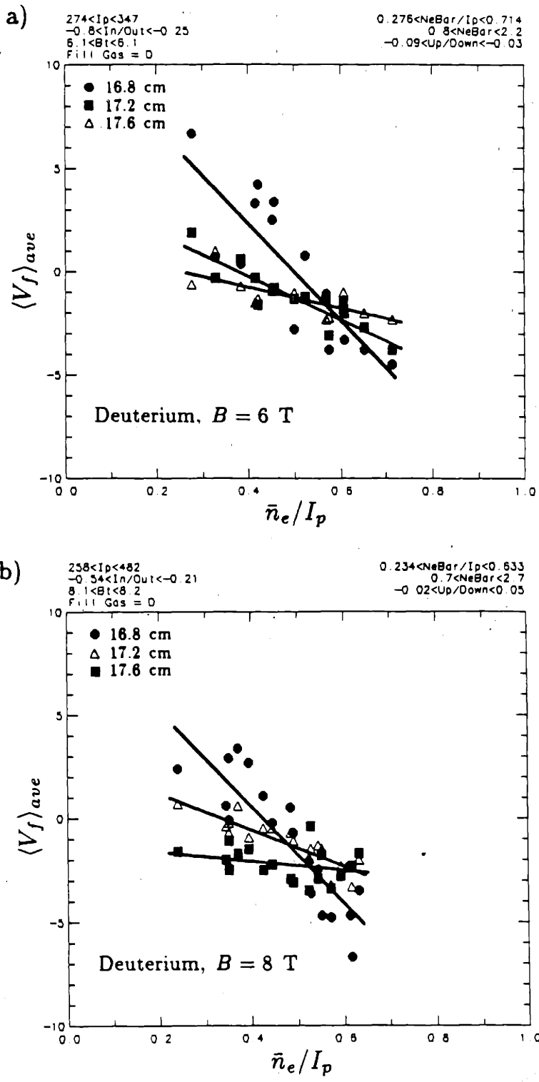
Figure 9.19 \langle V_f \rangle_{ave} vs. \bar{n}_e/I_p for Deuterium Discharges in 6 and 8 tesla Toroidal Magnetic Fields
