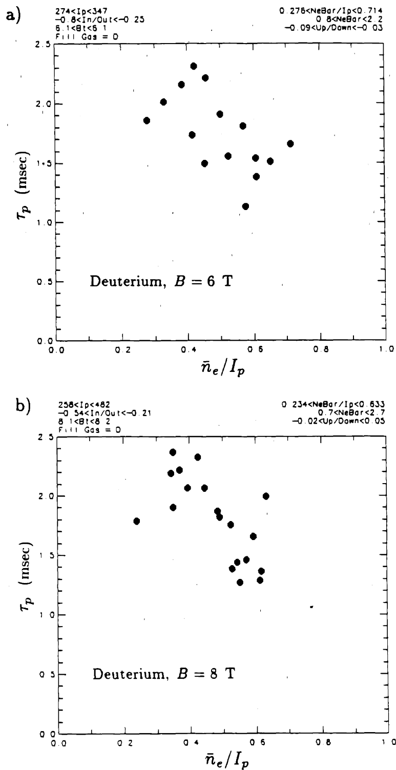
Figure 9.24 Estimated Global \tau_p vs. \bar{n}_e/I_p for Deuterium Discharges in 6 and 8 tesla Toroidal Magnetic Fields
