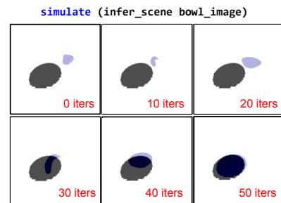
Fig. 2. Overview example: inferring the identity and pose of an object, given a point cloud
