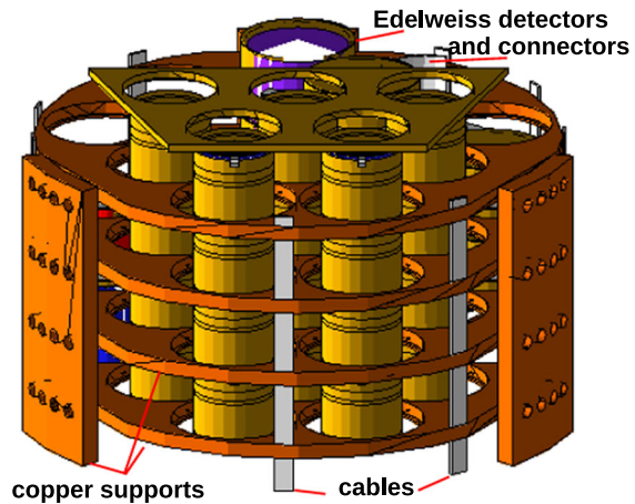
Inside the five towers are placed the LMO crystals, the light detectors, the clamps and the reflective foils (not seen). The readout cables and the structure supporting the towers are indicated
