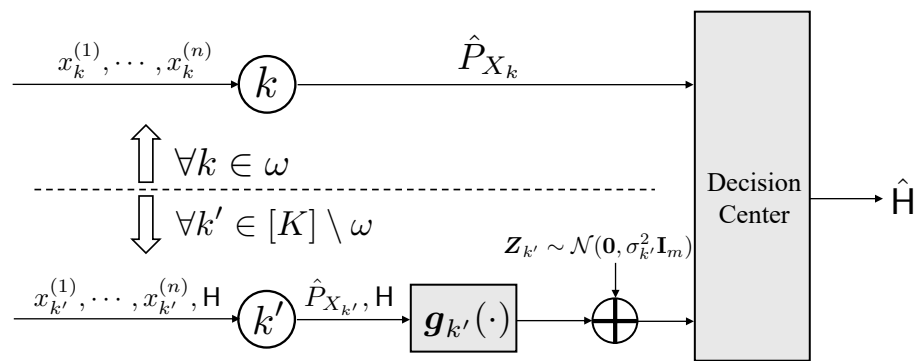
Figure 5. A geometric explanation of the genie-aided approach, which can lead to E_\omega as the upper bound of the error exponent in (4).
