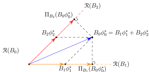
Figure 4. The information decomposition structure in distributed hypothesis testing with K = 2 nodes, compared with the orthogonal decompositions on the subspace \mathcal{R}(B_k) for each node k = 1, 2 .
