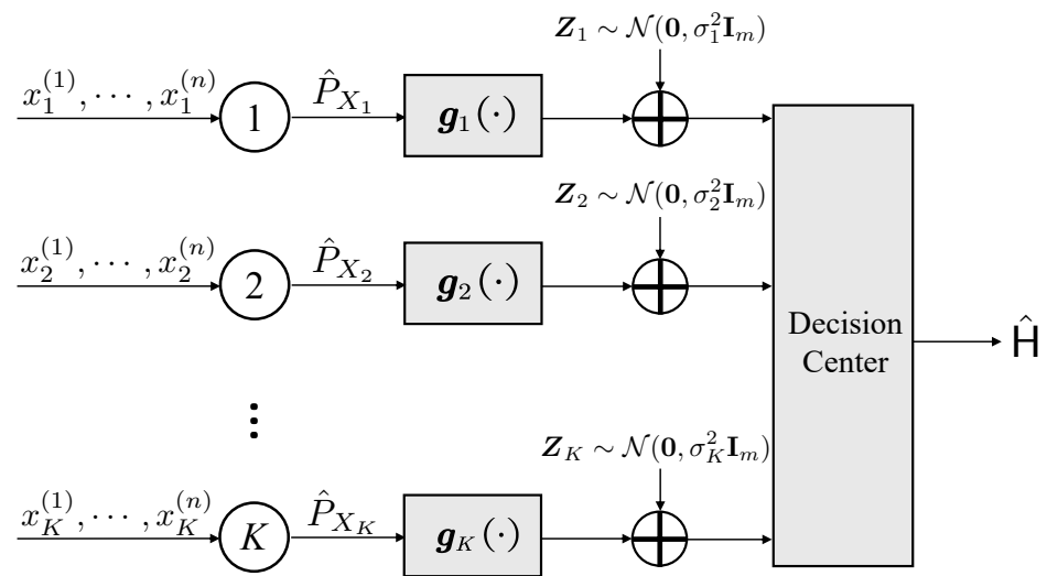
Figure 2. The transmission procedures for the type-based distributed hypothesis testing problem over AWGN channels.
