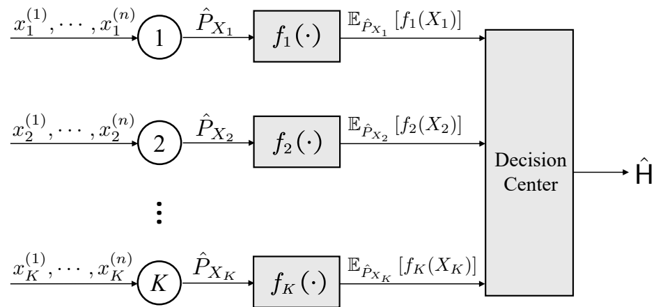
Figure 1. The transmission procedures for the type-based distributed hypothesis testing problem over noiseless channels.
