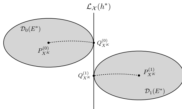
Figure 3. The geometric structure in distributed hypothesis testing, with Q_{X^k}^{(i)} denoting the I-projection of P_{X^k}^{(i)} onto the linear family \mathcal{L}_{\mathcal{X}}(h^*), i = 0, 1 , and \mathcal{L}_{\mathcal{X}}(h^*) can divide \mathcal{D}_0(E^*) and \mathcal{D}_1(E^*) in different half spaces.
