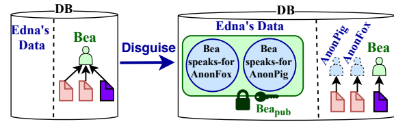
Figure 4. When Edna applies topic-based anonymization to Bea’s comments on stories tagged “Star Wars” (red), these comments are decorrelated to pseudoprincipals (“AnonPig”, “AnonFox”) and Edna stores encrypted speaks-for records mapping Bea to their pseudoprincipals.
