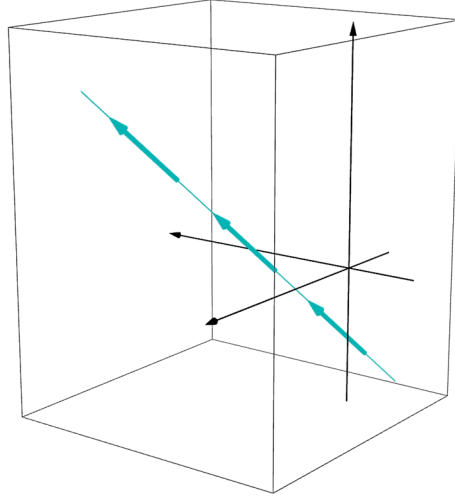
FIGURE 1. A blade \mathbf{n}_\infty \wedge \mathbf{a} \wedge \mathbf{b} \in \mathcal{G}_{4,1}^3 formed from three null vectors including the point-at-infinity \mathbf{n}_\infty can be interpreted as a line-bound vector , which is an oriented segment of a fixed line in space wherein the position of the segment on the line is indeterminate. (All the figures in this paper were prepared using the GeoGebra dynamic geometry software)
