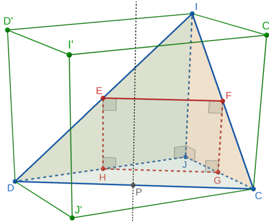
FIGURE 7. Drawing of the right-tetrahedron [[\mathbf{c}, \mathbf{d}, \mathbf{i}, \mathbf{j}]] , with vertices labeled C, D, I, J resp. The medial parallelogram of n_\infty \wedge \mathbf{c} \wedge \mathbf{d} and n_\infty \wedge \mathbf{i} \wedge \mathbf{j} , with vertices labeled E, F, G, H and an area of \|\mathbf{i} - \mathbf{j}\| \|\mathbf{c} - \mathbf{d}\| / 4 , is drawn in red, while an enveloping right-parallelepiped, wherein I', J' are obtained by \pi -rotations of I, J about the perpendicular line through the midpoint P of [[\mathbf{c}, \mathbf{d}]] , is in green
