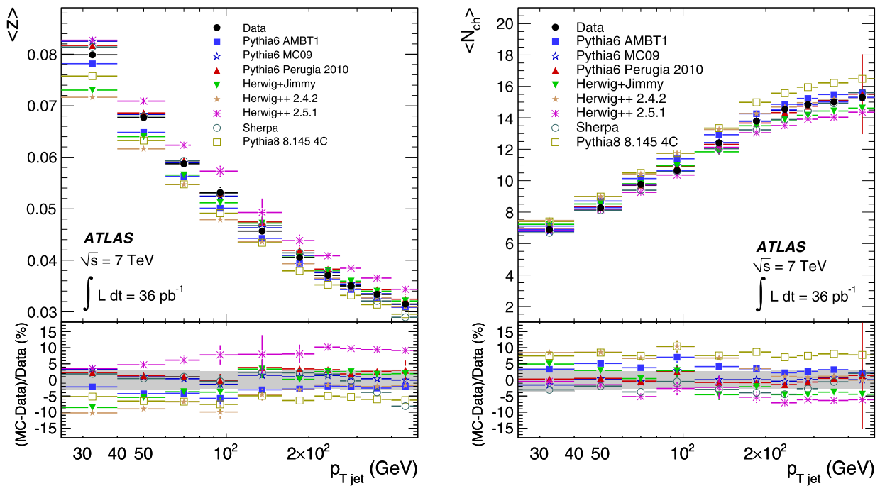
Fig. 7 Distributions of \langle z \rangle (left) and of the mean number of charged particles selected with the requirement p_{T,track} > 500 \text{ MeV} (right) as a function of p_{T,jet} for data and various Monte Carlos. The gray band indicated the total uncertainty
