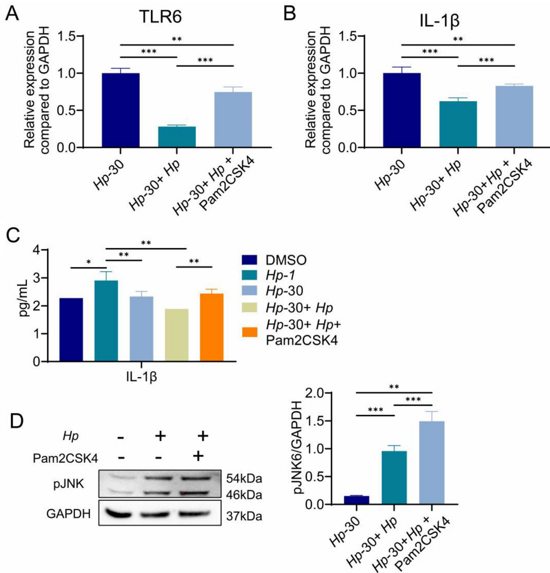
Fig. 4 TLR6 mRNA expression ( A ) and IL-1β mRNA expression ( B ) in Hp-30 cells, Hp-30 cells co-culture with H. pylori for 24 h and Hp-30 cells co-culture with H. pylori and 10 μg/ml Pam2CSK4 for 24 h. Supernatant IL-1β content ( C ) in control cells, Hp-1 cells, Hp-30 cells, Hp-30 cells infected with H. pylori for 24 h and Hp-
