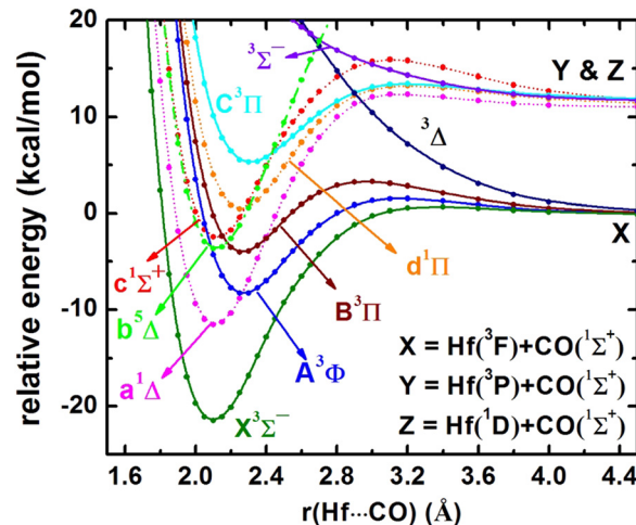
Fig. 1 Full MRCI PECs of HfCO with respect to the Hf...C distance [ r(\text{Hf}\cdots\text{C}) ] in Å. The CO distance is kept fixed to the experimental bond distance of CO ( X^1\Sigma^+ ) 1.128 Å. Only the b^5\Delta state originating from the interaction of Hf( ^3\text{F} ) + CO( X^1\Sigma^+ ) is depicted. Relative energies are referenced to the total energy of the Hf( ^3\text{F} ) + CO( X^1\Sigma^+ ) fragments, which are set to 0 kcal mol -1 . The PECs with triplet, singlet, and quintet spins are shown in solid, dotted, and dashed lines.
