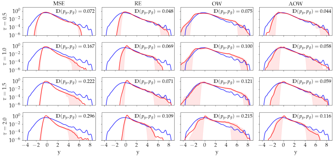
Figure 10: Density functions for the drag on a square cylinder using true data (blue) and 20 realizations of neural networks trained with each loss function (red).
