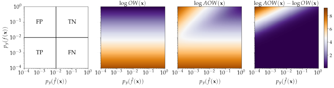
Figure 1: Visualization of weights used by L_{OW} and L_{AOW} . Left most figure shows hypothetical boundaries for true/false positive/negative regions. Pseudocolor plots show output weight, adjusted output weight, and difference. Disagreement is primarily within the false positive region.
