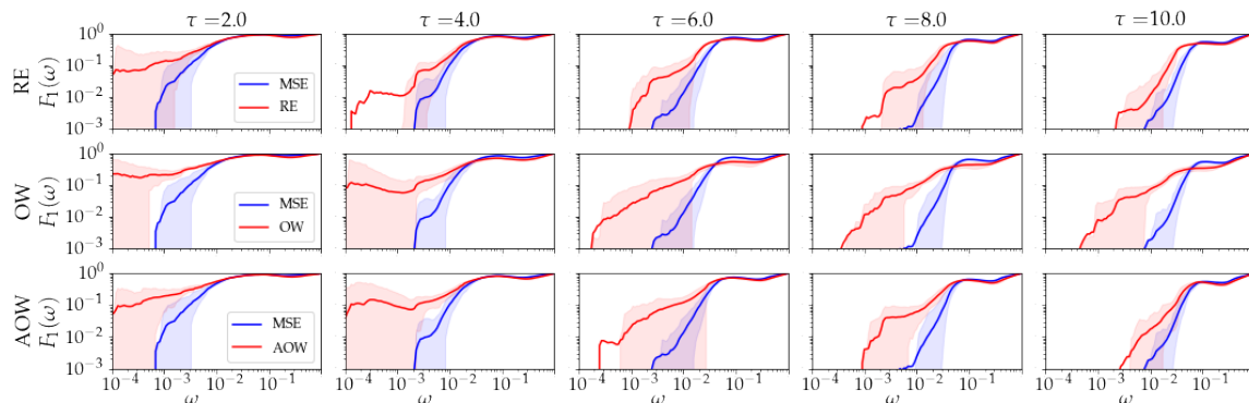
Figure 7: Comparison of F_1(\omega) for models trained using L_{MSE} (blue) and extreme event specific loss functions (red) for the Kolmogorov dataset. Lines indicates mean and shaded region is bounded by 10th and 90th percentiles.
