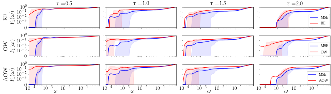
Figure 13: Comparison of F_1(\omega) for models trained using L_{MSE} (blue) and extreme event specific loss functions (red) for the square dataset.
