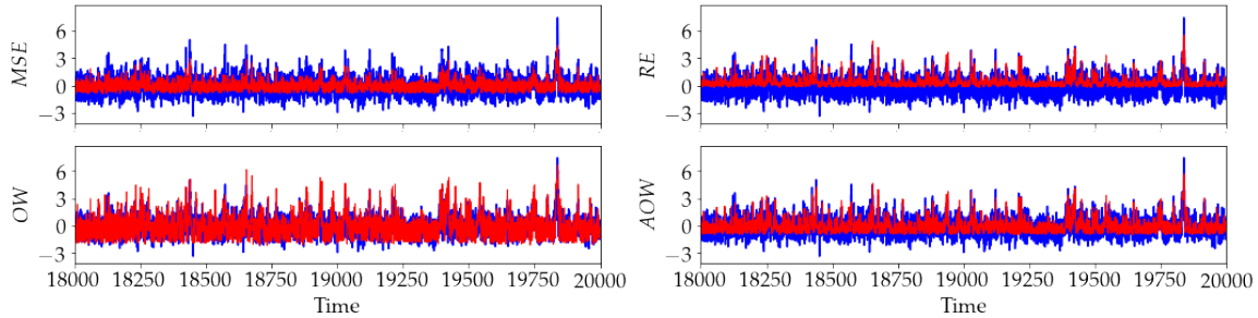
Figure 9: True centered and normalized drag coefficient (blue) and mean time series predictions (red) for test set data from each neural network for the drag on a square cylinder. Results are for a lead time of \tau = 1 .
