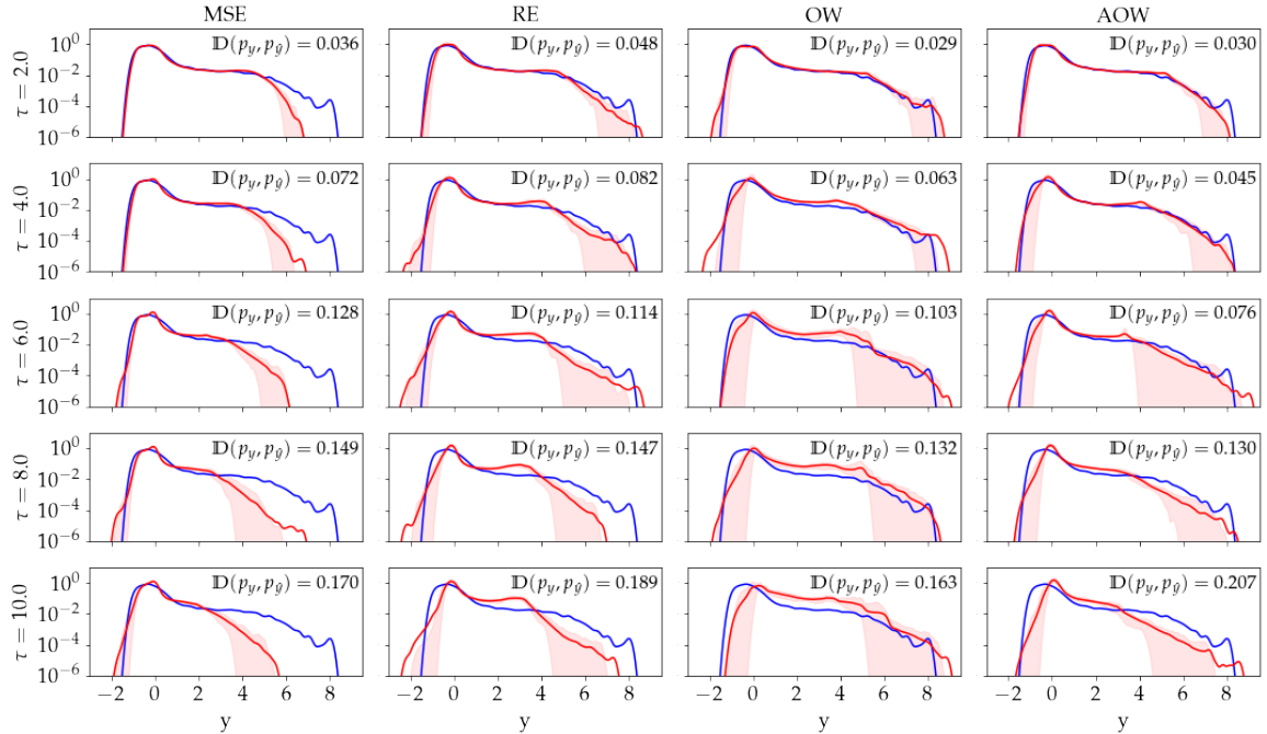
Figure 4: Density for the Kolmogorov flow energy dissipation using true data (blue) and 20 realizations of neural networks trained with each loss function (red). Reported \mathbb{D} is mean of Eq. (19).
