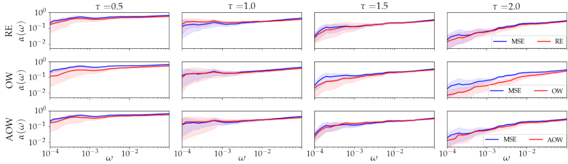
Figure 12: Comparison of \alpha(\omega) for models trained using L_{MSE} (blue) and extreme event specific loss functions (red) for the square dataset.
