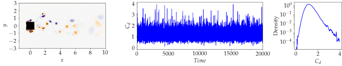
Figure 8: Flow around a square cylinder at Re = 5000 . Left: Snapshot of vorticity close to cylinder. Center: Time series for drag coefficient. Right: Empirical density function of drag coefficient.
