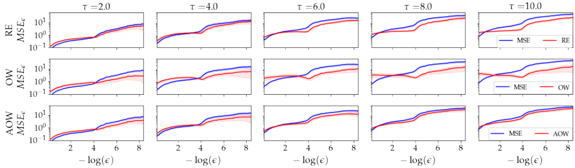
Figure 5: Comparison of MSE_\epsilon for models trained using L_{MSE} (blue) and extreme event specific loss functions (red) for the Kolmogorov dataset. Note that high -\log(\epsilon) corresponds to rare events.
