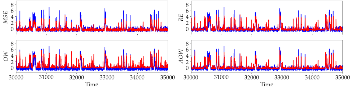
Figure 3: Mean predictions for subset of test data for the Kolmogorov dataset at lead time \tau = 6 . Blue time series is true D(t) and red is mean prediction across 20 trained neural networks.
