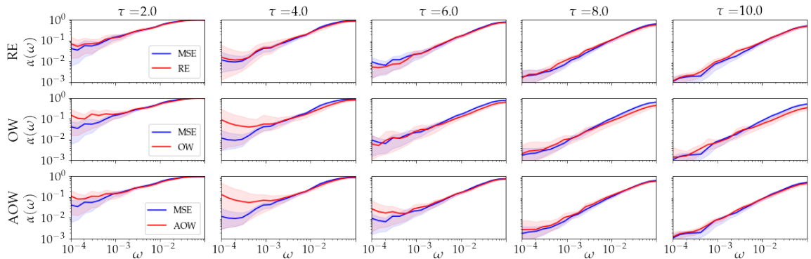
Figure 6: Comparison of \alpha(\omega) for models trained using L_{MSE} (blue) and extreme event specific loss functions (red) for the Kolmogorov dataset.
