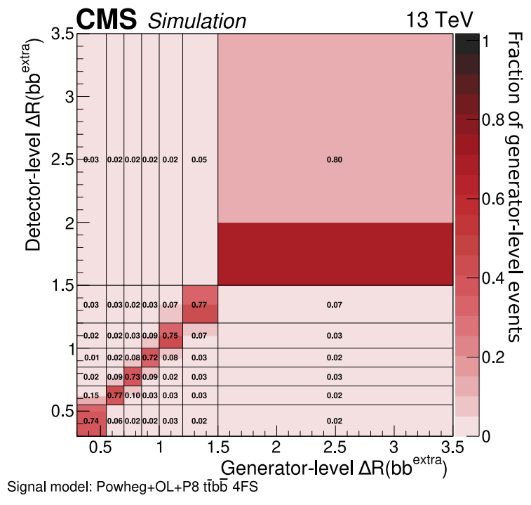
Figure 4. Response matrix for \Delta R(\text{bb}^{\text{extra}}) in the \geq 6 jets: \geq 4\text{b} phase space. The x ( y ) axes show the generator- (detector-)level observables. The upper figure includes the ancillary variable, unrolled on the same axis as the detector-level observable, so that the binning of the detector-level observable, stacked vertically, is repeated twice. For the lower figure, the ancillary variables are projected out to more easily visualize the correspondence between true and reconstructed values. The coloured bins show the finer binning used at reconstructed level (bins split in two), while the numbers show the values one would obtain when using the same binning at the generator and detector level.
