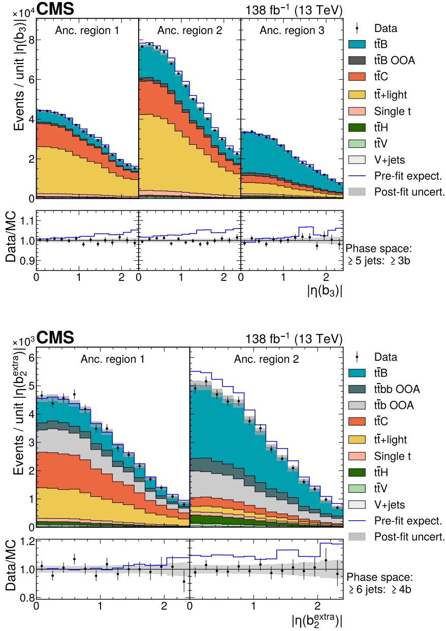
Figure 7. The |\eta| of the third-hardest b jet in p_T ( |\eta(b_3)| ) in the \geq 5 jets: \geq 3b phase space (upper) and the |\eta| of the subleading additional b jet ( |\eta(b_2^{extra})| ) in the \geq 6 jets: \geq 4b phase space (lower) after the fit to data, shown for both lepton channels and all data periods combined. The distributions are shown separately for each ancillary region, as defined in section 6.1. In the \geq 5 jets: \geq 3b ( \geq 6 jets: \geq 4b ) phase space the ancillary regions are defined as \leq 2 , 2, and \geq 3 ( \leq 3 and \geq 3 ) tight b-tagged jets. The shaded bands include all uncertainties described in section 7 after profiling the nuisance parameters in the fit, estimated by sampling the predicted yields from the fit covariance matrix. The blue line shows the sum of the predicted yields for all processes before the fit to data, using the nominal t\bar{t}b\bar{b} samples and its corresponding cross section for the signal. In the ratio panel the expected yields before the fit to data are shown relative to the predicted yields after the fit to data. The last bins contain the overflow.
