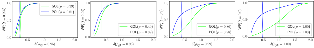
Figure 5.D.10: The plot of \delta vs. WP_t^\delta for the max-cut problem. See the caption of Fig. 5.D.4 for the meaning of the symbols. As different edge weights lead to different minima values, we choose the threshold t in a relative manner: the actual threshold used will be t times the best objective value found by PD.
