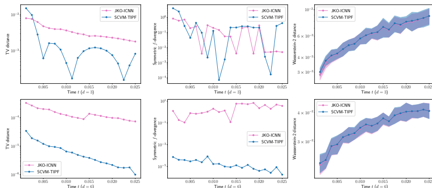
Figure 6.D.1: Metrics (TV, Symmetric f -divergence and Wasserstein-2 distance) across time for dimensions 3 and 6 between the estimated \mu_t and the ground-truth \mu_t^* when solving the Porous Medium Equation.
