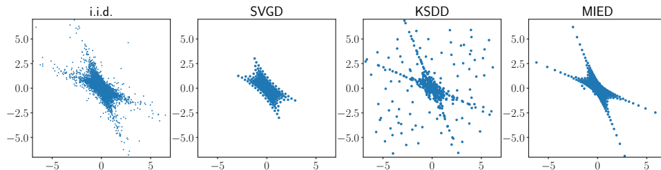
Figure 1.1: Mollified interaction energy descent (MIED) from Chapter 2 obtains well-spread samples from a heavy-tail distribution compared with i.i.d. samples and particle-based alternatives such as SVGD [LW16] and KSDD [Kor+21a].
