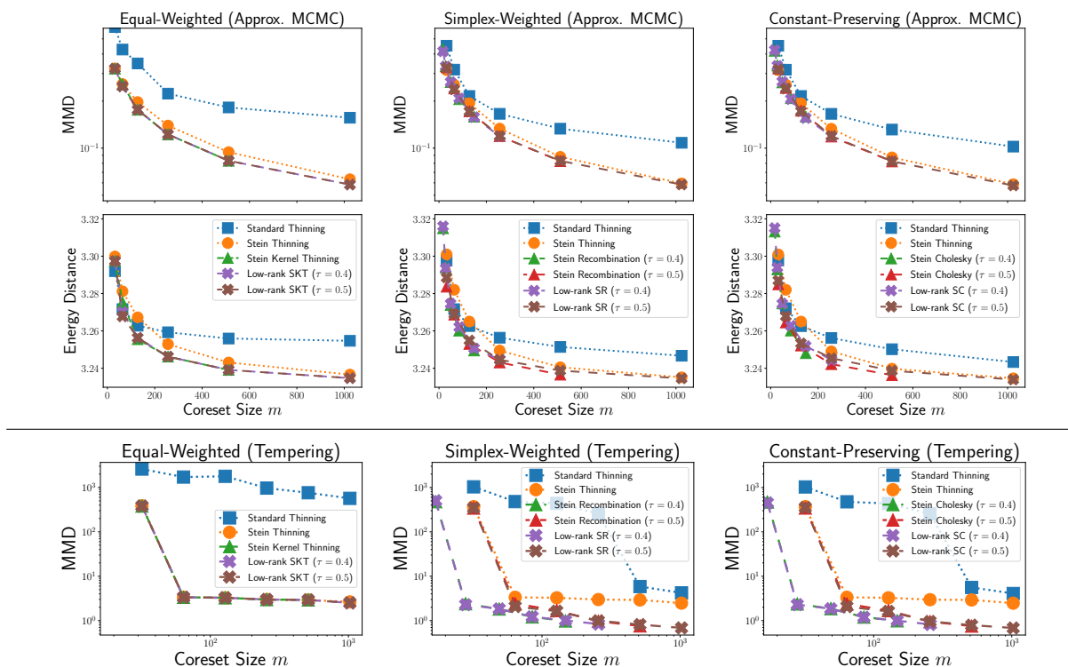
Figure 2: Correcting for approximate MCMC (top) and tempering (bottom). For posterior inference over the parameters of Bayesian logistic regression ( d = 54 , top) and a cardiac calcium signaling model ( d = 38 , bottom), our concise coreset constructions correct for approximate MCMC and tempering biases without need for explicit importance sampling.
