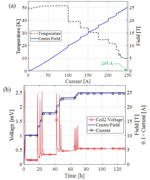
Fig. 6. The prototype magnet operation results: (a) temperature adjusting operation sequence up to 25 T at 245 A; and (b) center field and current vs.
