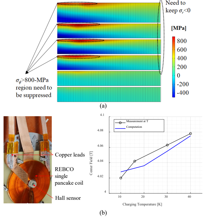
Fig. 4. Screening currents in the REBCO magnet: (a) hoop stress distribution in the 23.5-T prototype magnet at 10 K; and (b) validation test result by using a single pancake coil ramping up to 255 A.
