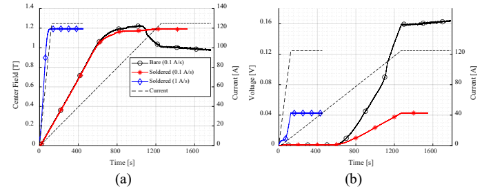
Fig. 3. Over-current testing results of test coils, bare and soldered, up to 125 A with 0.1 \text{ A}\cdot\text{s}^{-1} and 1 \text{ A}\cdot\text{s}^{-1} : (a) center field vs. time; and (b) voltage vs. time.
