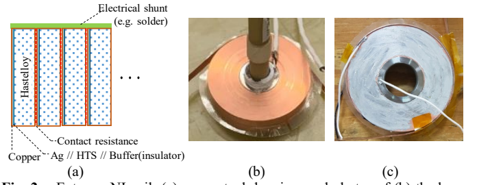
Fig. 2. Extreme-NI coil: (a) conceptual drawing; and photos of (b) the bare NI DP coil and (c) the NI DP coil with soldered surfaces.
