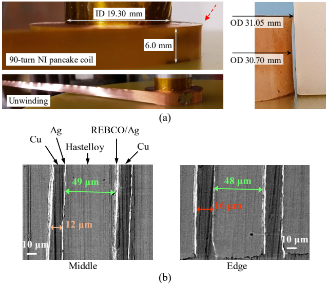
Fig. 1. A REBCO NI pancake test coil: (a) 90-turn winding and unwinding; (b) SEM images of cross-sections of middle and edge sides of the test coil.
