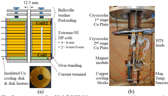
Fig. 5. A cryogen-free 23.5-T REBCO prototype magnet: (a) a cross-section view of schematic drawing; and (b) a photo of the magnet assembly.
