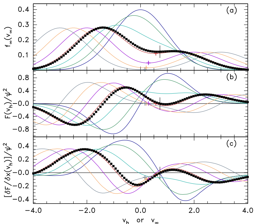
FIG. 7. Stability parameters as a function of v_h , for a range of distributions obtained by scaling the Maxwellian components' shift velocity ( v_{shift} \propto 0, .33, .66, 1., 1.33, 1.66, 2. ).
