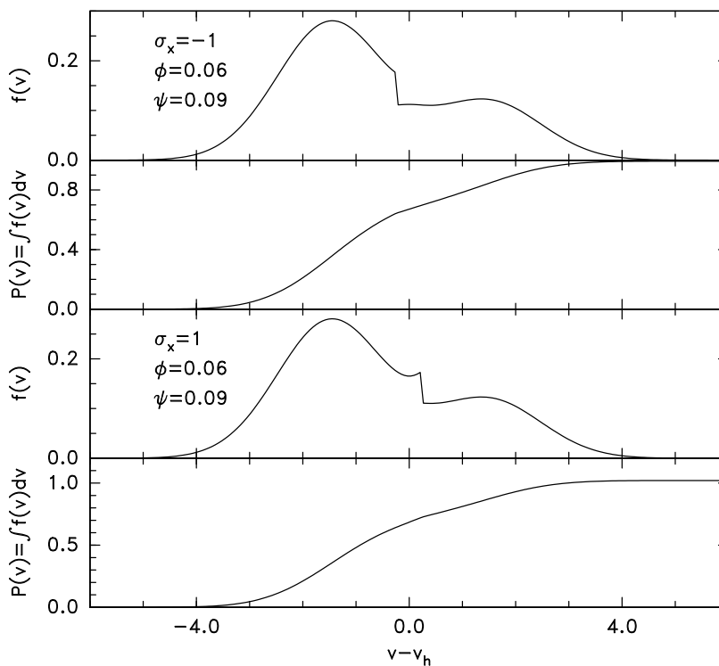
FIG. 2. Illustration of ion distributions on either side of the potential hill, and their integral P(v) , which is the cumulative probability distribution multiplied by n_i(\phi) (equal to n_i(\phi) at v = +\infty ).
