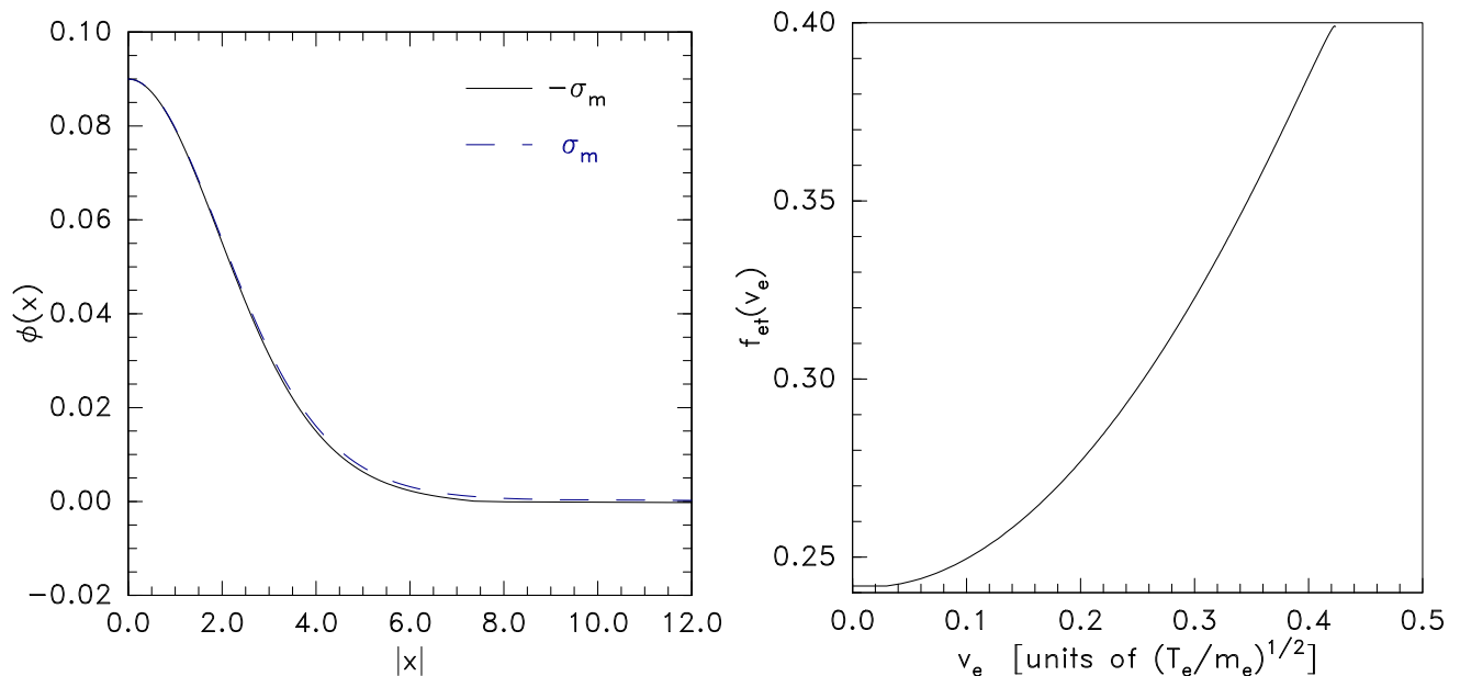
FIG. 6. (a) Potentials on the two sides of the hole. Prescribed side dashed line, Poisson solution side solid. (b) Corresponding trapped electron distribution function at x = 0 , \phi = \psi .
