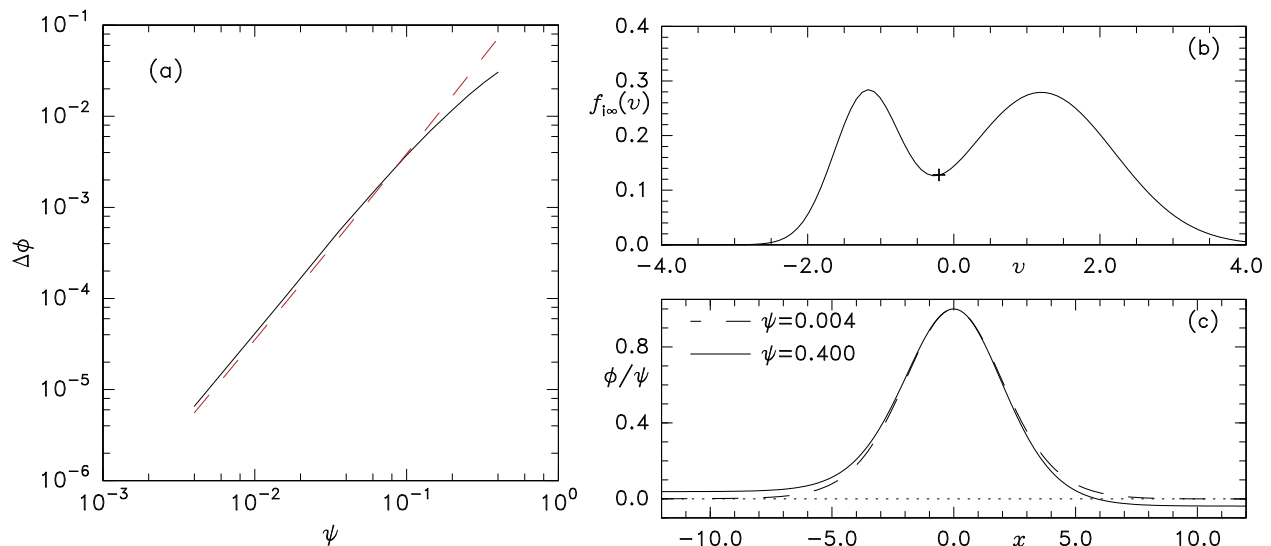
FIG. 9. (a) Comparison of numerical (solid black) and algebraic (dashed red) estimates of potential asymmetry \Delta\phi , showing its scaling proportional to the square of the electron hole peak potential \psi . In (b) is shown the ion distribution comprising Maxwellians T_1 = 1 , n_1 = 0.7 , v_1 = 1.197 , T_2 = 0.2 , n_2 = 0.3 , v_2 = -1.197 , and T_e = 1 , in scaled units. The potential profiles in (c) are from the ends of the scaling range.
