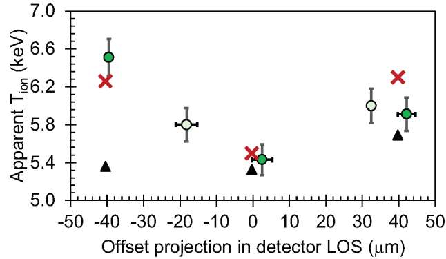
FIG. 6. (color online) Apparent T_{\text{ion}} as measured using the Petal nTOF (green circles) and simulated for the same LOS using 2D xRAGE (red crosses). Also shown is the 2D xRAGE-simulated BWTI T_{\text{ion}} , which is the thermal T_{\text{ion}} not considering flow broadening of the neutron spectrum (black triangles).
