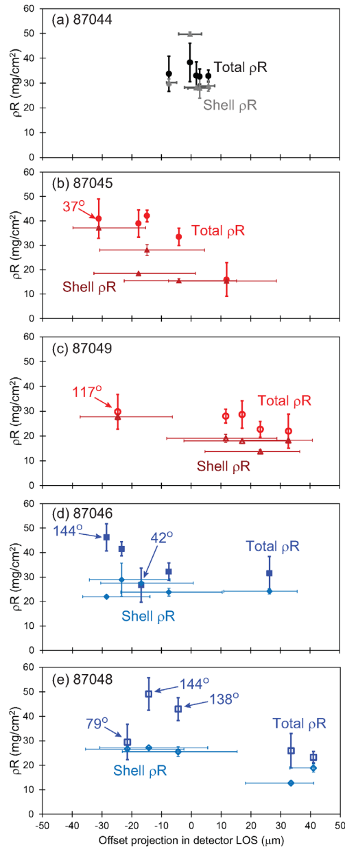
FIG. 14. (color online) Total (inferred from D^3He -p downshift) and shell (inferred from KO-p yield) \rho R for (a, b, c) shots 87044, 87045 and 87049, with capsule held by TIM4 (with circles and triangles representing total and shell \rho R , respectively), and (d, e) shots 87046 and 87048, with capsule held by TPS2 (with squares and diamonds representing total and shell \rho R , respectively). The angles shown in the figure represent the angle to the stalk for the indicated measurements. The \rho R asymmetry appears dominated by the offset.
