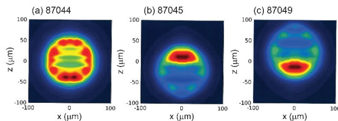
FIG. 8. (color online) 2D xRAGE-simulated time-integrated x-ray images for (a) shot 87044 (symmetric reference), (b) shot 87045 (downwards offset) and (c) shot 87049 (upwards offset). The stalk enters from the top in each image.
