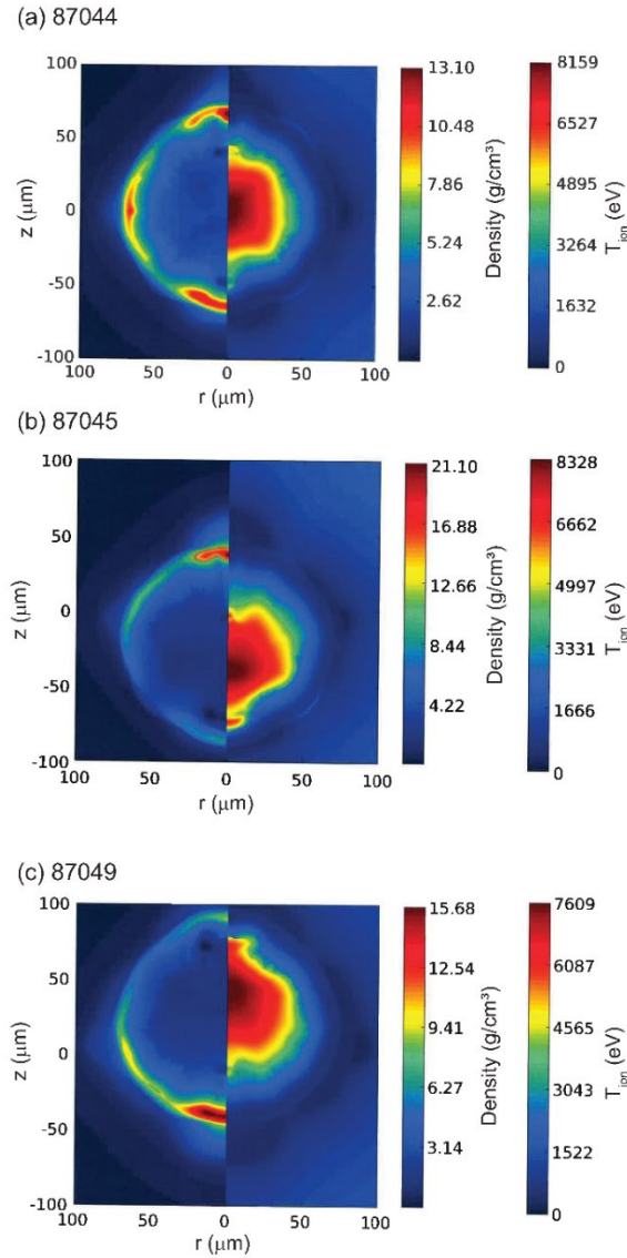
FIG. 3. (color online) 2D xRAGE-simulated density (left) and T_{\text{ion}} (right) color maps at bang time for (a) shot 87044, (b) shot 87045 and (c) shot 87049. The stalk is entering from the top in each image.
