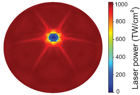
FIG. 13. (color online) Static VisRad simulation of an on-center capsule include stalk and glue spot. There is a clear spoke pattern from stalk shadowing.
