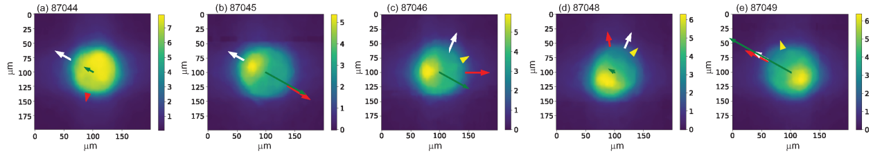
FIG. 7. (color online) Time-integrated x-ray images recorded with the GMXI diagnostic for (a) symmetric reference shot 87044, (b) shot 87045 with the offset away from the stalk, (c) shot 87046 with the offset at 76^\circ to the stalk, (d) shot 87048 with the offset at 42^\circ to the stalk, and (e) shot 87049 with the offset towards the stalk. The white arrow indicates the direction of the stalk mount in the GMXI plane, the red arrow the direction and magnitude of the offset. Note that there is a clear local enhancement (yellow) in the x-ray signal opposite the stalk for all offset shots except 87048, where the asymmetry does not appear to correlate with the offset direction. The green arrows represent the flow velocities (direction and magnitude) as measured with the Petal nTOF (note that Petal is located in the lower right in the image – a negative measured velocity will have the arrow pointed in the opposite direction). The yellow arrows in panels (c, d, e) represent the GMXI-plane projections of the mode 1 vector inferred from framing camera images.
