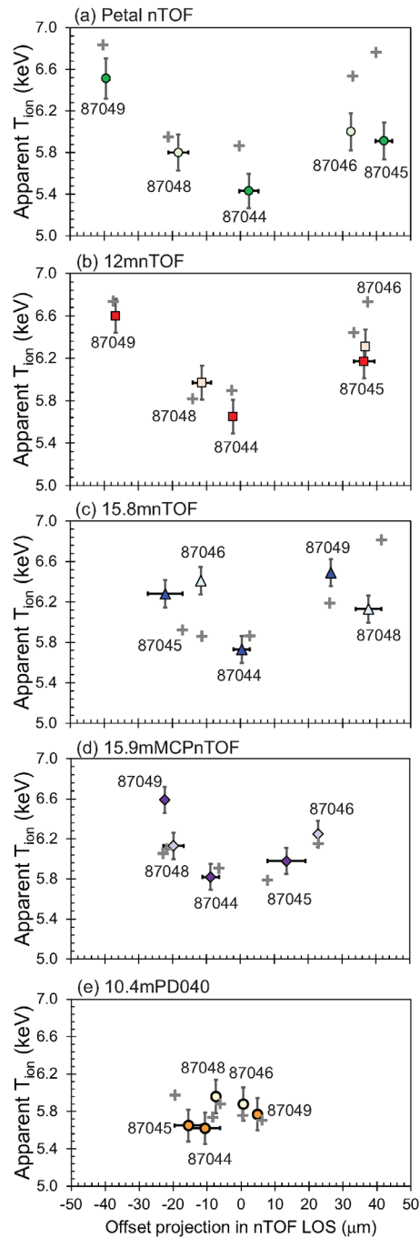
FIG. 5. (color online) Measured apparent T_{ion} as a function of offset projection in the nTOF line-of-sight for (a) Petal nTOF, (b) 12mntof, (c) 15.8mntof, (d) 15.9mMCPnTOF, and (e) 10.4mPD040 (see FIG. 2 for nTOF locations). Light symbols represent shots with the stalk in TPS2, while dark symbols represent shots with the stalk in TIM4. The offset projection is the average projection obtained using HSV and XRPC measured offsets, with the error bar spanning the range of using one or the other to calculate the projection. Gray plus signs represent 3D Chimera-simulated T_{ion} , using HSV offsets.
