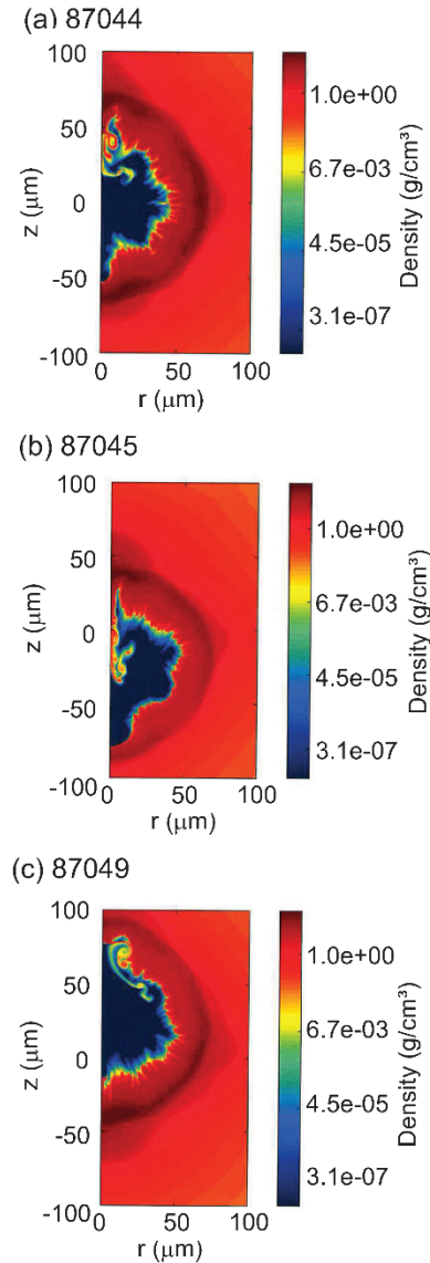
FIG. 12. (color online) 2D xRAGE-simulated contaminant density maps for (a) shot 87044 (symmetric reference), (b) shot 87045 (downwards offset) and (c) shot 87049 (upwards offset). The stalk is entering from the top in each image. These contaminant maps clearly show how shell/glue material is entrained into the hot spot by the jet formed due to drive shadowing.
