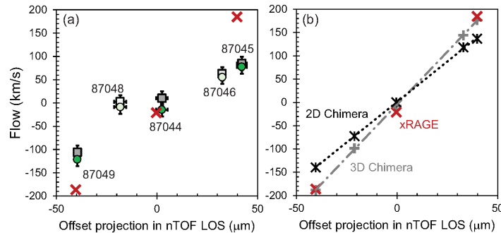
FIG. 4. (color online) (a) Directional flow as measured with the Petal nTOF (green circles) and the 8x4m nTOF (gray squares), sharing a single LOS. For Petal nTOF, the flow velocity is inferred from the DT neutron peak, while for 8x4mntof, the flow velocity is inferred from the DD neutron peak. Light data points represent shots with the stalk in TPS2, while dark data points represent shots with the stalk held by TIM4. The measured offset projection is the average projection obtained using HSV and XRPC measured offsets, with the error bar spanning the range of using one or the other to calculate the projection. Also shown are the xRAGE-simulated directional flows in the Petal LOS (red crosses). (b) xRAGE and Chimera-simulated directional flows, plotted against projected HSV offsets. The xRAGE results are shown in both panels for easy comparison.
