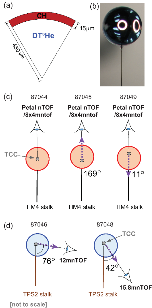
FIG. 1. (color online) Nominal experiment geometry. Target dimensions are shown in (a), a picture of the target used for shot 87048 in (b), and cartoons (not to scale) of the setup geometry for targets fielded on the TIM4 and TPS2 target positioners in (c) and (d), respectively. The cartoons show TCC as a grey cross, the offset direction with a purple dashed arrow, and the nTOF detector with maximum expected flow signature in each case as an eye. For the offset shots, the as-shot angles [as measured using high-speed video (HSV)] between the stalk and the offset directions are also indicated. Please note that targets are centered on the stalk for all shots; the offsets are exaggerated in the cartoon for illustration purposes only.
