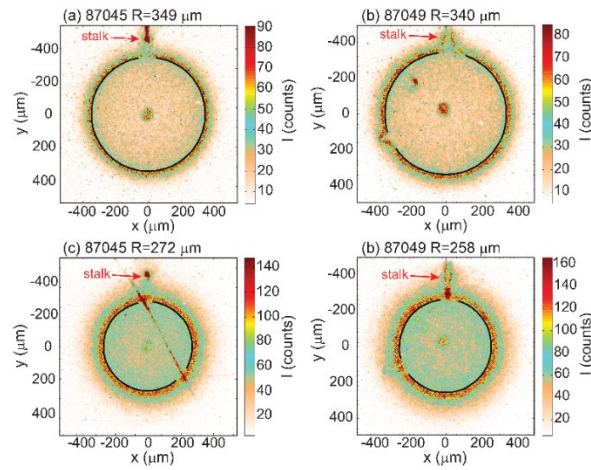
FIG. 9. (color online) Framing camera images obtained using a framing camera fielded in TIM2 with \theta=37^\circ , \phi=162^\circ for (a,c) shot 87045 with the offset away from the stalk, and (b,d) shot 87049 with the offset towards the stalk. The images in (a,b) are taken about 220 ps prior to the images in (c,d). The images visually show how the stalk perturbation is larger for the case with the offset towards (87049) than away from (87045) the stalk. The feature visible in the lower left corner of the images for 87049 \sim 120^\circ from the stalk arises due to residual glue from an initial, failed, stalk mount of this target.
