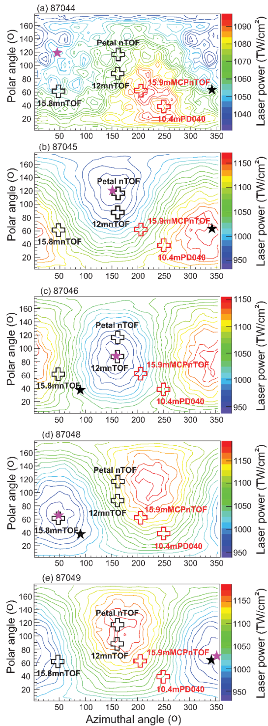
FIG. 2. (color online) VisRad-calculated drive asymmetry equivalent of the offsets, considering the as-shot laser drive but not the stalk and not any cross-beam energy transfer, for (a) symmetric reference shot 87044, (b) shot 87045 with the offset away from the stalk, (c) shot 87046 with the offset at 76^\circ to the stalk, (d) shot 87048 with the offset at 42^\circ to the stalk, and (e) shot 87049 with the offset towards the stalk. In each panel, the five nTOF detector directions are indicated with plus signs, the stalk direction with a black star, and the offset direction with a purple star. The (max-min)/min drive equivalent is 6.8% for shot 87044, 26.1% for shot 87045, 23.5% for shot 87046, 27.4% for shot 87048 and 28.1% for shot 87049.
