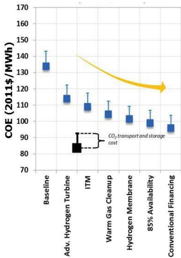
(b) IGCC plant
