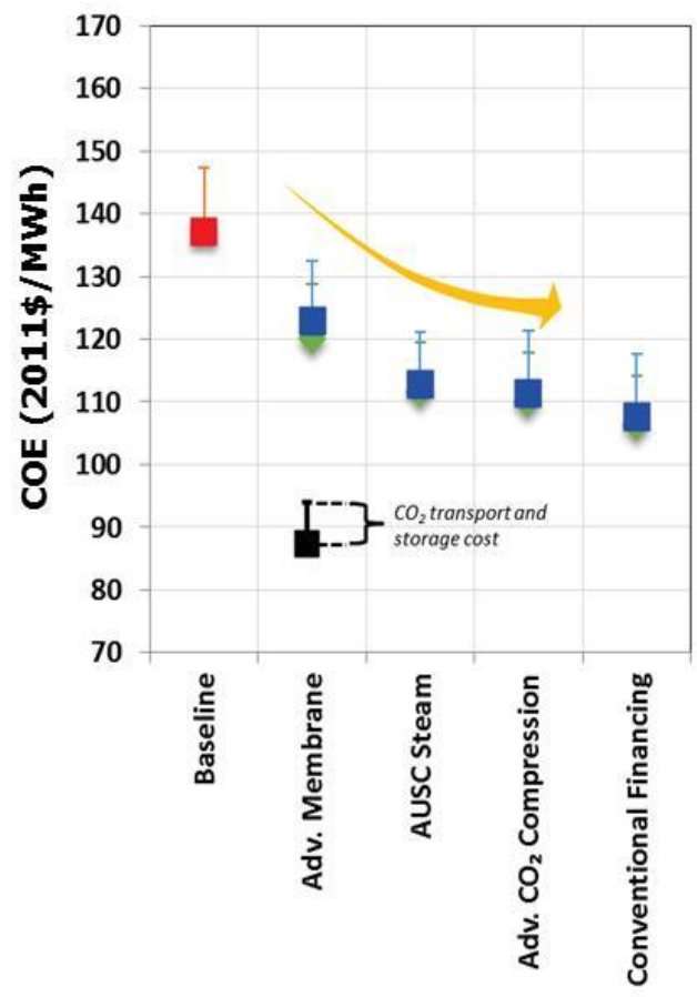
(a) PC plant
