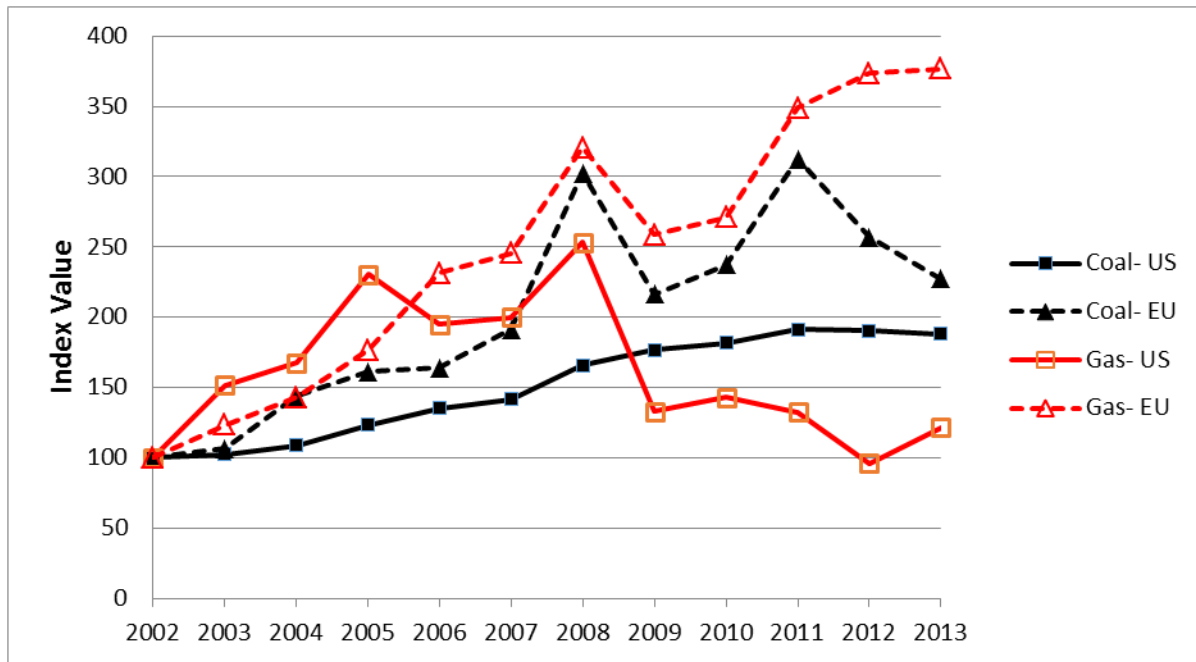
Figure 2. Fuel cost indices for coal and natural gas used by power plants in the US and Europe, normalized to 100 in year 2002 (based on data from USEIA, 2014; IEA, 2014).
