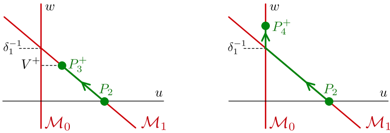
Fig. 3 Schematic of the singular heteroclinic orbit in the benign case where u \neq 0 after the invasion of the traveling wave (left) and the malignant case where u = 0 after the invasion (right)
