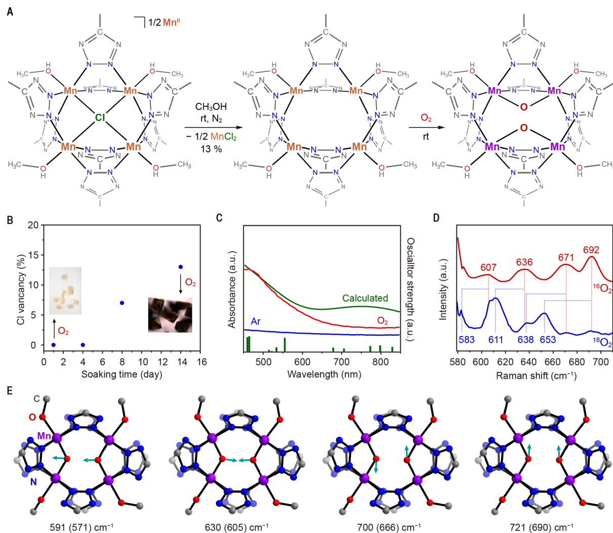
Figure 2. Generation of tetramanganese sites and oxygen reduction reactivity. (a) Generation of tetramanganese open site and its \text{O}_2 reduction reactivity. (b) Average chloride vacancy in each SBU determined by XPS, as a function of methanol soaking time. Insets show the color of activated, \text{O}_2 -exposed samples that were soaked in methanol for 1 day and 14 days, respectively. (c) Experimental electronic absorption spectra of activated 2 (blue trace) and 3 (red trace), and calculated electronic adsorption spectra of 3 (green trace), along with calculated individual excitations (green bars). (d) Raman spectra of 3 - ^{16}\text{O} and 3 - ^{18}\text{O} . (e) Simulated vibrational modes and corresponding frequencies for the [\text{Mn}_4(\mu\text{-O})_2(\text{tetrazole})_8(\text{CH}_3\text{OH})_4] unit. Vibrational frequencies for ^{18}\text{O} models are shown in parentheses.
