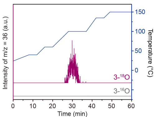
Figure 4. O 2 evolution from 3- 18 O . Oxygen evolution reactions were conducted in a continuous, tubular flow reactor under helium flow. The intensity of m/z = 36 of the outlet gas was monitored using mass spectrometry.
