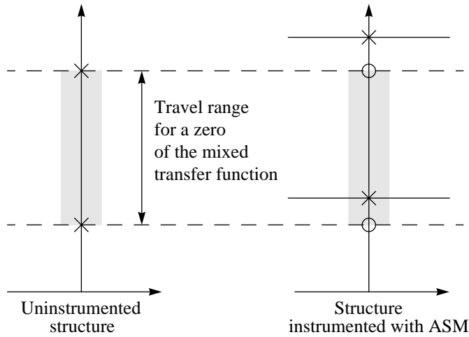
Figure 2.5 An illustration of the relationship between the poles of the original uninstrumented structure, the zeroes of the force transfer function and the travel range for the zeroes of the mixed transfer function.
