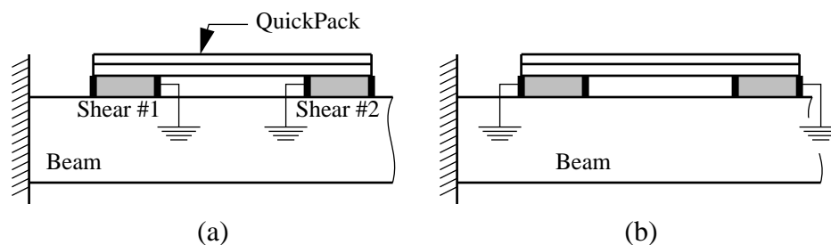
Figure 4.4 Two candidate electrode grounding schemes: (a) both inside electrodes are grounded; (b) both outside electrodes are grounded.
