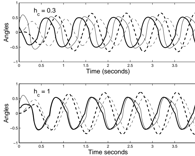
Figure 5-5: SIM Coupled system transients. The plots show the motion of the the set-points for the two masses (solid lines) and the actual mass motion (dashed), for two values of input gain h_c and \gamma = 0 . The thick lines refer to one mass-spring system, and the thin lines to the other. This value of \gamma should result in the oscillators producing outputs in phase, but this is only realized for high values of the coupling strength h_c , as shown in the lower graph. The two solutions also have different frequencies, being slower when h_c = 1 . The plot thus indicates the sensitivity of the system behavior to the values of the parameters. In addition, since the two mass-spring systems have different properties, even when the set-points are approximately in phase (lower graph), the mass motions have a phase difference between them. This means that some tuning would be required to make them move in phase.
