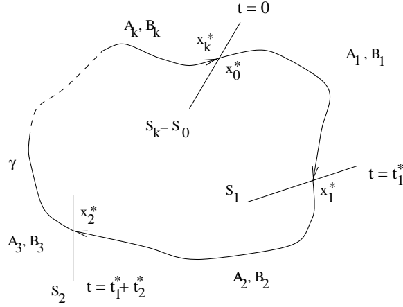
Figure 6-13: The limit cycle trajectory \gamma starts in state x_0^* , and travels through the first linear system ( \dot{\mathbf{x}} = A_1\mathbf{x} + B_1 ) until it crosses the first switching surface S_1 at time t_1^* . It continues into region 2, 3, etc. The limit cycle is complete after k switches, so that the state on the k th switch x_k^* is the same as the starting state i.e. x_k^* = x_0^* .
