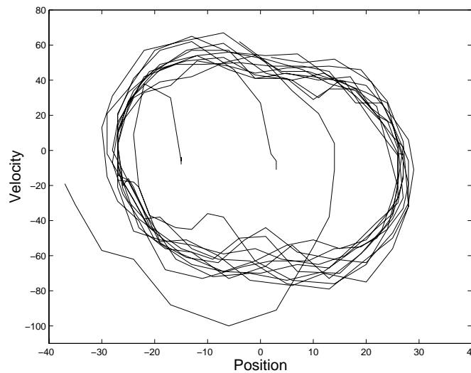
Figure 3-11: REAL Phase plot of robot motion. The plot shows velocity v . position for an oscillator driving a mass, recorded from one link of a robot arm. Shown are three traces overlaid starting from three different initial conditions. The three traces all converge to the limit cycle, indicative of the anecdotal observation that all initial conditions converge to the limit cycle.
