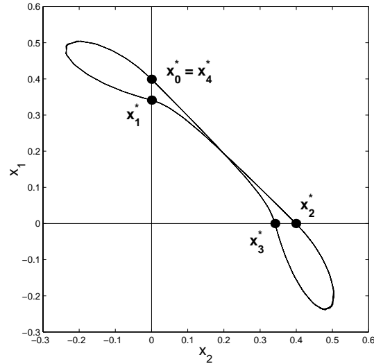
Figure 6-14: SIM Oscillator limit cycle plotted in the x_1 - x_2 plane. The points where the cycle crosses the switching surfaces x_1 = 0 (horizontal line), and x_2 = 0 (vertical line) are marked with \bullet 's. Using these points, and the times for the trajectory to go between them, the local stability of the limit cycle can be determined.
