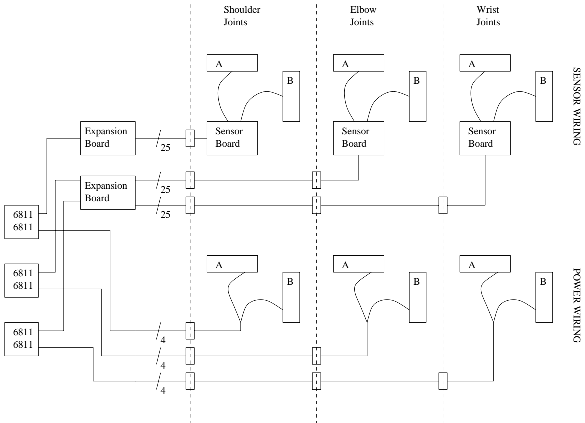
Figure A-24: Wiring diagram. The top half of the figure shows how the sensor cables from each set of joints are passed back along the arm to connect with expansion boards, and then to the motor controller boards (marked “6811”). Each sensor board handles the signals from two joints, and each expansion board handles two sensor boards. Each motor controller can drive two motors. The lower half of the figure shows the cables for the motor power. The dashed lines indicate where the arm can be easily split apart, with the boxes aligned with the lines indicating connectors. Thus the wrist joint can be removed by disconnecting only two connectors.
