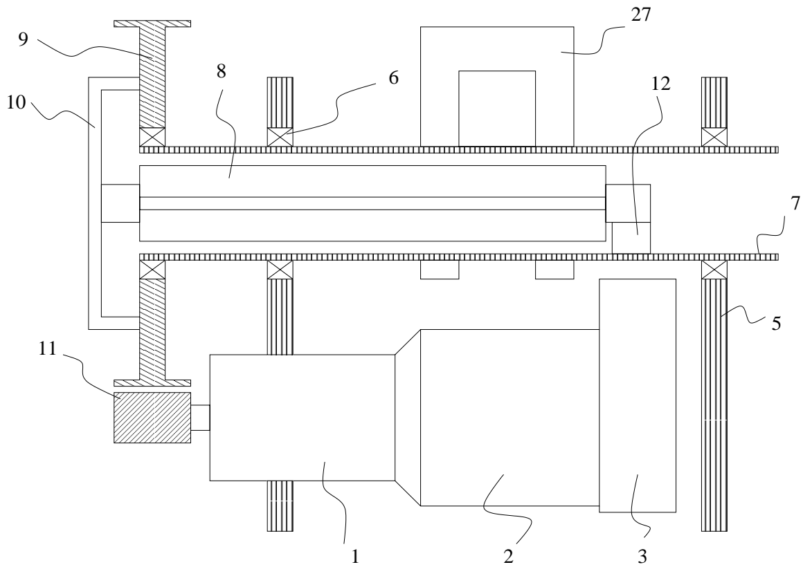
Figure A-12: Arm joint configuration II. This configuration is used for the shoulder-a, shoulder-b, elbow-b and wrist-b joints. The configuration is largely the same as in figure A-11, with the difference that the inputs and outputs to the actuator have been swapped. The motor and supports (1,2,3,5) is fixed, and the tube (7) moves. The output of the actuator can either be the right hand end of the tube (used in shoulder-a), or through the clamp (27) (used in the other joints). The advantage of using a clamp is that it can be easily removed.
