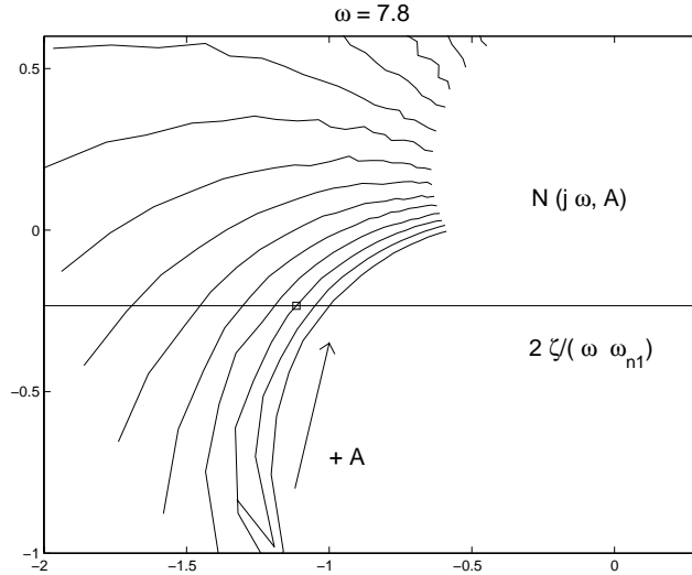
Figure D-2: SIM Local stability under torque feedback. The plot shows N(j\omega, A) and the line j2\zeta/(\omega\omega_n) = jc_1/(m_1k_1\omega) plotted on the complex plane, with a sample limit cycle marked with a \square . The limit cycle can be shown to be locally stable by examining changes in the system damping as the amplitude of oscillation A is varied. An increase in amplitude (in the direction of the arrow) results in N(j\omega, A) > 2\zeta/(\omega\omega_n) , which is equivalent to an increase in damping by (D.3), and so a reduction in the amplitude. A reduction in amplitude has the opposite effect, showing that the limit cycle is locally stable.
