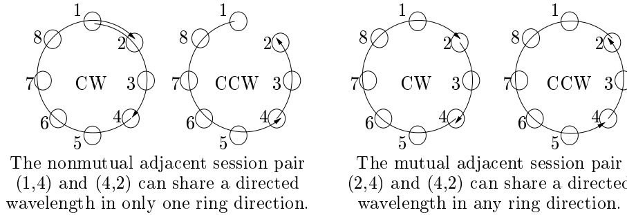
Figure 4-17: Supporting a mutual adjacent session pair on a directed wavelength.
