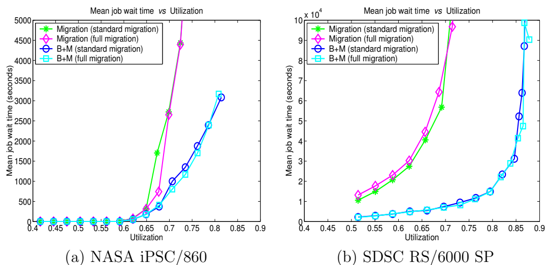
Figure 5-5: Mean job wait time vs utilization for the NASA and SDSC logs, comparing the standard migration policy to a full migration policy that always attempts to migrate.
